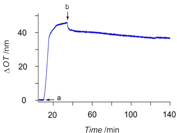
Figure 3: Change of optical thickness during measurement. a: Avidin addition. The adsorption of avidin on the walls of the porous film leads to an increase of the optical thickness. b: Rinsing with buffer.
