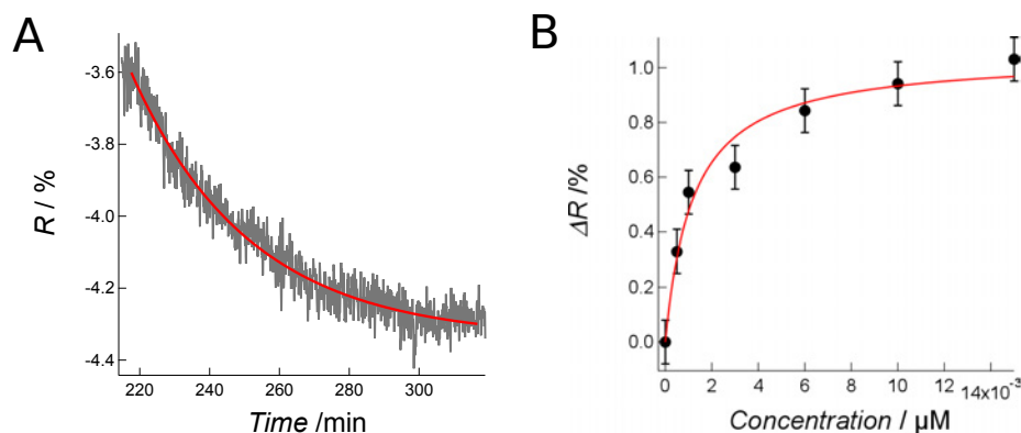
Figure 4: A: Change in reflectivity at 501 nm due to adsorption of Atto488-Biotin to an avidin-coated AAO membrane. The original data is shown in grey (smoothed) and the corresponding monoexponential fit in red. Atto488-Biotin was added at an overall concentration of 2 nM. B: Adsorption isotherm; Change in reflectivity as a function of biotin concentration (solid circles). The parameters of the Langmuir equation were fitted to the data (red curve), yielding a K_D value of (1.2 \pm 0.3) nM for the avidin-Atto488-Biotin interaction.
