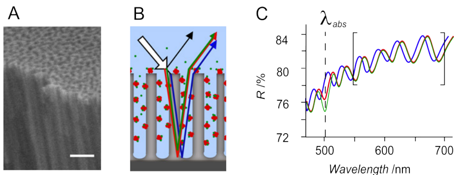
Figure 2: A: SEM image of AAO chip (scale bar: 500 nm). B: Scheme of sensing concept. Avidin (red dots) adsorbs on the pore walls of the AAO chip and causes a red shift of the interference spectrum shown in C (blue and red curve). When the dye-labelled biotin (green dots leading to the green beam) binds to the immobilised avidin, the reflectivity of the system is attenuated at the absorption maximum of the Atto dye shown as a drop in the spectrum in C (green curve).
