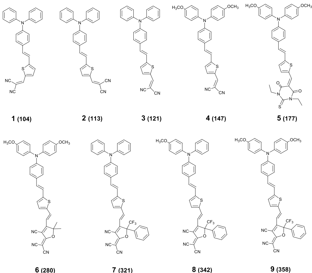
Scheme 1. The structures of three conformational isomers and several reported TAA based NLO chromophores. a Numbers in parentheses are \beta_{1907} value in units of 10^{-30} esu.
