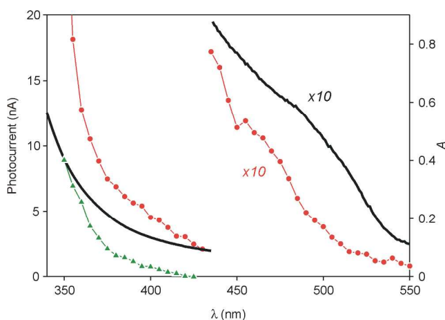
Fig. 6 Photocurrent spectrum (left scale) of the ITO electrode functionalized with ZnTe/ZnS (2 sh) nanocrystals (red circles) after subtraction of the photocurrent generated under the same conditions by the bare ITO (green triangles). The absorption spectrum of the QDs in \text{CHCl}_3 solution (black line, right scale) is also shown.
