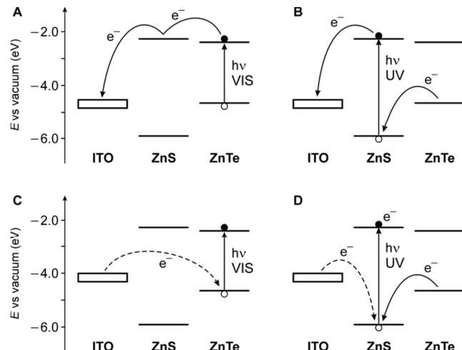
Fig. 7 Schematic energy-level diagram for the ITO photoelectrode coated with the ZnTe/ZnS QDs and representation of the electron-transfer processes that may occur under either visible light irradiation (A, anodic current; C, cathodic current) or UV irradiation (B, anodic current; D, cathodic current). The experimentally observed cases correspond to panels A and B. Dashed lines represent processes that are unlikely to occur. The electrode level is positioned considering an ITO work function of 4.4-4.7 eV, 59,60 taking into account the potential applied in the experiments.
