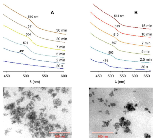
Fig. 3 Top: Absorption spectra ( \text{CHCl}_3 , room temperature) of the ZnTe nanocrystals at different growth times, prepared following (A) protocol 4 or (B) protocol 6 in Table 1 (the spectra are vertically offset for clarity). Bottom: TEM images of the nanocrystals obtained at saturation in case of (A) protocol 4 and (B) protocol 6. Scale bar, 100 nm.
