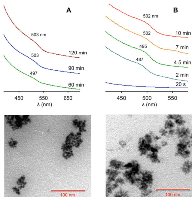
Fig. 2 Top: Absorption spectra ( \text{CHCl}_3 , room temperature) of the ZnTe nanocrystals at different growth times, prepared following (A) protocol 2 or (B) protocol 3 in Table 1. The spectra successive to the first one are vertically shifted for clarity. Bottom: TEM images of the nanocrystals obtained at saturation in case of (A) protocol 2 and (B) protocol 3. Scale bar, 100 nm.
