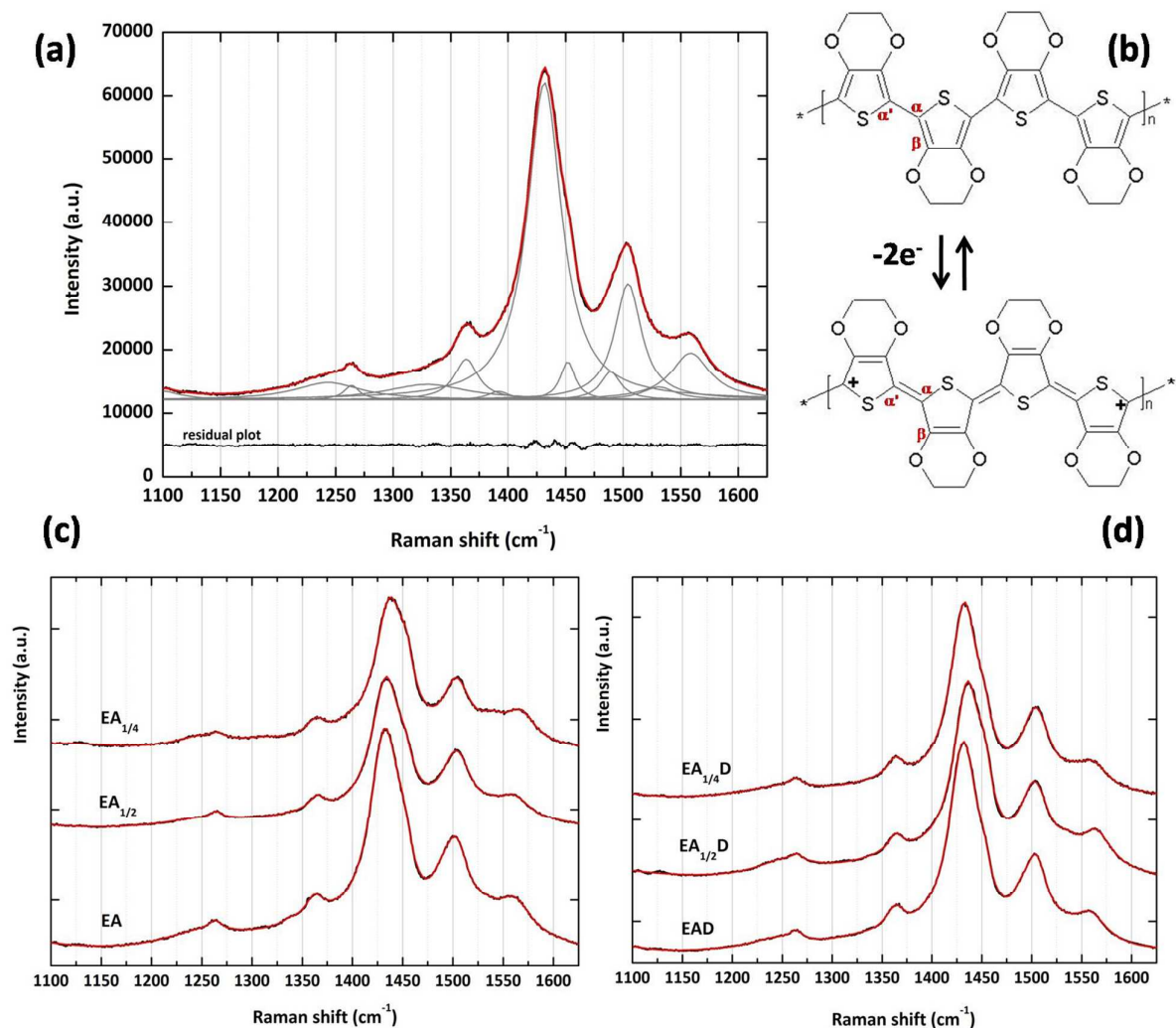
Figure 4. Raman spectra of the samples in the frequency range 1100-1600 cm -1 : (a) Raman spectrum of EAD sample with the bands resulting from the fitting; (b) sketch of the totally reduced and quinonoid totally oxidized form of PEDOT backbone; (c) spectra of EA, EA 1/2 and EA 1/4 samples; (d) spectra of EAD, EA 1/2 D and EA 1/4 D samples.
