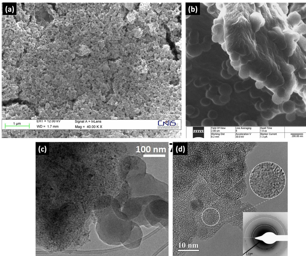
Figure 7. Pictures relating to the morphological study carried out on the PEDOT-ND sample EAD: (a) SEM image; (b) HIM image; (c) TEM image; (d) high resolution TEM image with the related ED pattern.
