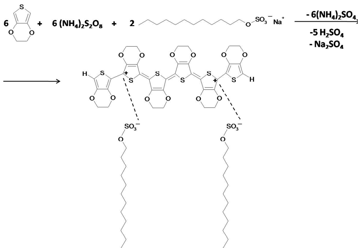
Figure 1. Reaction of EDOT oxidative polymerization to PEDOT - dodecyl sulfate initiated by APS . The reaction is depicted for the hexamer formation for simplification.
