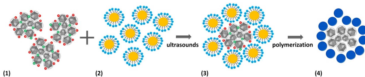
Figure 2. Depiction of the mechanism proposed for the soft-template synthesis route followed by the reagents during the preparation of the hybrid PEDOT-ND nanoparticles systems: (1) stable ND aggregates functionalized by positively charged (red dots) and radical (green dots) species; (2) EDOT monomers droplets stabilized in water by means of the anionic surfactant micelles; (3) self-assembly onto the ND aggregates surface of the EDOT-dodecyl sulfate surfactant systems; and (4) PEDOT nanospheres (blue circles) grown and assembled on nanodiamond grains.
