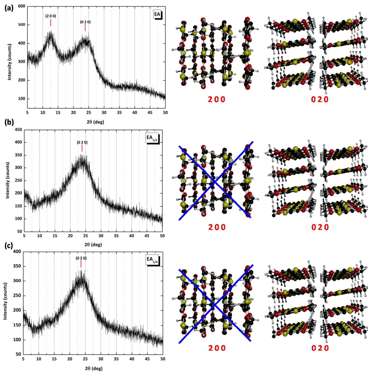
Figure 6. XRD spectra and depictions of parallel (200) and normal (020) periodicity of the polymer backbones of pure PEDOT samples: (a) EA; (b) EA 1/2 ; and (c) EA 1/4 .
