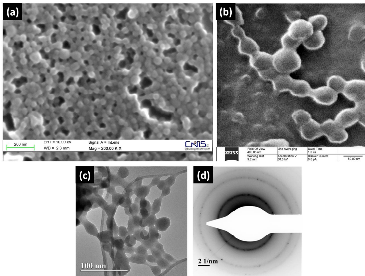
Figure 9. Pictures relating to the morphological study carried out on the PEDOT-ND sample EA 1/4 D: (a) SEM image; (b) HIM image; (c) TEM image; (d) ED pattern.
