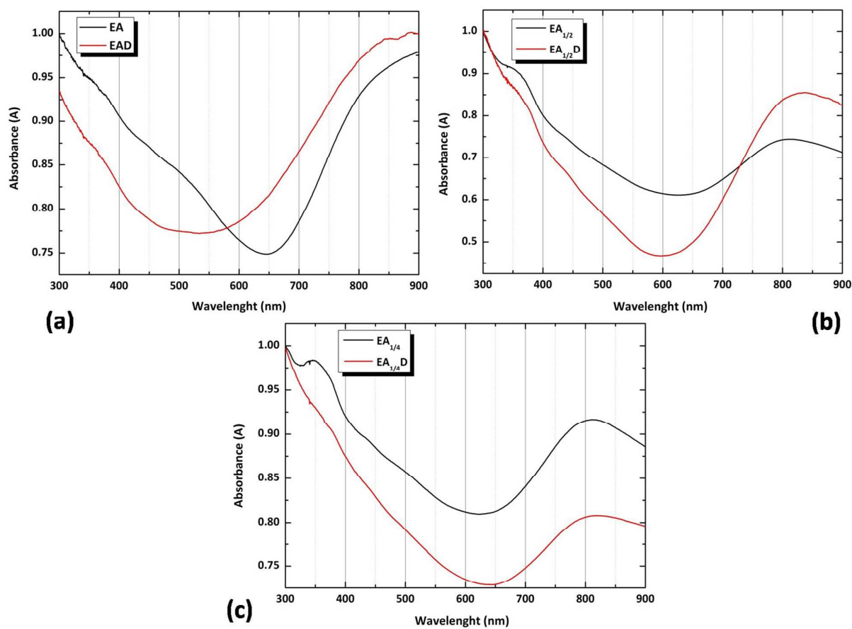
Figure 3. Absorption spectra of pure PEDOT and PEDOT-ND composites samples: (a) EA and EAD; (b) EA 1/2 and EA 1/2 D; (c) EA 1/4 and EA 1/4 D.
