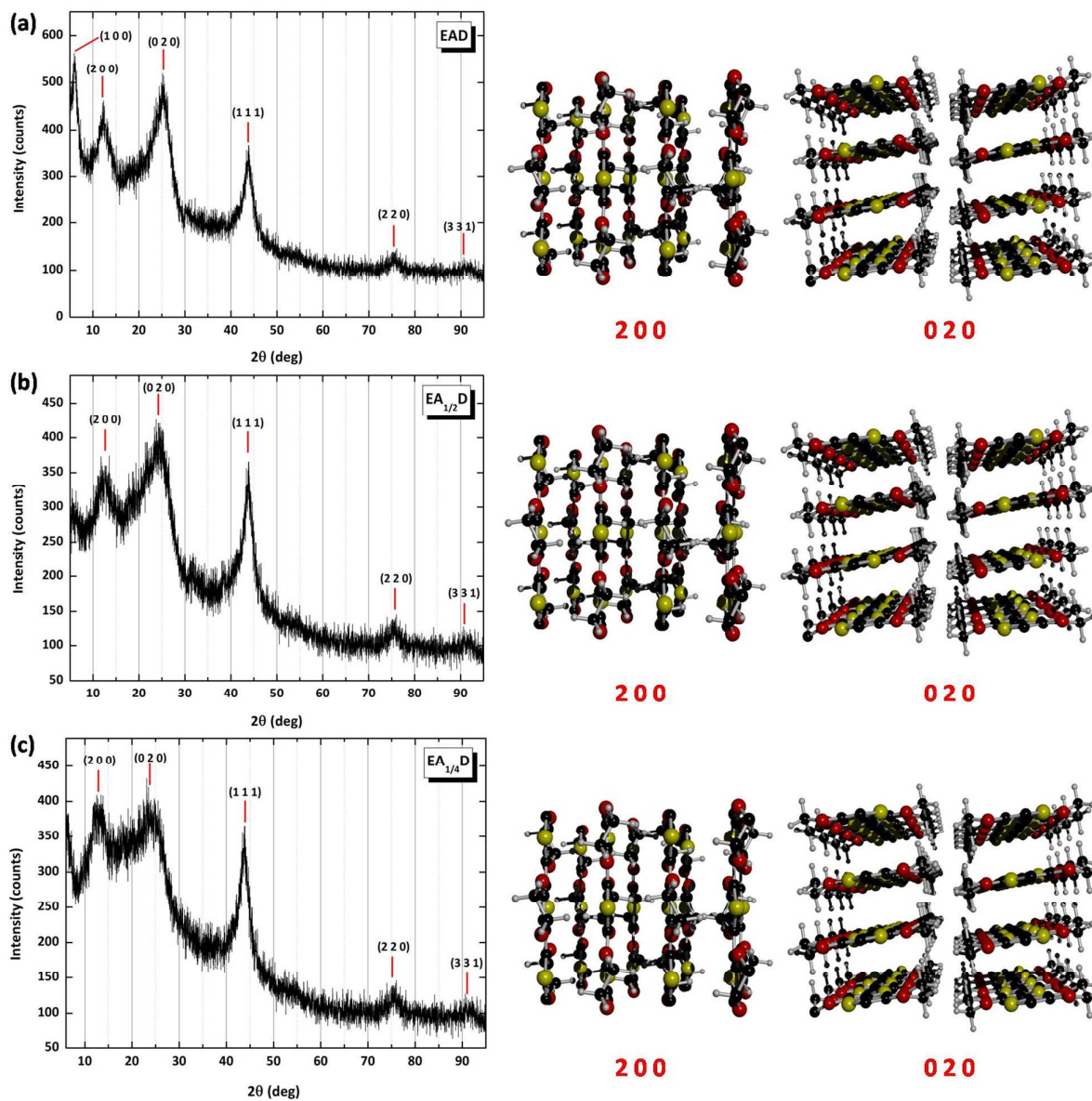
Figure 10. XRD spectra and depictions of parallel (200) and normal (020) periodicity of the polymer backbones of PEDOT-ND composites samples: (a) EAD; (b) EA_{1/2}D ; and (c) EA_{1/4}D .
