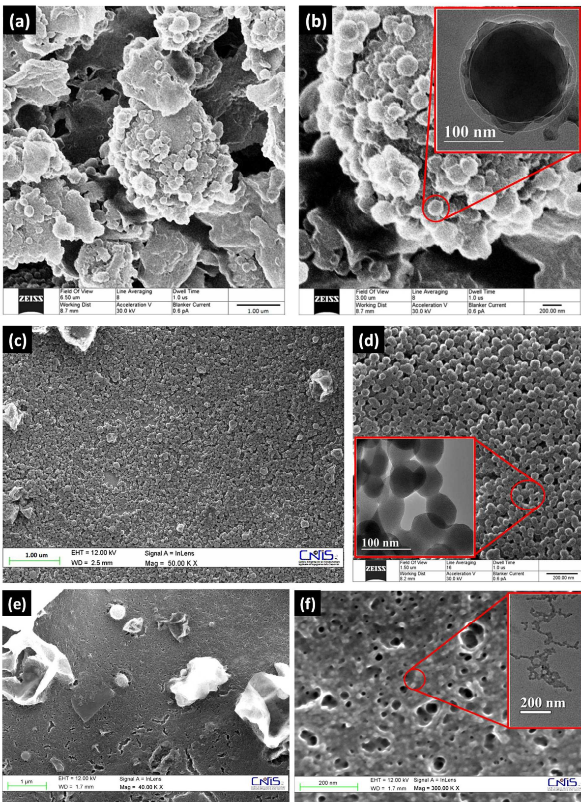
Figure 5. Pictures at different magnification of pure PEDOT samples: (a-b) HIM images of EA; (c) SEM and (d) HIM images of EA 1/2 and (e-f) SEM images of EA 1/4 . In Figure 4b, 4d and 4f insets showing TEM photos of the relating samples are shown.
