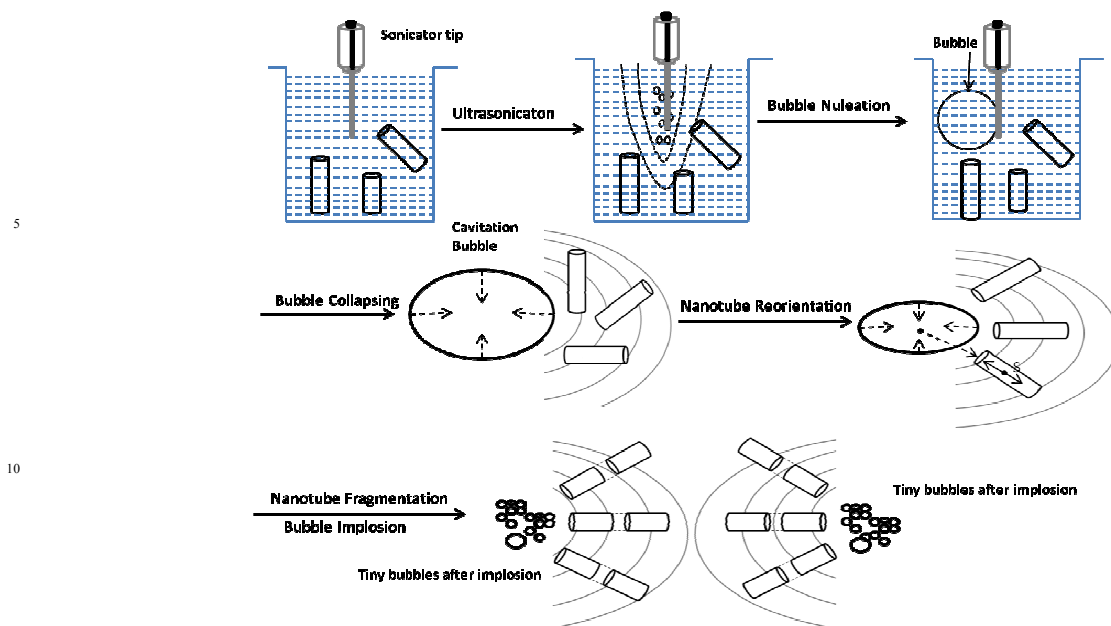
Fig. 3 Mechanism of sonication-induced scission for fragmentation of long polymer nanotubes
