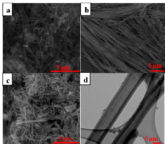
Fig. 2 SEM images of uniform PGMA-PNIPAAm long nanotubes with thermo-responsive gating system (a) before dialysis and (b) after dialysis; (c) PGMA-PNIPAAm fragmented short nanotubes with thermo-responsive gating system; and (d) TEM image of PGMA-PNIPAAm nanotubes
