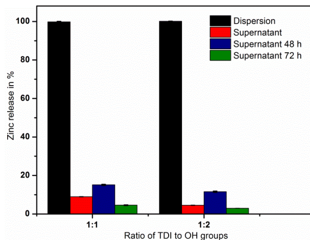
Figure 7: Relative zinc release from DexMa-PAAm nanogels with TDI shell is plotted with respect to the amount of TDI used for the shell formation (expressed as the ratio of TDI units to the amount of OH groups available from the dextran). Zn^{2+} content in the supernatant after redispersion (24h) and in the following two days is displayed relative to the redispersed samples ('Dispersion') which is set to 100% zinc content.
