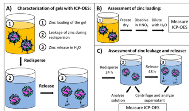
55 Figure 2: A) Scheme showing the three steps of sample characterization by ICP-OES. The steps include the investigation of zinc loading in the gel, of zinc leakage during the redispersion process and the release of zinc during consecutive water immersion. B) Sample collection for assessment 60 of zinc loading. C) Sample collection for assessment of zinc release, additional sampling after 72 h for nanogel-shell hybrids.
