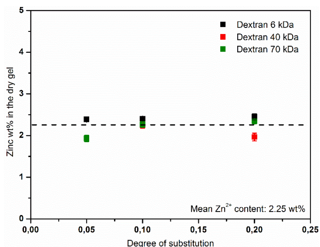
Figure 4: Weight percent of zinc with respect to the dry gel is plotted vs. the degree of substitution of dextran ( M_w : 6, 40 and 70 kDa). The average zinc loading is noted in the graph.
