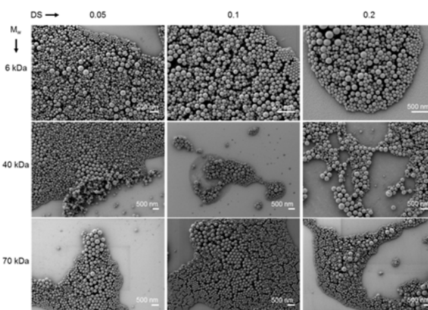
Figure 3: Scanning electron micrographs showing zinc loaded dextran-polyacrylamide nanogels dried from cyclohexane.
