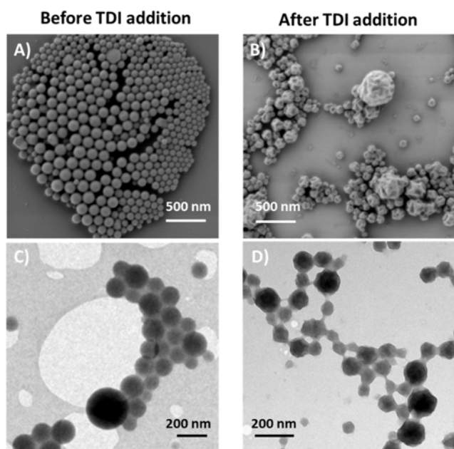
Figure 6: Micrographs of dried DexMa-PAAm nanogels A) and C) before TDI addition show spherical morphology, B) and D) Nanogels after shell formation with TDI, nanogels show crumpled morphology caused by water evaporation during drying process in SEM and TEM, respectively.
