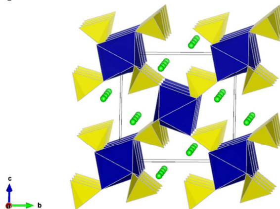
Fig. 1 \text{Li}_2M(\text{SO}_4)_2 ( M = \text{Fe}, \text{Mn}, \text{Co} ) crystal structure showing \text{MO}_6 octahedra (blue), \text{SO}_4 tetrahedra (yellow) and chains of Li ions (green) running parallel to the a -axis. [Experimental refinement data in Table S2].
