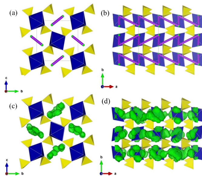
Fig. 4 Low energy Li diffusion paths within [100] channel of \text{Li}_2\text{M}(\text{SO}_4)_2 ( M = \text{Fe, Mn, Co} ). (a), (b) Static lattice calculations of low energy Li migration path combining L1 and L4 jumps. (c), (d) Li density plot as calculated using MD at 473 K. (a), (c) and (b), (d) are equivalent views along the a -axis and c -axis respectively.
