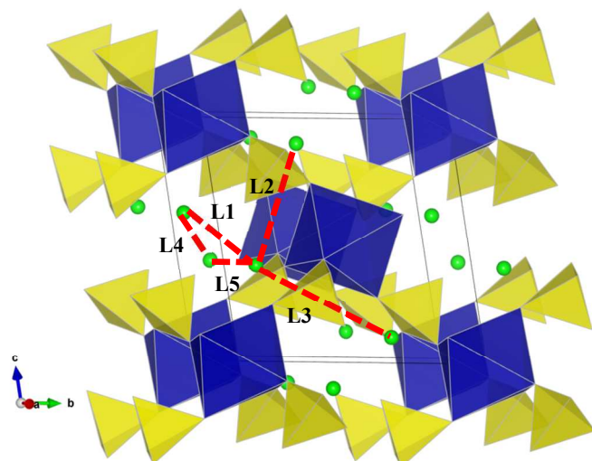
Fig. 3 Lithium ion migration paths in \text{Li}_2\text{M}(\text{SO}_4)_2 ( M = \text{Fe, Mn, Co} ) between adjacent Li sites (with initial Li positions found in table S2). Li-Li jumps considered are labelled L1-L5 (with Li-Li separations found in table S3).
