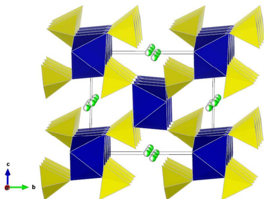
Fig. 2 Crystal structure of the delithiated phase LiFe(SO 4 ) 2 showing FeO 6 octahedra (blue), SO 4 tetrahedra (yellow) and Li ions (green) running parallel to the a -axis. [Experimental refinement data in Table S2].
