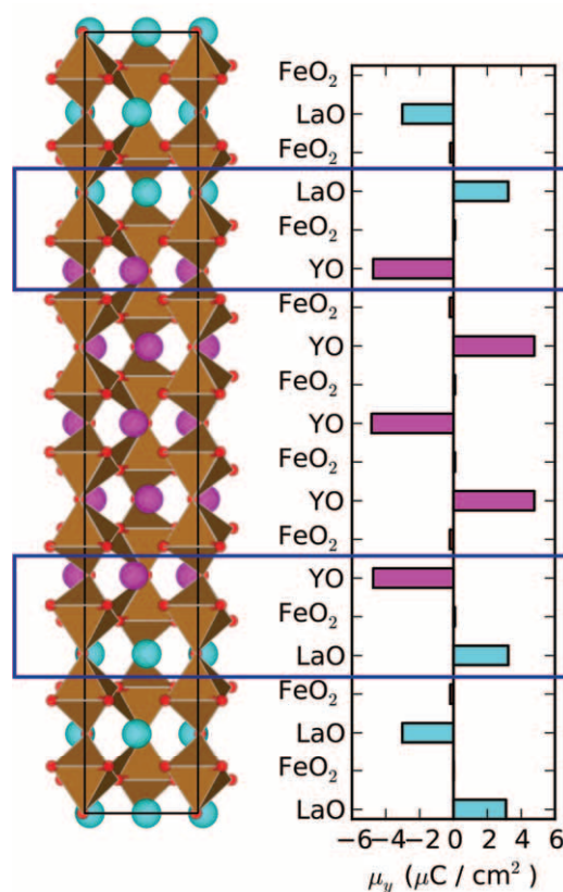
Figure 4: The calculated structure of the (\text{LaFeO}_3)_5(\text{YFeO}_3)_5 superlattice is shown alongside the contribution from each layer to the overall polarization. The box highlights the interface region where the local centre of symmetry is lost, leading to different contributions to the polarization from the AO layers above and below the interface and a finite overall polarization.
