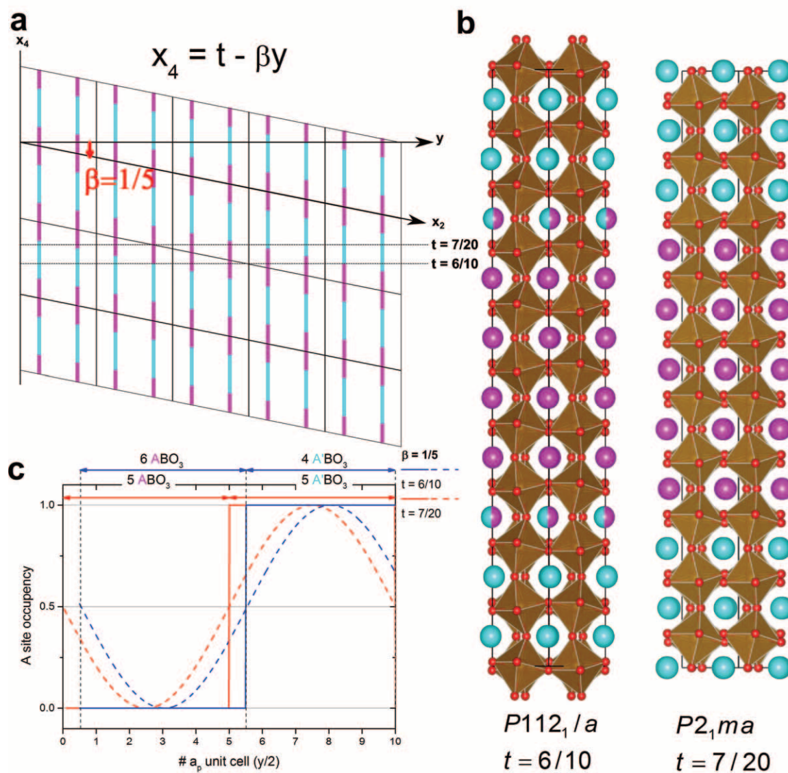
Figure 3: (a) Projection of the x_4, x_2 plane for \beta = 1/5 showing how the stacking sequence can be built up, here projections parallel to y correspond to structures in real space, where a cyan occupation domain is intersected a La is present on the A site
