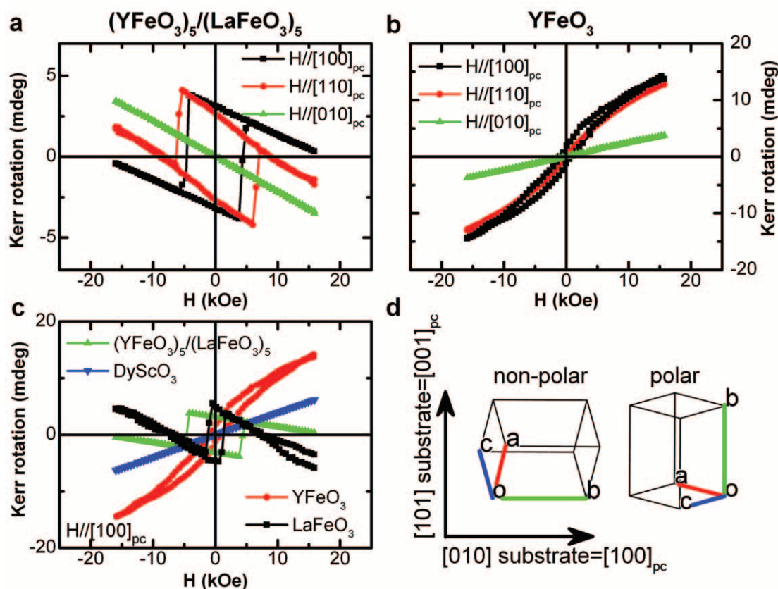
Figure 10: Magnetic hysteresis loops measured by longitudinal MOKE at room temperature on (a) the (YFeO 3 ) 5 /(LaFeO 3 ) 5 heterostructure and (b) on thin YFeO 3 film both grown on DyScO 3 (101) Pnma substrates, with magnetic field applied in different directions with respect to DyScO 3 [010] Pnma or [100] pc in orthorhombic and pseudo-cubic notations, respectively. (c) Comparison of MOKE hysteresis loops measured on blank substrate DyScO 3 (101) Pnma and on thin films of (YFeO 3 ) 5 /(LaFeO 3 ) 5 , YFeO 3 and LaFeO 3 grown on DyScO 3 (101) Pnma substrates, respectively. The magnetic field is applied along the DyScO 3 [010] Pnma axis. (d) Three-dimensional drawings of orthorhombic unit cells corresponding to the polar and non-polar phases in (YFeO 3 ) 5 /(LaFeO 3 ) 5 and their orientations with respect to orthorhombic (Pnma) or pseudo-cubic crystal axes of DyScO 3 (101) Pnma substrate.
