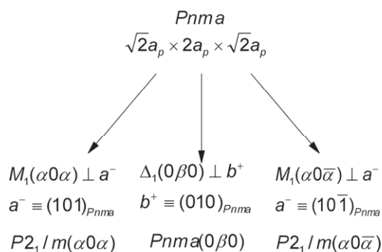
Figure 2: Layered A cation order perpendicular to the three Pnma axes can be treated as modulations at the M(\alpha 0\gamma) point, in the Brillouin zone for Pnma 47 , for the a^- axes (the general point corresponds to general planar orders perpendicular to the ac plane and the special cases (\alpha 0\alpha) , (\alpha 0-\alpha) to the two planes of interest) and \Delta(0\beta 0) point for the b^+ axis, subscripts
