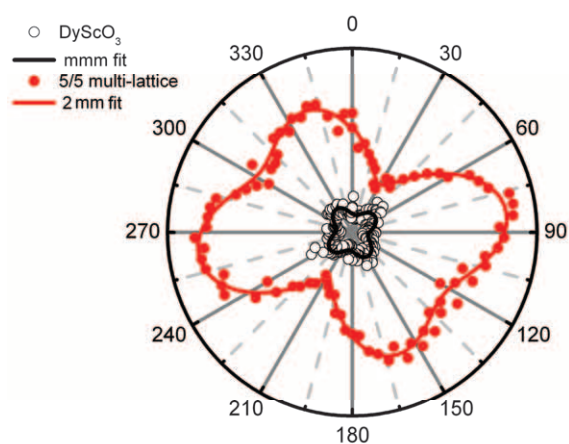
Figure 11: Optical second harmonic response vs. rotational angle of the polarizer. Filled (open) symbols and red (black) solid line represent data points and the corresponding fit for the film and blank \text{DyScO}_3 ( 101 ) _{Pnma} substrate with point symmetry group 2mm and mmm , respectively.
