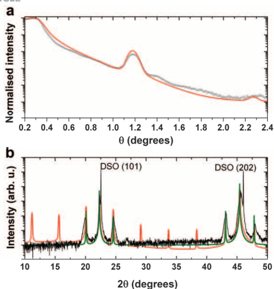
Figure 7: (a) x-ray reflectivity of the [(YFeO_3)_5(LaFeO_3)_5]_{40} heterostructure showing a Bragg reflection corresponding to an interatomic separation of 38.8 \text{ \AA} , the red line is a simulation of the heterostructure, the second feature around 2.3 degrees can be modeled using a surface roughness of 0.8 \text{ nm} . (b) Out of plane \theta - 2\theta XRD pattern of the heterostructure, the red line corresponds to a simulation of the structure using a crenel modulation (perfect interfaces) with the expected odd harmonic reflections whereas the green line corresponds to a simulation using a sinusoidal modulation of the A cation composition.
