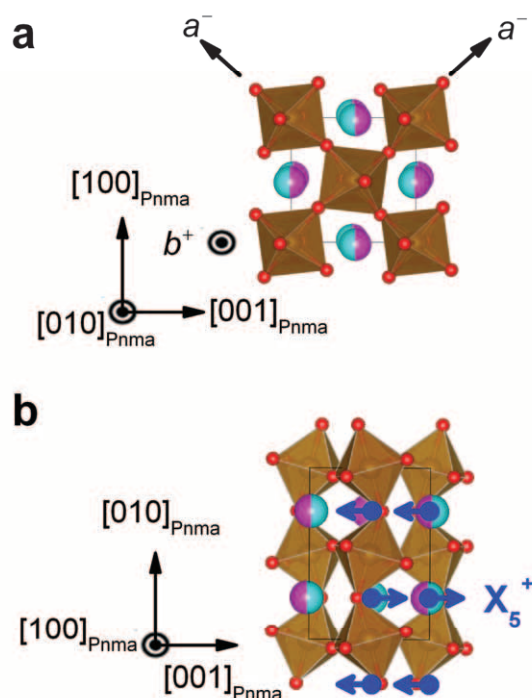
Figure 1: Projection of the Pnma GdFeO_3 structure (a) projected along the b axis showing the orientation of the tilt axes and (b), projected along a highlighting the X_5^+ A site antiferrodistortive displacement mode symmetry. Atoms are colored La (cyan), Y (magenta), Fe (brown) and O (red) throughout the manuscript.
