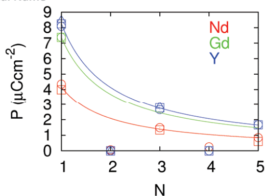
Figure 5: Polarization ( P ) versus the number of perovskite unit cells ( N ) in each block for \text{LaFeO}_3 - \text{LnFeO}_3 superlattices ( \text{Ln} = \text{Nd}, \text{Gd}, \text{Y} ). Data is plotted for three methods of calculating polarization: static charges (squares), Born effective charges (circles) and Berry phase (triangles). The function P1/N , where P1 is the average calculated polarization for the 1-1 superlattices, is plotted as a line for each family.
