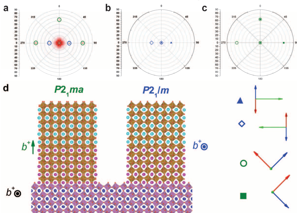
Figure 9: (a) Measured pole figure of the (111) reflection of the Pnma subcell showing two different domains corresponding to the non polar phase (peaks highlighted as blue circles) and the polar phase (peaks highlighted as green circles). (b) Simulated pole figure for the non-polar P2_1m phase considering two variants corresponding to different orientations of the 2a_p b^+ axis. (c) Simulated pole figure for the polar P2_1ma phase considering two variants corresponding to different orientations of the \sqrt{2}a_p a^- axes. (d) Representation of the two phases obtained from the A cation ordering stacked along the b^+ tilt (left structure) and perpendicular to the b^+ tilt (right structure) together with the substrate. The key on the bottom right explains the relationship between the Pnma perovskite subcell orientations in the two domains seen for each of the two phases (the 2a_p direction is shown in green, the two \sqrt{2}a_p directions in blue and red).
