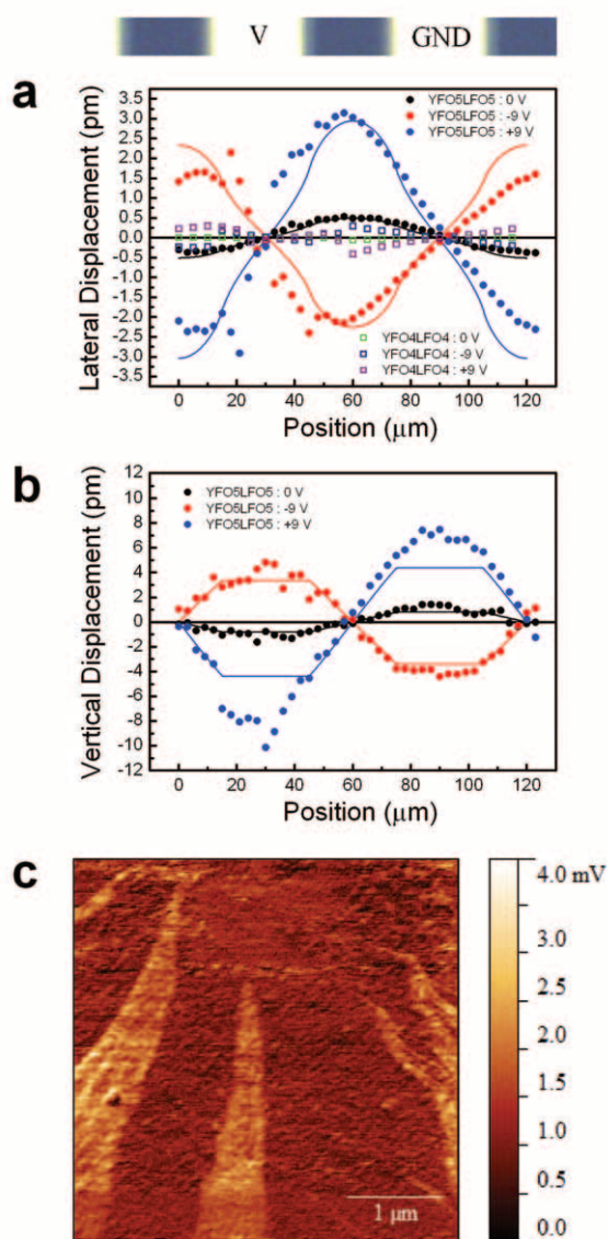
Figure 12: (a) Lateral and (b) vertical piezoresponse profile measurements (solid circles) and simulations (lines) for the (\text{LaFeO}_3)_5(\text{YFeO}_3)_5 and (\text{LaFeO}_3)_4(\text{YFeO}_3)_4 (square) thin films across a series of interdigitated electrodes shown in the top optical micrograph. The measurements and simulations are shown for three values of voltage offset, 0 V and \pm 9 V. (c) Scanning-mode PFM image of the (\text{LaFeO}_3)_5(\text{YFeO}_3)_5 film measured at a cantilever resonance using 1 V amplitude at 320 kHz. The vertical response amplitude is plotted, bright areas indicating polar domains whilst the dark areas are non-polar regions.
