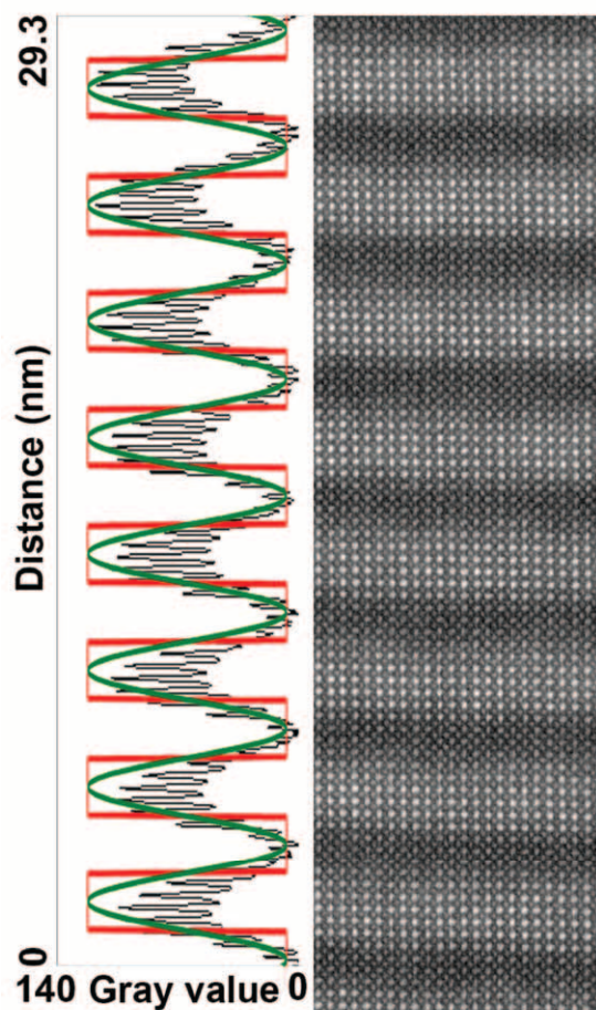
Figure 8: HAADF-STEM image (right) and intensity profile (left) over the same region of the [(YFeO_3)_5(LaFeO_3)_5]_{40} heterostructure. The red and green functions superimposed on the intensity profile correspond to the crenel and sine-wave modulation models used to produce the XRD simulations. The gradual overall decrease in peak height from top to bottom is due to varying cross-section thickness.
