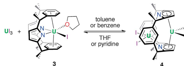
Scheme 5 Equilibrium behaviour of 3 and 4 in solution.
