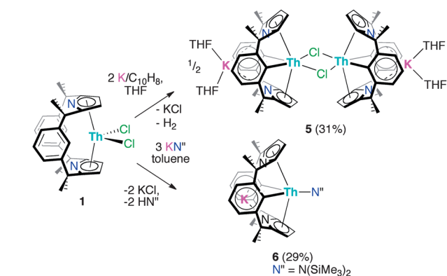
Scheme 6 Syntheses of [K(THF) 2 Th( \mu -Cl)(L -2H ) 2 , 5 and K[Th(N'')(L -2H )], 6 .
