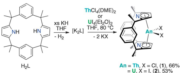
Scheme 2 Syntheses of [ThCl 2 (L)], 1 and [U 2 (L)], 2 .
