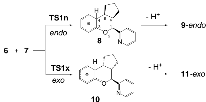
Scheme 5
