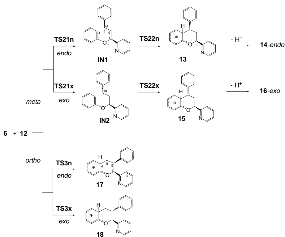
Scheme 6
