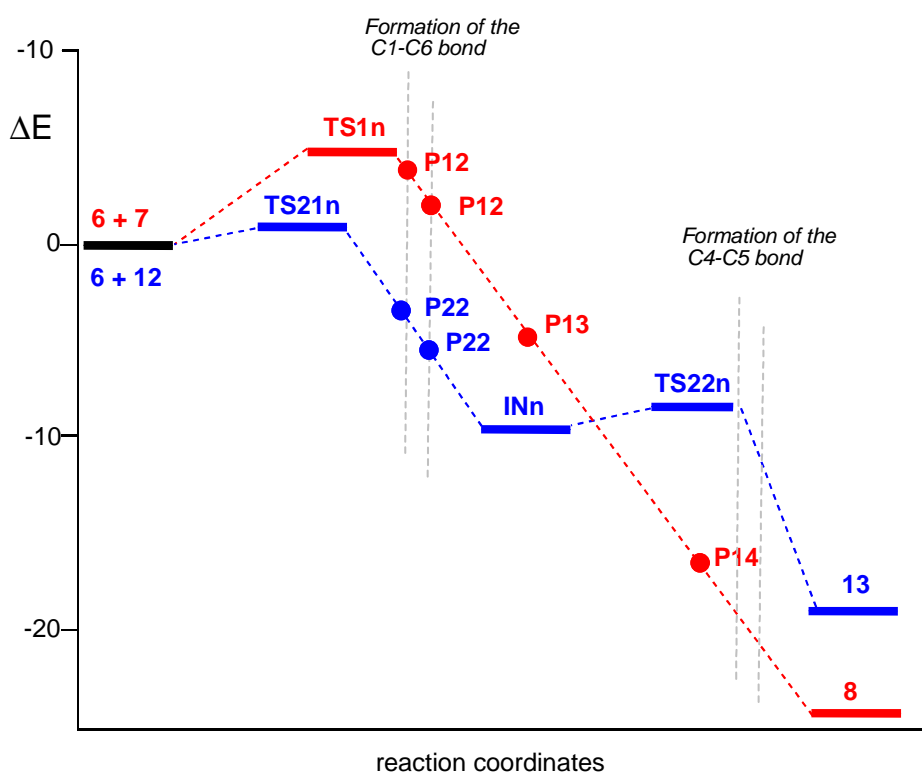
Figure 4. Schematic representation of the energy profiles along the one-step (in red) and two-step (in blue) mechanisms of the I-DA reactions of oxonium cation 6 with cyclopentene 7 and styrene 12 . The non-stationary selected points of the IRC used in the ELF analysis are represented by points.
