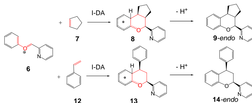
Scheme 4
