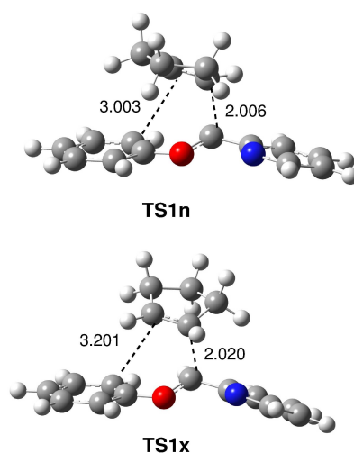
Figure 1. Transition state structures involved in the I-DA reactions between oxonium cation 6 and cyclopentene 7 . Lengths are given in Angstroms.
