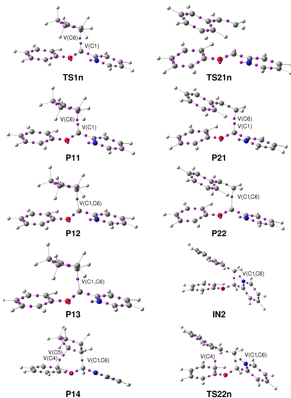
Figure 3. Most relevant ELF attractors at some selected points of the IRCs of the one-step and two-step I-DA reactions of oxonium cation 6 with cyclopentene 7 and styrene 12 .
