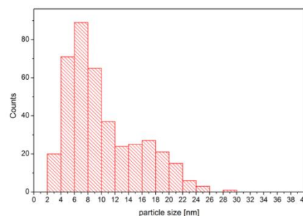
Figure 3: Ag-NPs synthesised in n -Bu 4 POAc (scale bar 100 nm). The major maximum is at 6.7 nm and the minor maximum at 15.6 nm.
