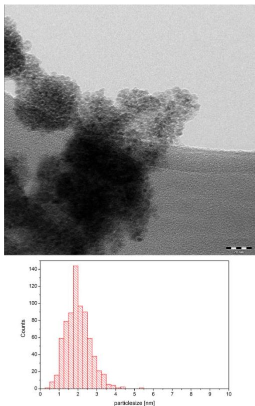
Figure 6: TEM-picture of nickel(II)oxide nanoparticles (2.0 nm) synthesised in bmmim NTf 2 (scale bar 20 nm) with size distribution.
