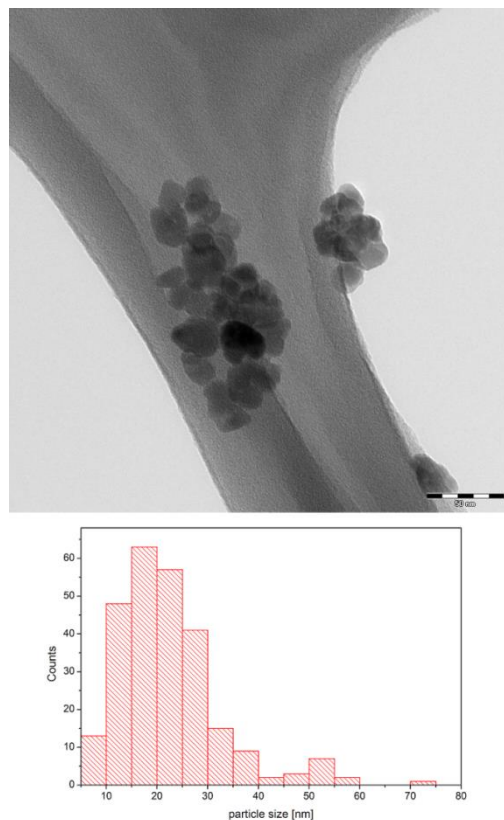
Figure 7: TEM-picture of zinc oxide nanoparticles (22.2 nm) synthesised in n -Bu 4 POAc (scale bar 50 nm) with size distribution.
