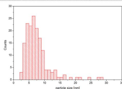
Figure 5: TEM-picture of nickel(II)oxide nanoparticles (5.8 nm) synthesised in n -Bu 4 POAc (scale bar 20 nm) with size distribution.
