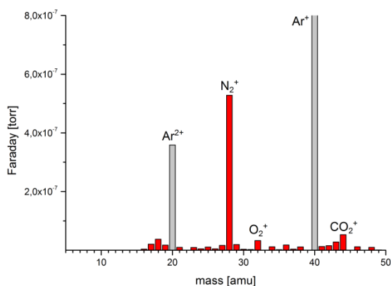
Figure 9: Gas-phase mass spectrogram of volatile compounds of the reductive decomposition of Copper(II)acetate in bmmim NTf 2 . Argon (m/z = 40, m/z = 20) is used as carrier gas.
