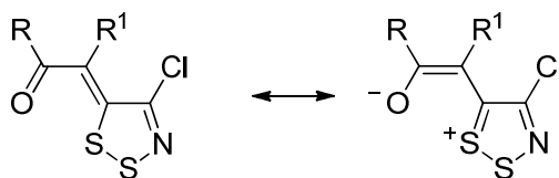
Scheme 5. Resonance structures of dithiazolylidenes supporting \beta -carbonyl groups.
