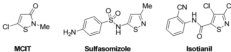
Figure 1. Commercially important isothiazoles.
