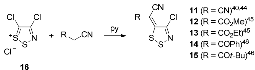
Scheme 2. Route to known (dithiazolylidene)acetonitriles 11-15 .
