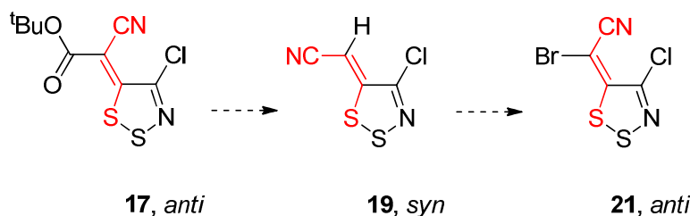
Scheme 8. Stereochemical changes on transforming dithiazole 17 into 21 .
