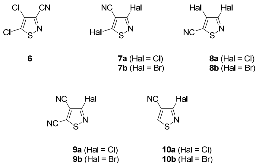
Figure 3. Chemical structures of common haloisothiazolecarbonitriles.
