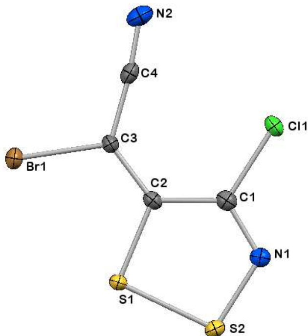
Figure 5. Ellipsoid (probability level of 50%) representation of the crystal structure of ( E )-2-bromo-2-(4-chloro-5 H -1,2,3-dithiazol-5-ylidene)acetonitrile ( 21 ) with crystallographic atom labelling.
