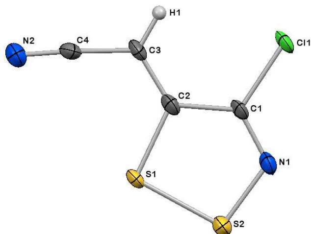
Figure 4. Ellipsoid (probability level of 50%) representation of the crystal structure of (Z)-2-(4-chloro-5H-1,2,3-dithiazol-5-ylidene)acetonitrile ( 19 ) with crystallographic atom labelling.
