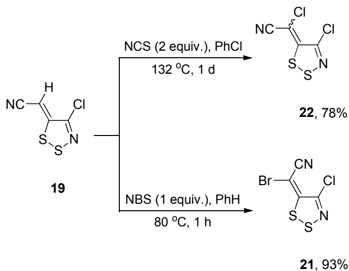
Scheme 7. Preparation of 2-bromo and 2-chloro(dithiazolylidene)acetonitriles 21 and 22 .
