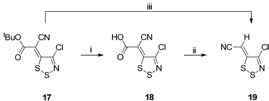
Scheme 3. Reagents and conditions: i) c. H 2 SO 4 , ca. 20 °C, 5 min, 93%; ii) TsOH (10 mol%), PhCl, 132 °C, 4 h, 87%; iii) TsOH (10 mol%), PhCl, 132 °C, 4 h, 94%.
