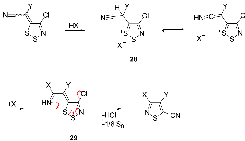
Scheme 9. General mechanism for the ring transformation of dithiazoles to give isothiazole.
