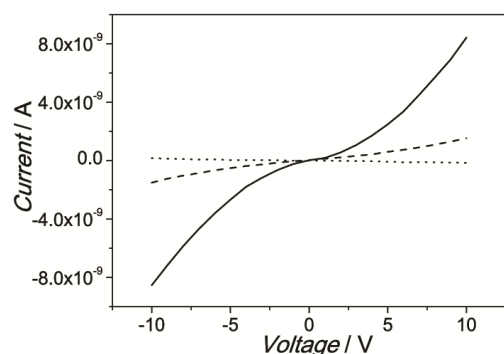
Fig. 7 I-V curves measured for nanobelts and nanoleaves of \text{Zn}[\text{Pc}(\text{OPh})_8] formed from n -hexane (solid line) and methanol (dash line) and the cast film (dot line) deposited on ITO IDEs/glass substrates.
