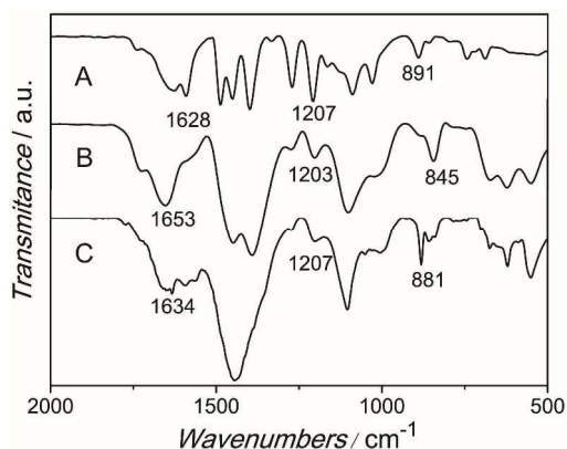
Fig. 2 IR spectra of (A) the bulk Zn[Pc(OPh) 8 ], its self-assembled nanostructures formed (B) in n -hexane and (C) in methanol, in the region of 500-2000 cm -1 with 2 cm -1 resolution.
