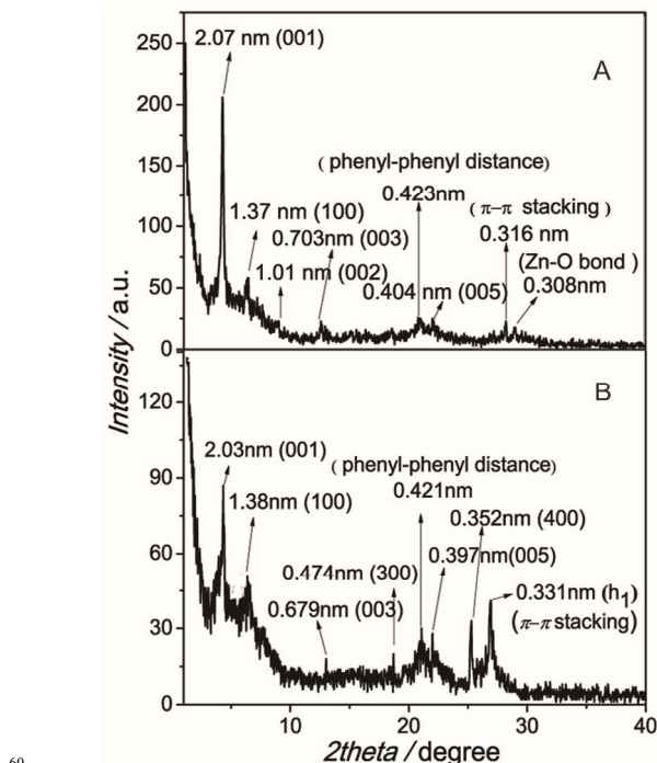
Fig. 3 X-ray diffraction patterns of the self-assembled nanostructures of Zn[Pc(OPh) 8 ] formed (A) in n -hexane and (B) in methanol.
