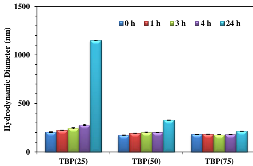
Figure 8. Polyplex stability ( \pm ratio = 4) over 24 h in salt solution, Dulbecco's modified Eagle's media (DMEM).
