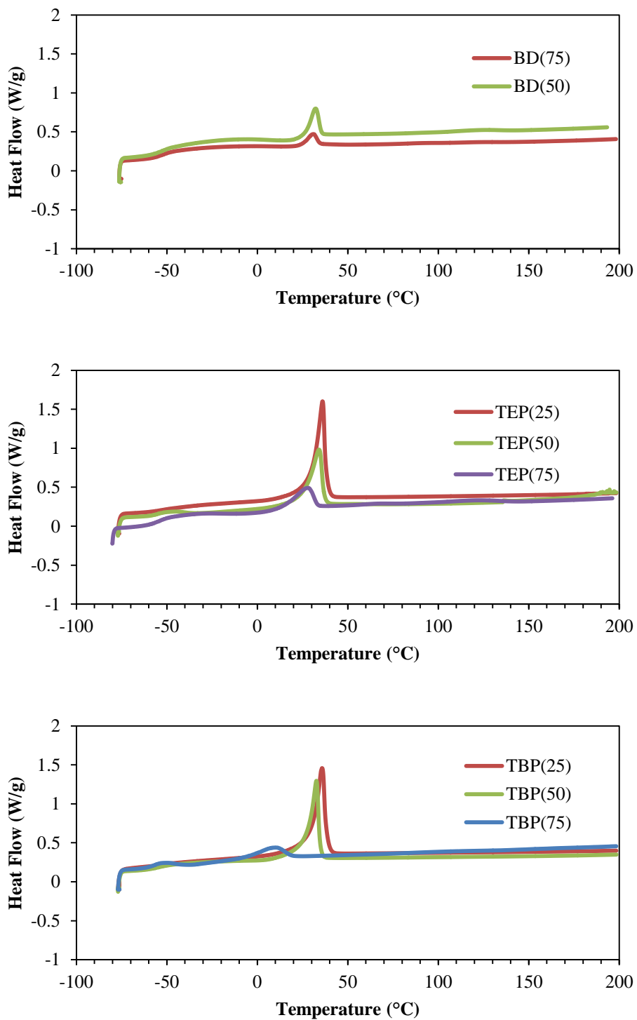
Figure S 10. Second heat DSC traces of polyurethane compositions (Ramp 10 °C/min, N 2 ).
