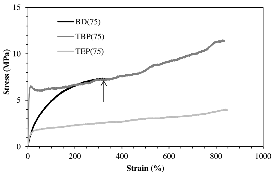
Figure 5. Representative tensile stress-strain curves of noncharged and phosphonium polyurethanes. Arrow designates the stress and strain at break for BD(75).
