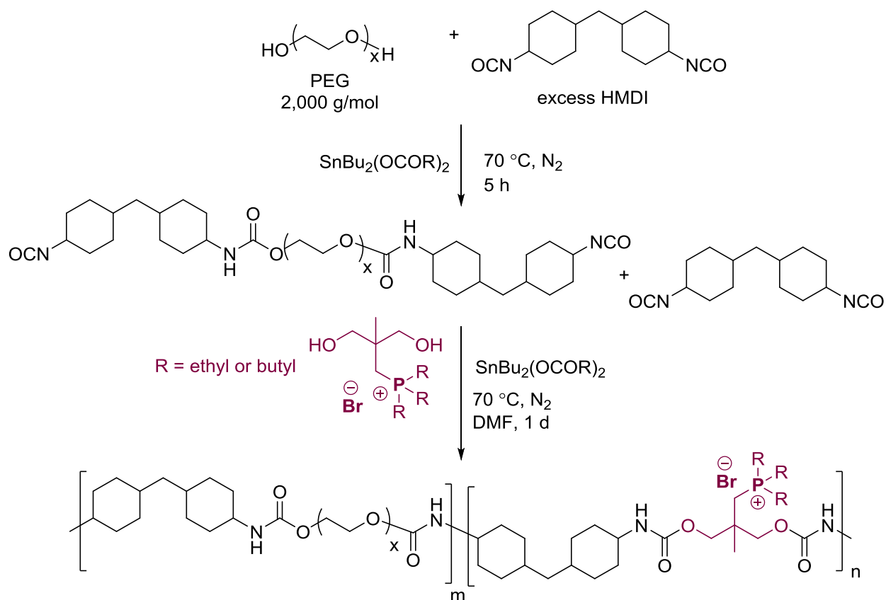
Scheme 2. Synthesis of trialkylphosphonium polyurethanes.
