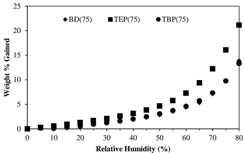
Figure 6. Sorption isotherm of noncharged and phosphonium polyurethanes (75 mol% HS) at 25 °C.
