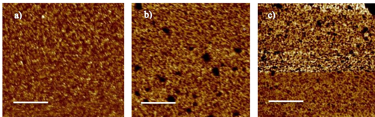
Figure 4. Atomic force microscopy phase images: a) BD(75), b) TEP(75), and c) TBP(75) polyurethanes. The scale bars represent 200 nm.
