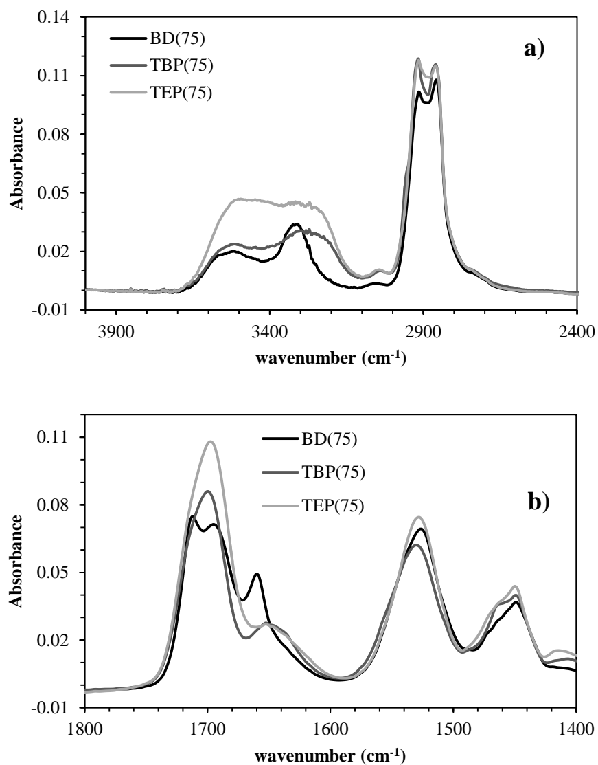
Figure 3. FTIR spectra of noncharged and phosphonium polyurethanes: a) N-H stretch between 3000 – 3500 cm -1 and b) carbonyl stretch between 1600 – 1750 cm -1 .
