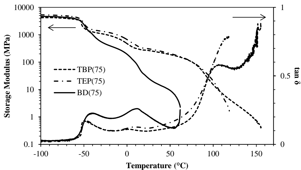
Figure 2. Dynamic mechanical analysis of noncharged and phosphonium PU (75 mol% HS). Left and right arrows indicate curves for the storage modulus and \tan \delta , respectively.
