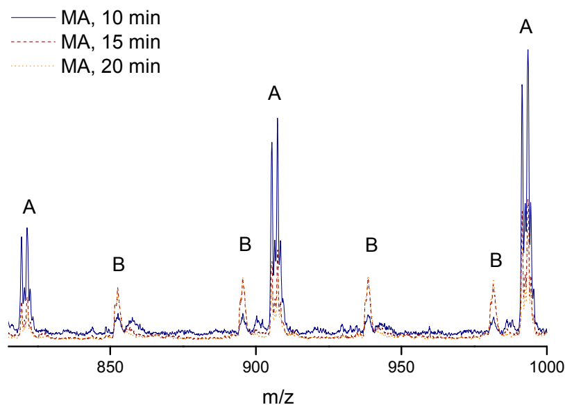
Figure 5: Zoom into ESI-MS spectra of poly(methyl acrylate) obtained by UV-copper-mediated polymerization in flow reactors. The 15 and 20 min sample show higher relative intensities for double charged species due to their higher M_n which lies above the scan range of 2000 \text{ g} \cdot \text{mol}^{-1} .
