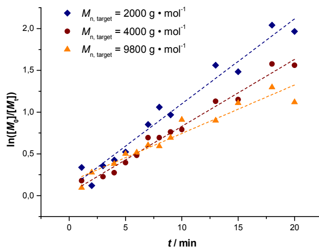
Figure 2: First order kinetic plots of the MA polymerizations in a milli-flow reactor with targeted M_n = 2000 (◆), 4000 (●) and 9800 (▲) \text{g} \cdot \text{mol}^{-1} .
