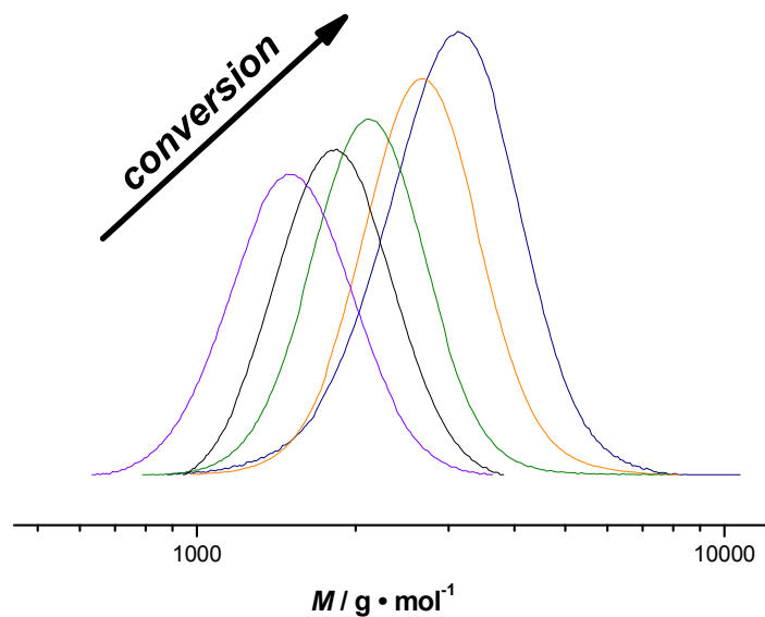
Figure 3: Molecular weight distributions of pMA with increasing residence time in the microflow reactor synthesized via UV-initiated copper-mediated polymerization and with targeted M_n of 4000 \text{ g} \cdot \text{mol}^{-1} . All distributions are scaled to monomer conversion.
