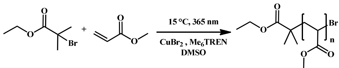
Scheme 1: UV-induced copper-mediated polymerization of methyl acrylate (MA) in DMSO using CuBr 2 and Me 6 TREN as catalyst/ligand pair.
