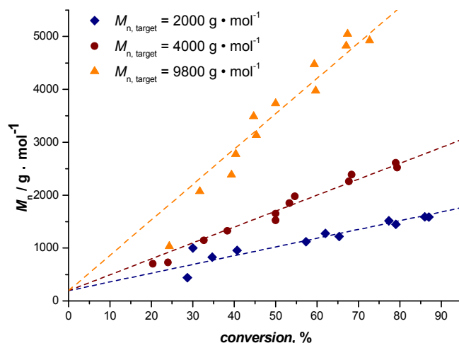
Figure 1: Development of the M_n of a UV initiated copper-mediated polymerization of MA, with targeted M_n = 2000 ( \blacklozenge ), 4000 ( \bullet ) and 9800 ( \blacktriangle ) \text{g}\cdot\text{mol}^{-1} , in a tubular milli-flow reactor. The dotted lines are best fits of the data whereby the axis intercept was set to the molar mass of the initiator.
