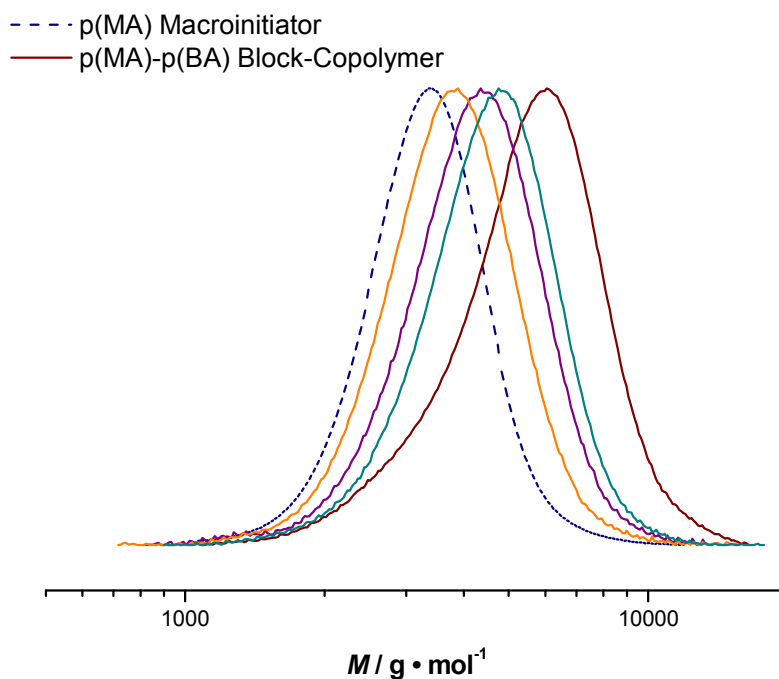
Figure 6: Evolution of molecular weight distributions for the p(MA)- b -p(BA) block copolymers (solid line) obtained in flow microreactor and the distribution of the p(MA) macroinitiator (dashed line).
