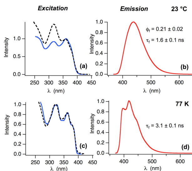
Fig. 2 Fluorescence excitation (blue; a, c) and emission (red; b, d) spectra of Me-sFCC in EtOH at room temperature (a, b) and EtOH glass at 77 K (c, d). \lambda_{\text{ex}} = 360 nm. The absorption spectra of 1 at room temperature (a) and at 77 K (c) are shown as black dashed lines.
