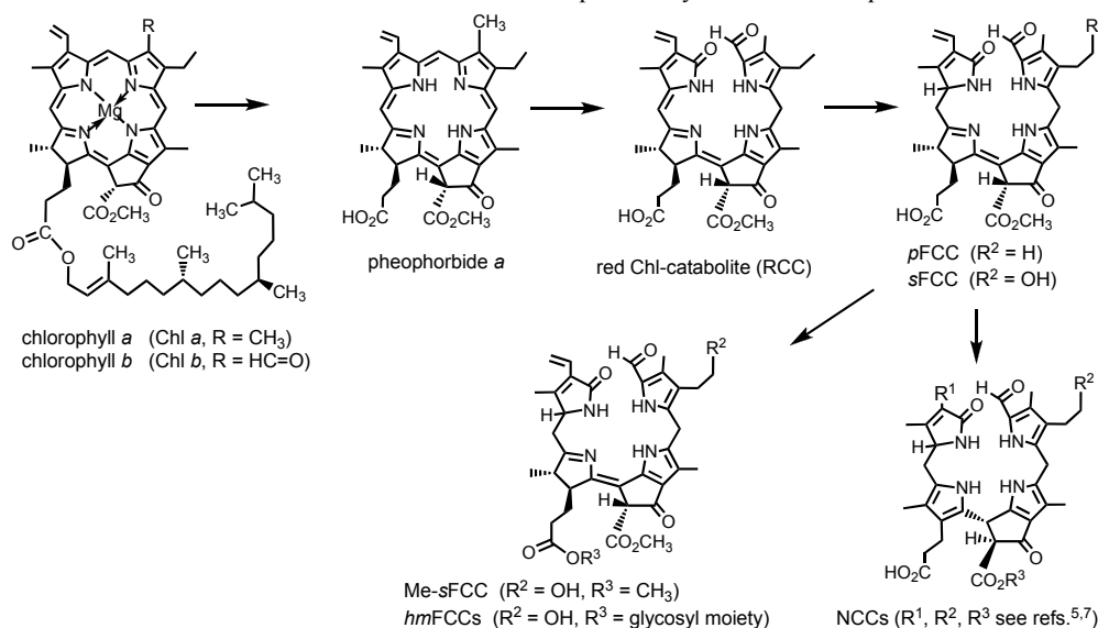
Scheme 1. Outline of chlorophyll breakdown in higher plants with structural formulas and names of key compounds (see refs. 5,7,18 for more details).
