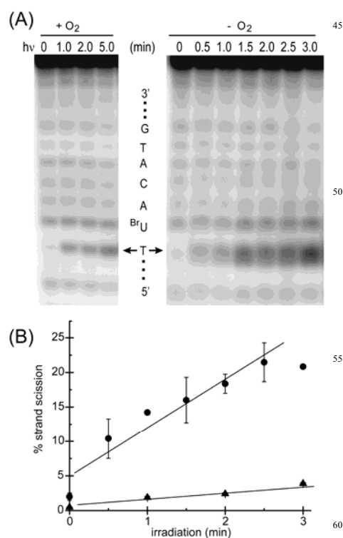
Fig. 1 EET induced between by a diffusible donor and a BrdU acceptor within duplex DNA containing an abasic site. (A) DNA ( ODN1/ODN2 ) and diamino-naphthalene ( 1 , 1 mM) were irradiated for the indicated time ( \lambda > 335 nm) under aerobic and anaerobic conditions alternatively and then treated with hot piperidine to induce strand scission at the residue (T) on the 5'-side of BrdU after its capture of an electron. Products were separated by gel electrophoresis and detected by phosphorimager. (B) The fraction of the 5' scission product formed under aerobic (▲) and anaerobic (●) conditions was quantified relative to total DNA. The error represents the spread of duplicate measurements, and linear best fits were used to estimate the initial rate of the collective processes controlling electron injection, migration and capture. 35 The background level of strand scission induced by piperidine treatment is indicated by the value measured at t_0 . This was not subtracted from the yield of scission as evident by the non-zero interceptions.
