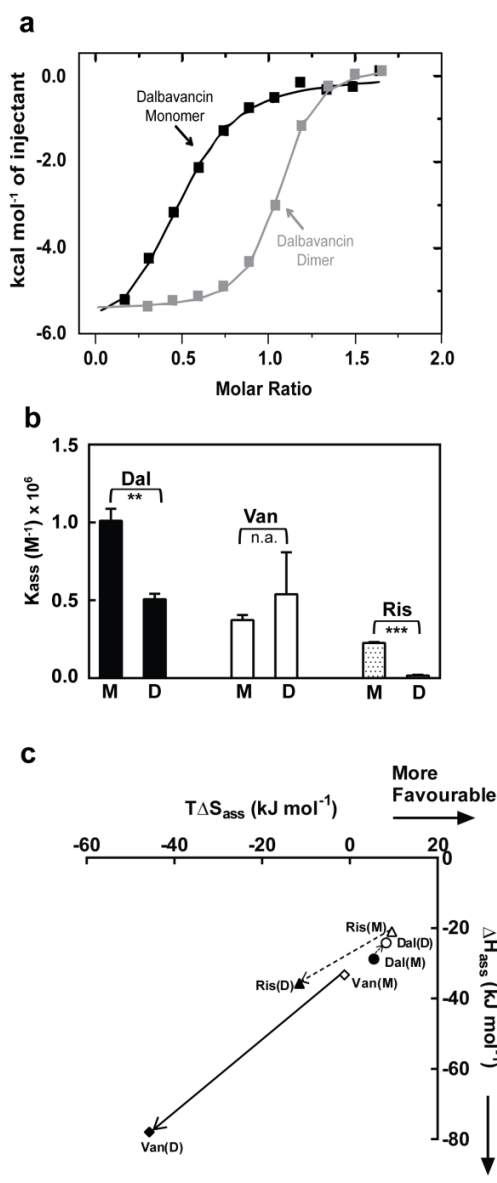
Fig. 3 ITC binding data of dalbavancin (Dal), vancomycin (Van) and ristocetin A (Ris) at 25°C in 0.1 M NaOAc (pH 5.0) showing anti-cooperativity of ligand binding to dimer for dalbavancin and ristocetin A. (a) Integrated titration curves upon complexation of Ac 2 -Kaa with dalbavancin monomer (black) and dimer (grey), with theoretical fit to a single site binding mode. 40 (b) The binding constant ( K_{ass} ) of antibiotic monomers (M) and dimers (D). Statistical comparison of K_{ass} values was performed by the two-tailed Student's t -test (**, p < 0.01 ; ***, p < 0.001 ). (c) Enthalpy-entropy plots showing thermodynamics of ligand binding for three antibiotics (Dal: ○; Van: ◇; Ris: △). Means ± SD for n=3 .
