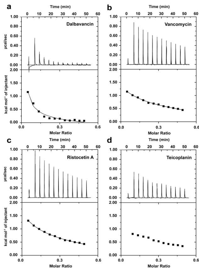
Fig. 2 Typical ITC dilution data of dalbavancin (a), vancomycin (b), ristocetin A (c) and teicoplanin (d) in the absence of ligand at 25°C in 0.1 M NaOAc buffer, pH 5.0. Upper profile: endothermic responses for sequential injections; lower profile: integrated dilution heat effects with theoretical fit to a dimer-monomer dissociation model. 20
