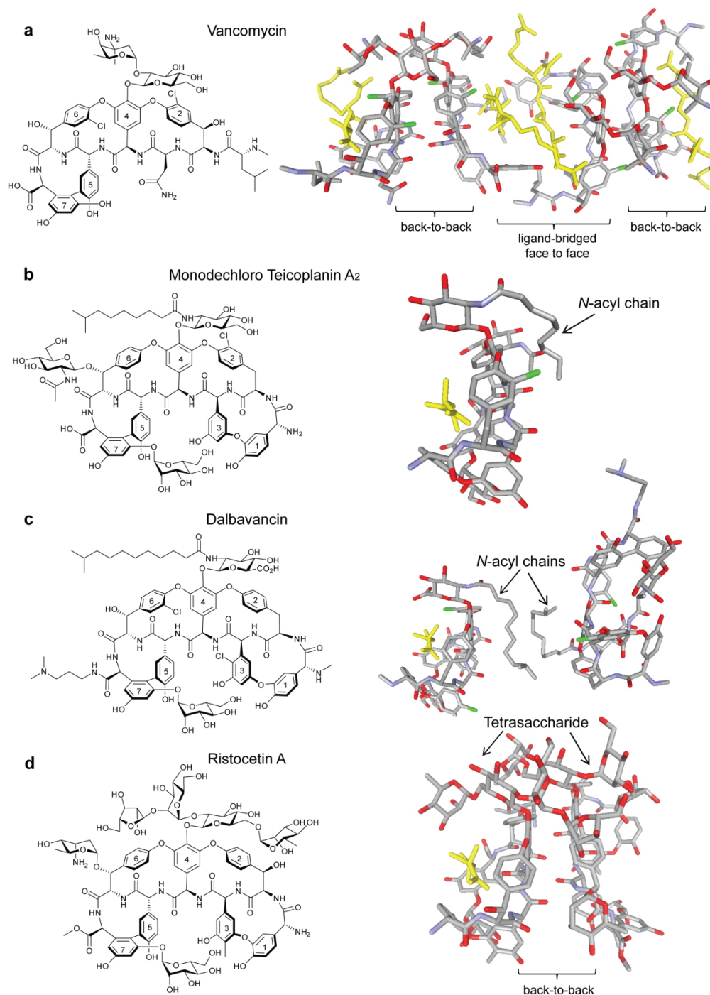
Fig. 1 Glycopeptide antibiotics vancomycin (a), 19 monodechloro teicoplanin A 2 (b), 33 dalbavancin (c) 19 and ristocetin A (d) 19 with published crystal structures 19,33 highlighted to show bound ligand Lys-D-Ala-D-Ala (yellow) in the Lipid II binding site. Carrier proteins used for crystallisation omitted from b, c and d.
