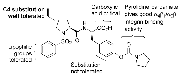
Figure 2. Structure activity relationship for N -phenylsulfonyl proline-based \alpha_9\beta_1 integrin antagonists.
