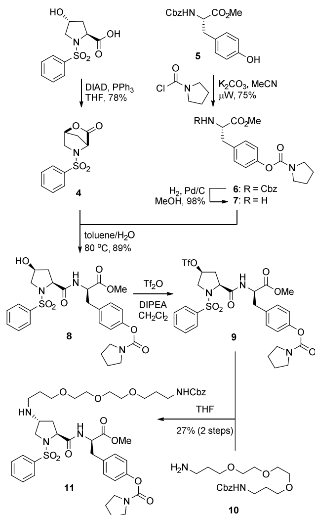
Scheme 1. Synthesis of PEGylated derivative via triflate displacement approach
