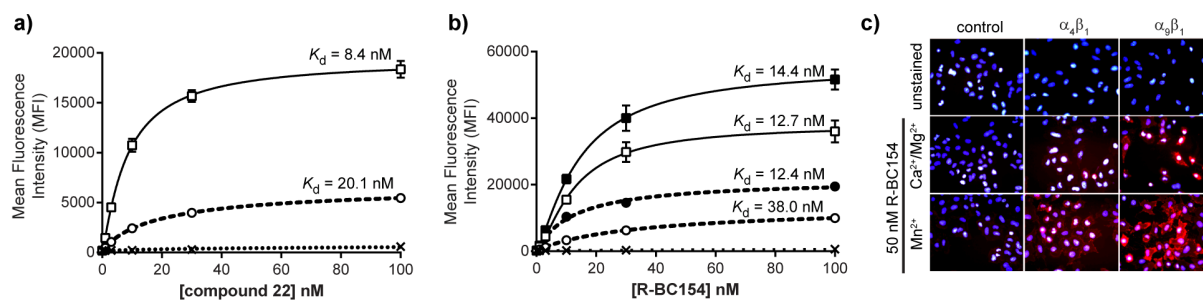
Figure 3. Saturation binding experiment of compound 22 and R-BC154 to control (no integrins; cross-dotted line), \alpha_4\beta_1 (circle-dashed line) and \alpha_9\beta_1 (square-solid line) LN18 cells with a) compound 22 in the presence of 1 mM \text{Ca}^{2+}/\text{Mg}^{2+} (open symbol) and b) R-BC154 in the presence of either 1 mM \text{Ca}^{2+}/\text{Mg}^{2+} (open symbol) or 1 mM \text{Mn}^{2+} (closed symbol). Data shown are expressed as mean fluorescence intensity (MFI) \pm SEM ( n = 3 ); c) Fluorescence microscopy images of over-expressing and control LN18 cells stained with 50 nM R-BC154 (red) under \text{Ca}^{2+}/\text{Mg}^{2+} and \text{Mn}^{2+} conditions. Cells were counterstained with DAPI (blue)
