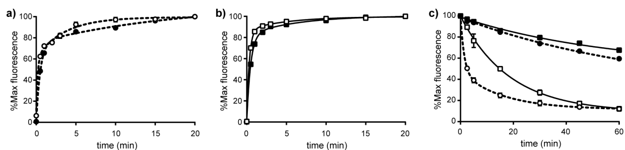
Figure 4. Kinetics measurements of R-BC154 binding to LN18 cells. Association rates for binding of R-BC154 to a) \alpha_4\beta_1 (circle-dashed line) and b) \alpha_9\beta_1 (square-solid line) integrins were determined in the presence of 1 mM \text{Ca}^{2+}/\text{Mg}^{2+} (open symbol) and 1 mM \text{Mn}^{2+} (closed symbol) in TBS buffer by treatment of cells with 50 nM R-BC154 for 0, 0.5, 1, 2, 3, 5, 10, 15 and 20 minutes at 37 °C; c) Dissociation rate measurements for binding of R-BC154 to \alpha_4\beta_1 (circle-dashed line) and \alpha_9\beta_1 (square-solid line) integrins were determined in the presence of
