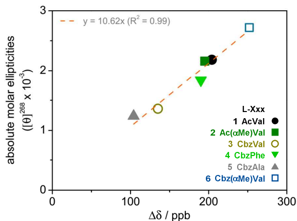
Figure 4. Relationship between the measured absolute molar ellipticities at 268 nm and the h.e. values for peptides 1-6.
