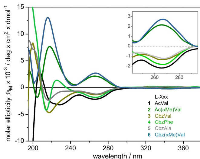
Figure 3. CD spectra of the endothiopeptides 1-6 in methanol. Inset: the region of the spectrum arising from the \pi - \pi^* transition of the thioamide chromophore.
