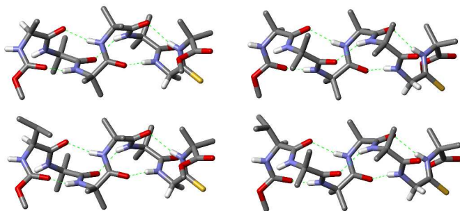
Figure 5. X-ray crystal structures of endothiopeptides 3 (top) and 5 (bottom) in their M (left) and P (right) conformations as observed in the unit cell. ‡ The M conformations display an N-terminal Type II \beta -turn while the P conformations display a Type III \beta -turn. 47 Cbz phenyl rings have been removed for clarity.
