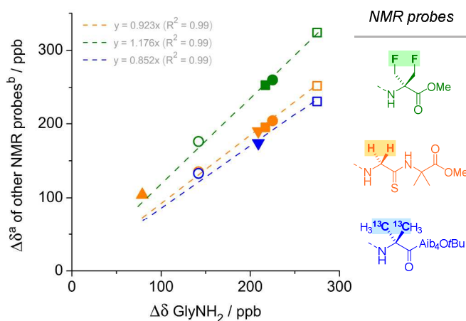
Figure 2. Comparing the performance of the glycine thioamide as a ^1H NMR probe with other NMR reporters of helical screw-sense; a for ^{13}C Aib probe (blue), \Delta\delta/10 ; b measured anisochronicity of the signals from highlighted nuclei in the ^1H , ^{13}C and ^{19}F NMR spectrum.
