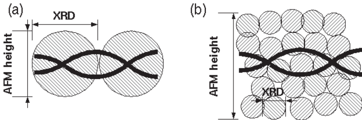
Figure 4: Schematics showing two types of nanowire structure. (a) A nanowire for which the AFM height measurements and Scherrer analysis of the powder X-ray patterns indicate similar crystallite sizes; such systems may undergo a transformation to a smooth nanowire described by equation (4). Examples include \text{Cu}_2\text{O}/\text{DNA} (Ref. [42]) and \text{Fe}_3\text{O}_4/\text{DNA} (Ref. [39]). (b) A nanowire where the crystallite size determined from the Scherrer analysis is much less than the height observed in AFM images; this nanowire is better understood in terms of the lattice gas model of section (2.3). Reprinted from ref. [55], Royal Society of Chemistry.
