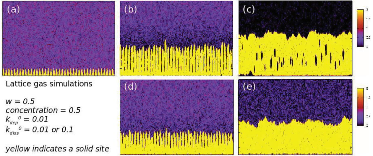
Figure 7: Lattice gas simulations of the growth of DNA-templated nanowires on a square lattice of 2000 \times 200 sites. The template lies along the x-axis in each figure. The colour scale indicates solid templated material for values in the range 1–2 (yellow) and dissolved atoms for values < 1 . The common parameters are w = 0.5 , concentration of dissolved metal ions, c = 0.5 (per site) and k_{dep}^0 = 0.01 . The initial state of the system was taken to be hemispherical nuclei of radius 20 sites on the x-axis, representing the DNA template. The simulations were run for 10^6 – 10^7 time steps: (a) t = 0 ; (b) k_{diss}^0 = 0.01 and t = 10^4 time-steps; (c) k_{diss}^0 = 0.01 and t = 10^7 time-steps; (d) k_{diss}^0 = 0.1 and t = 10^4 timesteps and (e) k_{diss}^0 = 0.1 and t = 10^7 time-steps. Reprinted from ref. [55], Royal Society of Chemistry.
