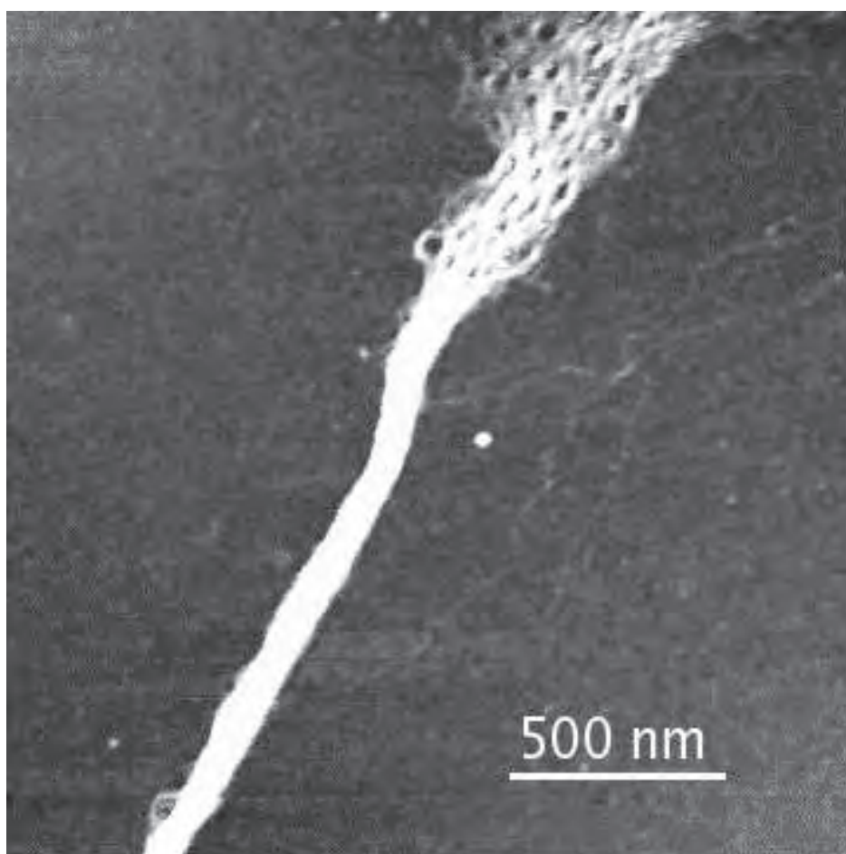
Figure 3: AFM image of polypyrrole nanowires on a \lambda -DNA template showing the formation of a thick rope that comprises strands which are themselves PPY/DNA nanowires and are seen unravelling at the end towards the top of the image. The image was recorded in Tapping Mode TM on an Si/SiO 2 substrate, the scale bar represents 500 nm and the grayscale represents 8 nm. Reprinted from ref. [52], with permission from Wiley, VCH.
