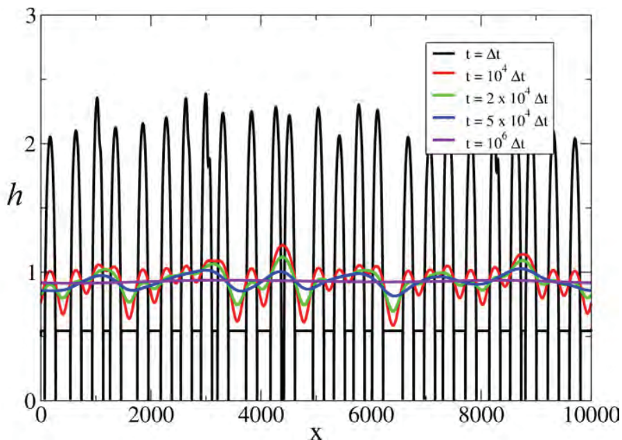
Figure 5: Numerical simulation using equation (4) showing the transition from beads-on-a-string to a smooth nanowire. The graph shows the thickness of templated material h(x) along the template X at various times. The deterministic part of equation (4) was integrated by a forward-time, centred-space explicit finite difference algorithm from an initial condition corresponding to nuclei of random heights and separation. \mu = 0.45 and r_T = 0.5 . Reprinted from ref. [56], with permission from IOP.
