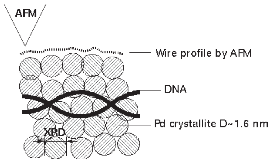
Figure 8: Schematic showing the structure of the Pd NWs which comprise small crystallites of diameter \simeq 1.6 nm by analysis of the X-ray diffraction pattern linewidth, but a relatively smooth & uniform appearance in AFM images [55].
