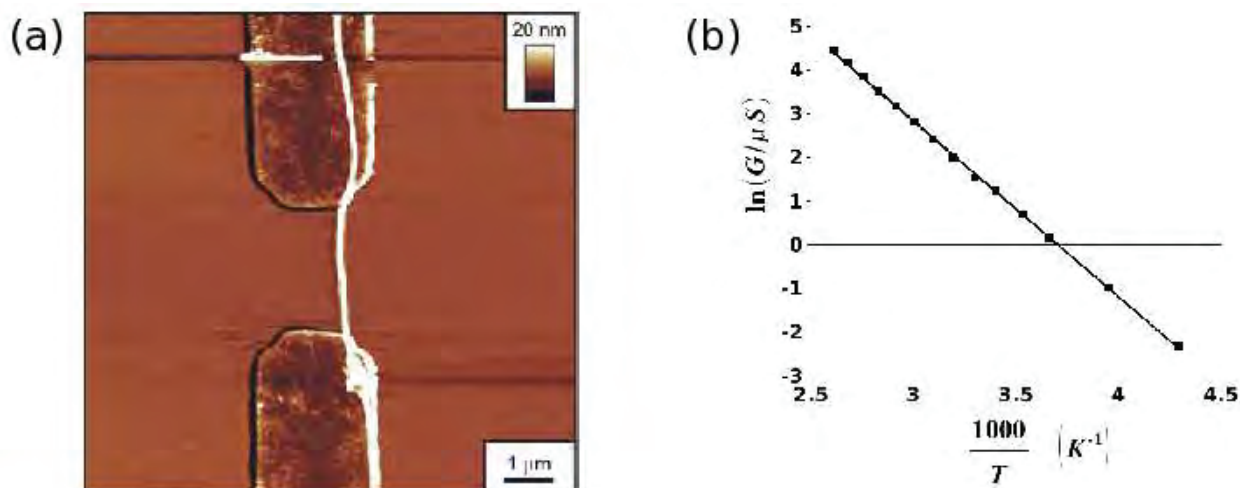
Figure 9: Two examples illustrating i-V characterisation of DNA-templated nanowires. (a) TappingMode AFM image of a poly(dithienylpyrrole)/DNA nanowire aligned across a 2.5 \mu\text{m} gap between two Au microelectrodes. The Au electrodes are embedded in a thermally grown, 200 nm thick insulating \text{SiO}_2 layer on a Si substrate so that the nanowire can more easily be aligned across the electrodes and so that the portions of the nanowire on the dielectric and on the electrodes can both be imaged. In the absence of a nanowire, the background current under a dry nitrogen atmosphere is \leq 10 \text{ fA} for bias voltages -5V < V_{bias} < 5V . Reprinted from ref. [46], with permission from Wiley, VCH. (b) Arrhenius plot for the zero-bias conductance of a poly(indole)/DNA nanowire of diameter 19 nm between gold contact electrodes of separation 1.7 \mu\text{m} . The fitted parameters are E_a = 33.5 \pm 0.2 \text{ kJ mol}^{-1} and G_0 = 3.0 \pm 0.25 \text{ S} . Reprinted from ref. [47], with permission from ACS.
