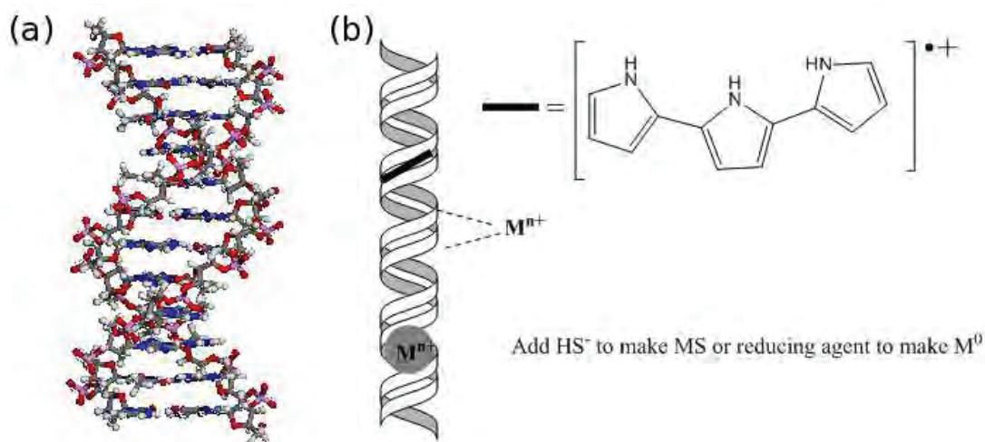
Figure 1: (a) Ball and stick model of duplex DNA. The colour scheme for the atoms is O (red), P (purple), C (grey) and N (blue). (b) Schematic illustrating possible binding modes of metal ions (to the phosphate groups and the nitrogen atoms of the nucleobases) and of short oligomers (in the minor groove). Binding of these species facilitates the nucleation of metals ( M^0 ), binary semiconductors (MS) and conductive polymers (e.g., poly(pyrrole)) on the DNA template.
