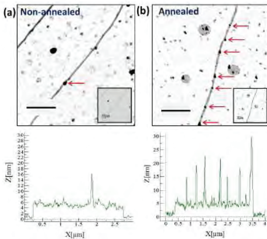
Figure 6: AFM height images of Cu-DNA before (a) and after annealing (b) at 400C for 1 hour. A transformation of the nanostructure surface morphology is observed, as indicated by the height profiles (below). Red arrows point to locations of larger nanoparticles along the structure. Insets show the path of the line trace along the nanostructure. Scale bars = 500 nm, height scales = 10 nm [26].
