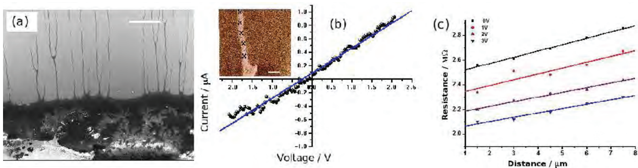
Figure 10: c-AFM measurements of Pd/DNA nanowires. (a) Electron micrograph of the dense mass of Pd/ DNA nanowires (lower third of image); single Pd/DNA nanowires are seen protruding from the mass (scale bar = 20 \mu\text{m} ). (b) Current–voltage curve with the tip contacting a single nanowire (inset = cAFM current image, data scale = 500 nA, tip/sample bias = 5 V, scale bar = 1 \mu\text{m} ). (c) cAFM measurements of resistance at different points along a single Pd/DNA nanowire. The distance is that between the point at which the tip contacts the nanowire and the dense mass shown in (a) & (b). The nanowire resistance per unit length is the slope of the plot and the intercept at zero distance is the contact resistance. Measurements obtained at different setpoints (tip/sample force) are shown in different colours. Reprinted from ref. [55], Royal Society of Chemistry.
