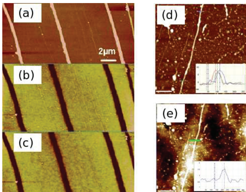
Figure 11: Electrical characterisation of Pd/DNA nanowires by scanned conductance microscopy. (a) AFM height image of Pd/DNA nanowires (the data scale is 25 nm). (b) and (c) are the corresponding SCM phase images of the same nanowires with applied bias voltages of +6 V and -6 V respectively (the data scale is 3). The dark contrast indicates that the nanowires are conductive. Reprinted from ref. [55], Royal Society of Chemistry. (d) AFM image of a \lambda -DNA molecule subjected to treatment with \text{Cu}(\text{CH}_3\text{CN})_4.\text{PF}_6 and phenylsilane to produce a copper nanowire (inset: height profiles of copper nanostructure taken at various points along the structure) and (e) the corresponding EFM phase image at an applied bias of 10V showing that the copper nanowire is insulating despite its continuous appearance. Scale bars= 500 nm. The colour scales of the images are (d) 20 nm and (e) 2 [26].
