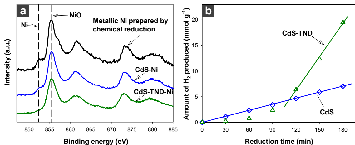
Figure 6. XPS spectrum of Ni 2p in the CdS-TND-Ni MPs after 2 hours of Ni 2+ reduction in comparison to that of Ni in CdS-Ni sample and metallic Ni nanoparticles prepared by chemical reduction using NaBH 4 as reducing agent and Ni(NO 3 ) 2 as nickel precursor (a). Amount of H 2 gas produced as a function of irradiation time during the photoreduction of Ni 2+ over CdS-TND composite (sample C 5 ) and CdS.
