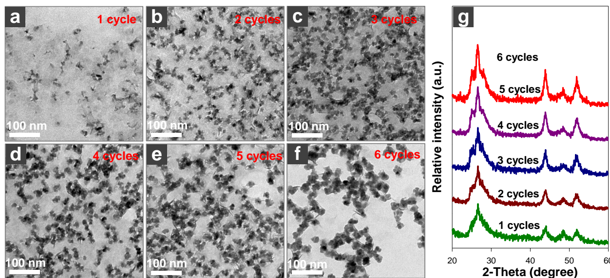
Figure 2. TEM images (a-f) and XRD patterns (g) of the CdS-TND composites obtained at different stages of the growth process.
