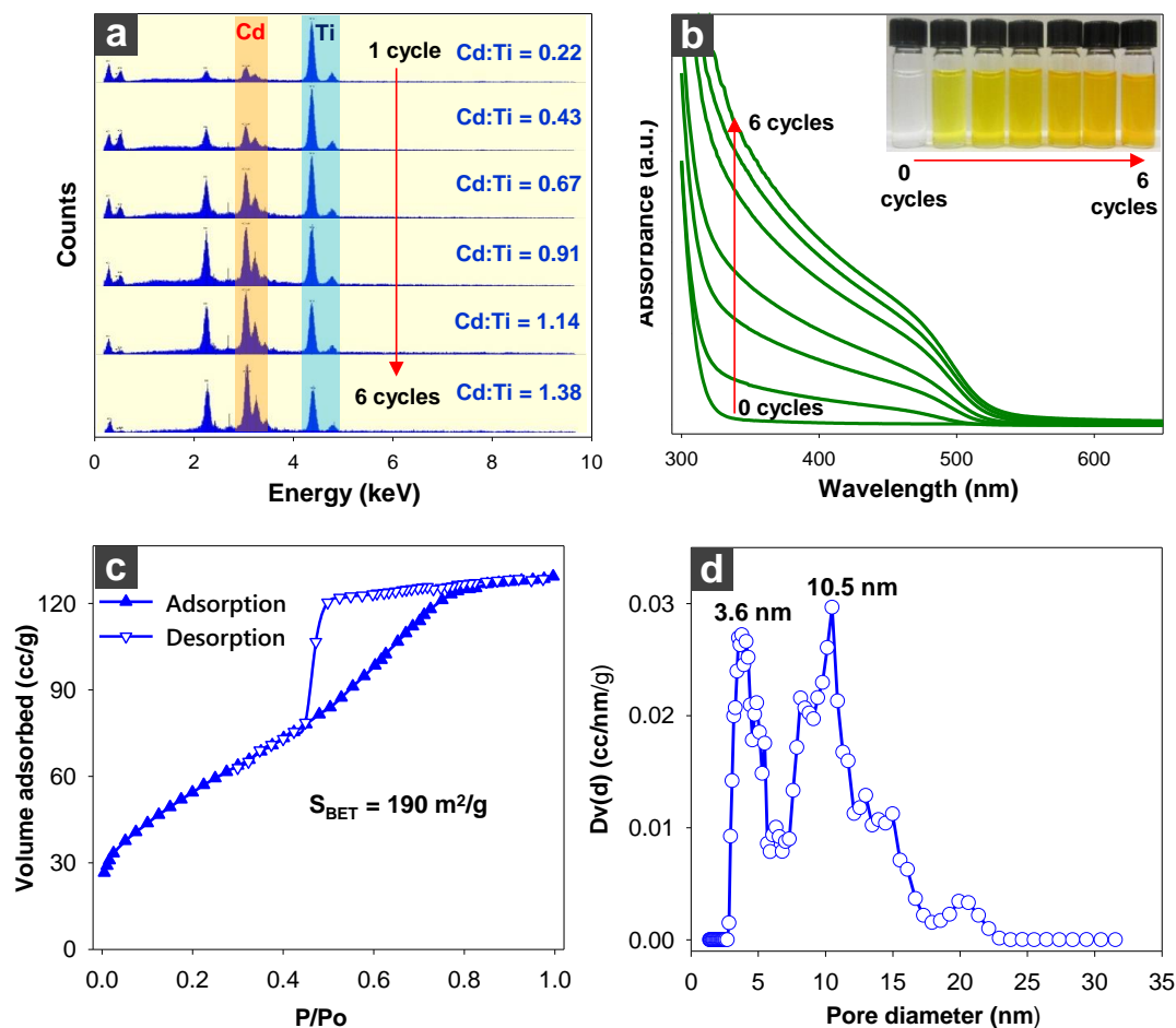
Figure 4. EDX (a) and UV-vis spectra (b), photographs (inset in b) of the CdS-TND composites obtained at different stages of the CdS growth process. Nitrogen sorption isotherms (c) measured at -196 °C for CdS-TND composites, obtained by 5 cycles of CdS growth, after the treatment with dilute HNO 3 to replace the TEA cations with H + and the respective NLDFT pore size distribution calculated from the adsorption branch (d).
