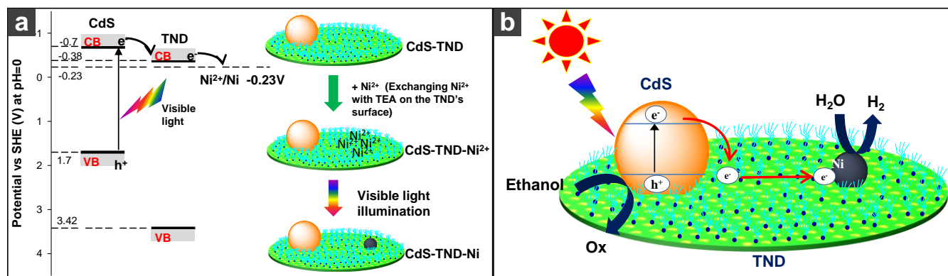
Figure 7. Schematic illustration of the electron transfer in the photoreduction of Ni^{2+} adsorbed on the surface of TNDs under visible light illumination and schematic illustration of the formation of Ni clusters on the surface of TND in the CdS-TND composites by visible light illumination (a). Schematic illustration of the charge transfer in CdS-TND-Ni MPs in the photocatalytic H_2 production from water-ethanol mixture under visible light. To simplify, only one particle of each component is shown, although a MP colloid is composed of several CdS NPs, TNDs and Ni clusters.
