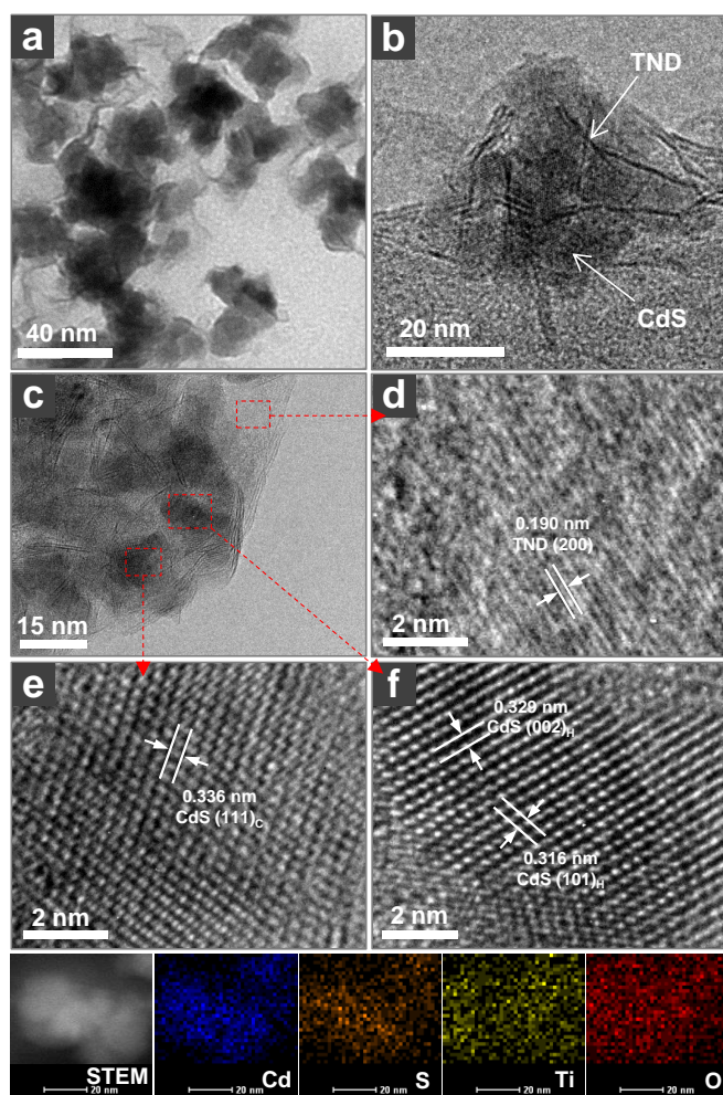
Figure 3. TEM (a, b), HRTEM (c-f) images and EDX elemental mapping data (lower panel) of the CdS-TND composite obtained by 5 cycles of CdS growth.
