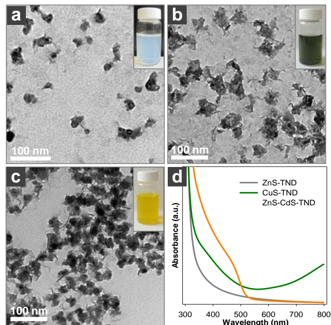
Figure 8. (a) TEM images of: ZnS-TND composites obtained by 3 cycles of ZnS growth. (b) CuS-TND composite obtained by 4 cycles of CuS growth. (c) ZnS-CdS-TND composite obtained by 3 cycles of CdS growth and 2 cycles of ZnS growth. (d) UV-vis spectra of different metal sulfide-TND composites. Insets in a, b, c are photograph of the corresponding metal sulfide-TND composite solutions.
