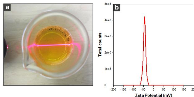
Figure 1. Photograph of the CdS-TND solution with a typical Tyndall Effect of colloidal solution (a). Zeta potential of CdS-TND composite colloidal solution measured at pH = 7.5 (b).
