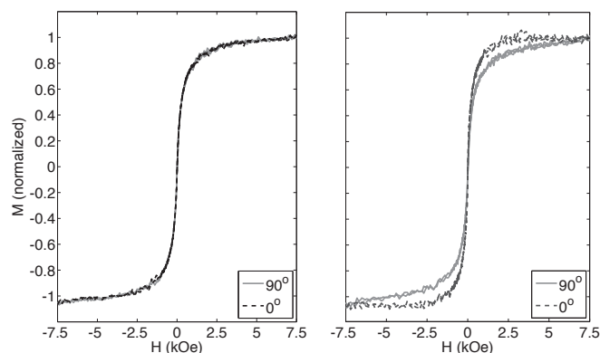
Fig. 2 Normalized M-H characteristics of the normal (left) and magnetically programmed (right) samples over two in-plane directions taken by VSM. The first has the same magnetization characteristics over all directions. For the latter 0^\circ shows the direction of the lines and 90^\circ shows perpendicular to lines.
