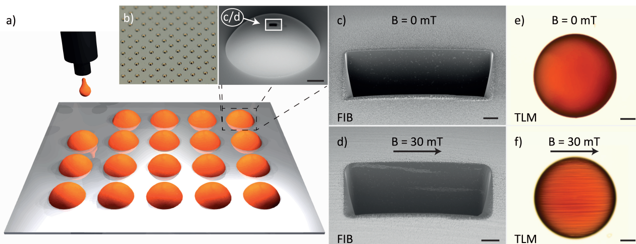
Fig. 1 The MPC hemispheres are fabricated by inkjet printing (a) (scale bar of inlet is 50\mu\text{m} ). The photo of an array of MPC hemispheres is shown (b). The cross sectional SEM image of the normal MPC (c) and anisotropic MPC (d) obtained by FIB cut (scale bar is 2\mu\text{m} ). In normal MPC (c) the nanoparticles are homogeneously distributed in the polymer matrix. In MA MPC (d) the formed lines are approximately 2\mu\text{m} apart from each other. The microscope image of the normal hemisphere is shown in (e) and the MA hemisphere in (f) (scale bar is 50\mu\text{m} ). The nanoparticles can not be seen normally, but the lines of nanoparticles in the MA hemisphere can be seen easily by an optical microscope.
