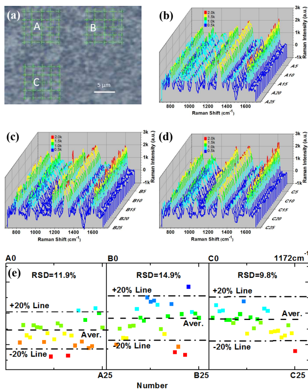
Fig. 5 (a) Optical image of the flat film obtained via the double sided tape-assisted film transformation method; (b) - (d) SERS spectra obtained from the point by point scanning of the three regions shown in (a) measured by a 633 nm excitation laser; (e) The intensity of the main Raman vibrations of CV molecule at the concentration of 10^{-10} M.
