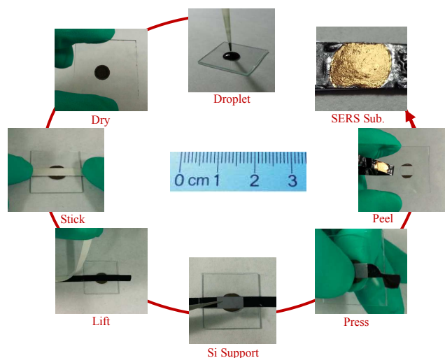
Scheme 2. Flow-process diagram of the procedures for fabricating SERS substrate using HAAA-NUs by double sided tape-assisted film transformation method.
