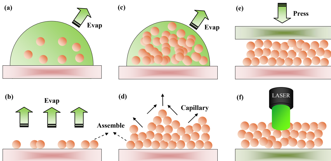
Scheme 1. The schematic plots of solvent evaporation and double sided tape-assisted film transformation. The formation of a film with (a)-(b) a thin layer, (c)-(d) a thick layer, (e) the double sided tape-assisted film transformation process, (f) SERS detection of the obtained inverted surface.
