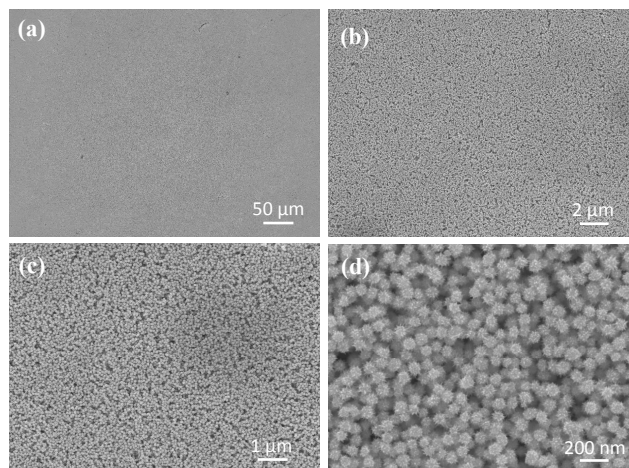
Fig. 2 (a) Low magnified SEM image of the SERS substrate with \sim 0.4 mm in width and \sim 0.5 mm in length; (b) - (d) Different magnified SEM images of the SERS substrate.
