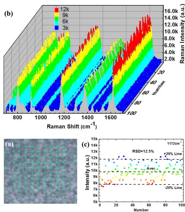
Fig. 4 (a) optical images of flat film obtained from via double sided tape-assisted film transformation method; (b) SERS spectra obtained from the point by point scanning of the area show in (a) measured by a 633 nm excitation laser; (c) The intensity of the main Raman vibrations of CV at the concentration of 10^{-8}\text{ M} .
