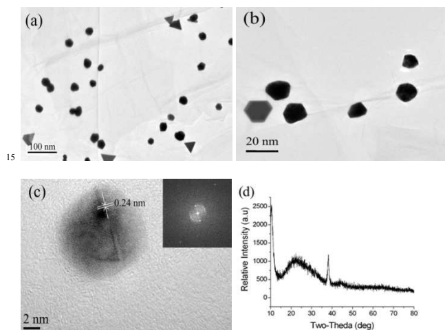
Fig.1 Low (a, b) and high (c) resolution TEM images, and XRD pattern (d) of AuNCs decorated on GO with 20% oxygen content. The inset in (c) is the fast Fourier transform (FFT) of the high resolution TEM (HRTEM) image.
