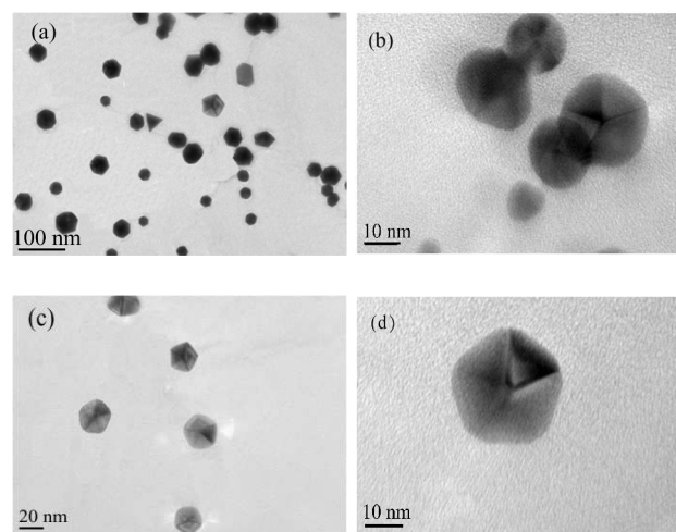
Fig.3 TEM images of AuNCs decorated on GO with 10% (a, b) and 5% (c, d) oxygen.
