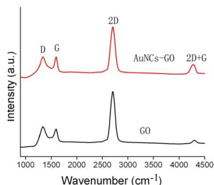
Fig.6 The Raman spectra of GO and AuNCs-GO with 5% oxygen.
