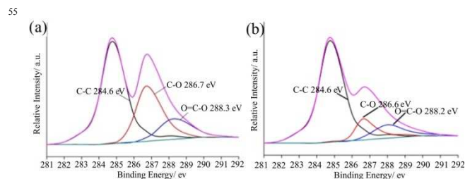
Fig.2 XPS of \text{C}_{1s} on GO (a) and AuNCs-GO (b) with 20% oxygen content.
