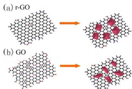
Fig.4 Schematic AuNCs growth on graphene with low (a) and high (b) degree of oxidation.
