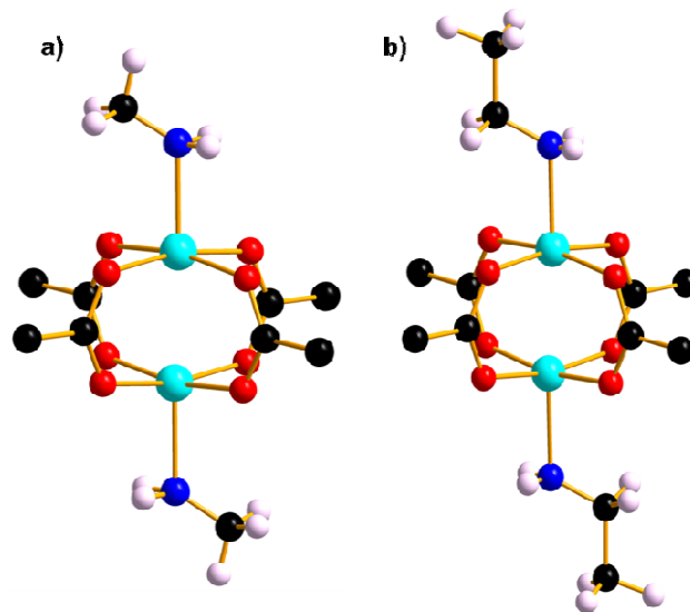
Fig. 7 Cu paddle wheel units in (a) STAM-1 MeNH 2 and (b) STAM-1 EiNH 2 . The part-occupied amine ligands are shown at full occupancy.
