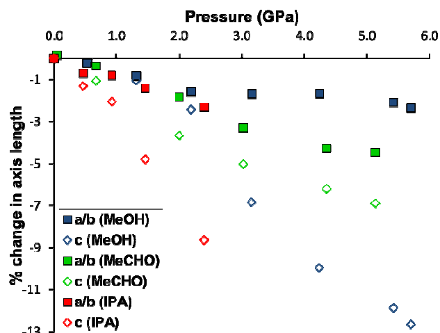
Fig. 6 Change in the length of the a/b -(squares) and c -axes (open diamonds) of STAM-1 in methanol (blue), acetaldehyde (green) and IPA (red) as a function of pressure.
