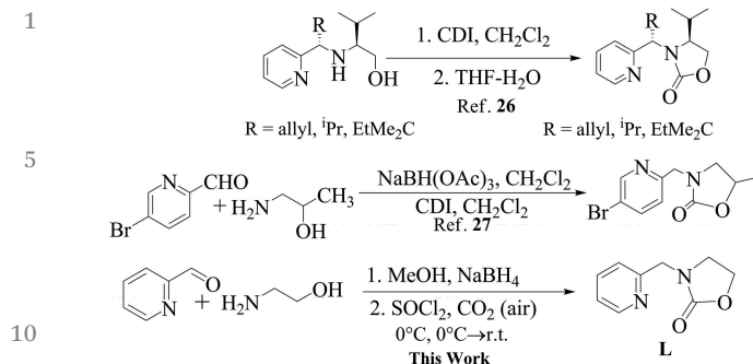
Scheme 2 Synthetic method of pyridine based oxazolidinone compounds reported earlier and ligand L in this work.
