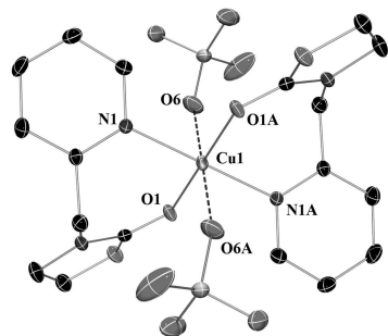
Fig. 1 Diagram of complex 1 with 50% probability thermal ellipsoids. Hydrogen atoms have been omitted for clarity. Symmetry transformations used to generate equivalent atoms: A = -x + 1, -y, -z + 2 .
