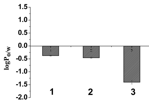
Fig. 3 Lipophilicity of complexes 1–3 represented by a bar diagram showing comparative \log P values of 1–3 in octanol–water system, where error bars in the graph represent the standard deviation in measurement.
