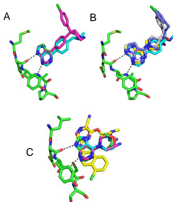
Fig. 2 A) Overlay of 1 (green, 2UVX), 2 (cyan, 2UVY), 4 (magenta, 2UWO) bound to PKB-PKA chimera; B) Overlay of 1 (green, 2UVX), 5 (cyan, 2VNW), 6 (yellow, 2VNY), 7 (grey, 2VO6) bound to PKB-PKA chimera and 8 (blue, 2X39) bound to PKB \beta ; C) Overlay of 9 (green, 2WMU), 10 (cyan, 2WMV), 11 (magenta, 2YM6), 13 (yellow, 2YM8) bound to CHK1. Kinase hinge regions (GK to GK+4, green) and hydrogen bonds from fragments 1 or 9 (dashed lines) are shown.
