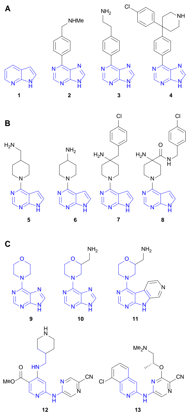
Fig. 1 Three fragment-to-lead series of kinase inhibitors. A) and B) PKB inhibitors developed from 7-azaindole ( 1 ); C) CHK1 inhibitors developed from 4-(9H-purin-6-yl)morpholine ( 9 ). The heavy atom footprint of the fragment preserved in the elaborated molecules is indicated in blue.
