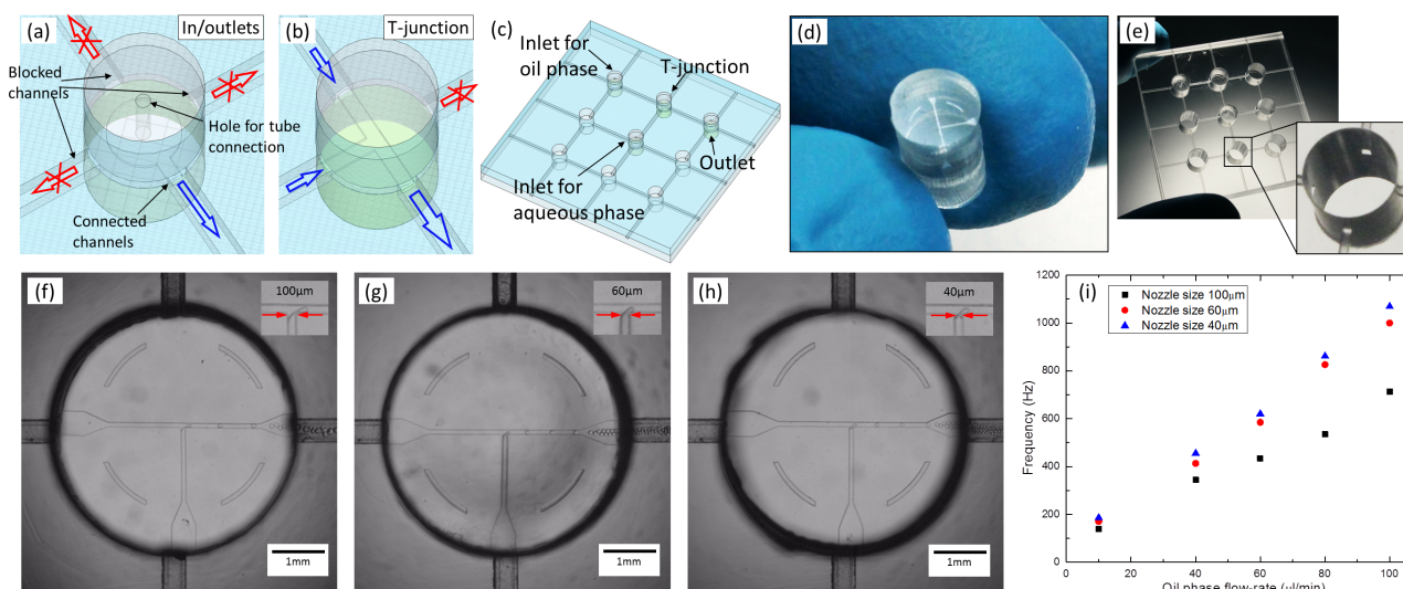
Fig. 3 Example of the modular microfluidic system for droplet formation using a T-junction. (a) in/outlet module (b) one T-junction module (c) Integration of four modules on the scaffold. Photograph of the (d) T-junction module and the (e) module integrated scaffold. (f,g,h) Droplet production using three T-junction modules with three different nozzle sizes (100 μm (f), 60 μm (g) and 40 μm (h)), and (i) measured frequency of the droplet production. The T-junction modules have simply been replaced on the scaffold between the successive experiments.
