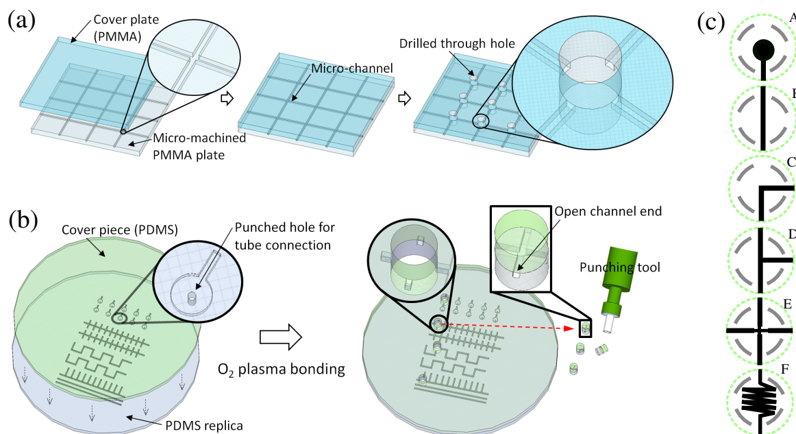
Fig. 1 Modular fabrication of a microfluidic chip (a) PMMA scaffold fabrication process, and (b) PDMS functional modules. (c) schematic representation of the functions for the functional units (A:Inlet/Outlet, B,C:Linkers, D:T-junction, E:Flow focusing, F:Incubation line.)
