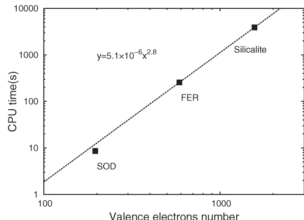
Fig. 2 CPU time (per processor per dynamic step) scaling with system size expressed as the number of valence electrons.
