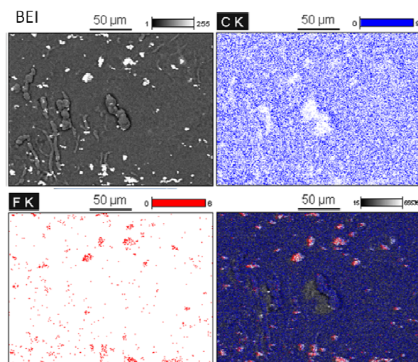
Fig. 6 Carbon and fluorine elemental distribution maps for the magnified area shown in Figure 5. Note the correspondence between bright spots in BEI image and fluorine-rich areas in the elemental map.
