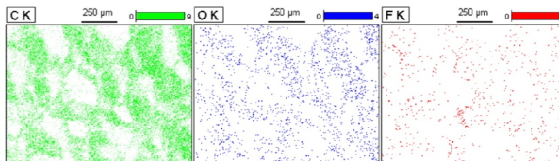
Fig. 3 EDX elemental distribution maps of a negative area of LDPE foam. Note the superposition of dotted areas in the C, O and F maps and the variability of dot density.
