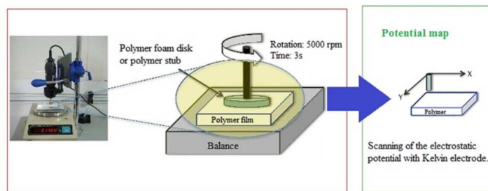
Fig. 1 Experimental sketch of a tribocharging experiment.
