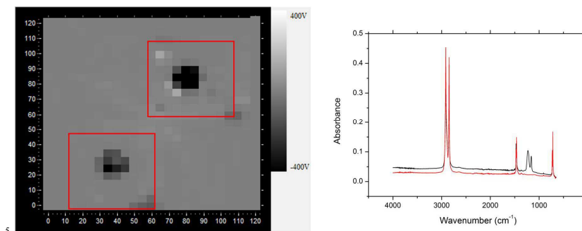
Fig. 4 (Left) Electrostatic potential maps of HDPE film sheared with a PTFE stub. (Right) Infrared spectra of a sheared area carrying negative charge (black) and a pristine area (red) of HDPE film tribocharged with PTFE.
