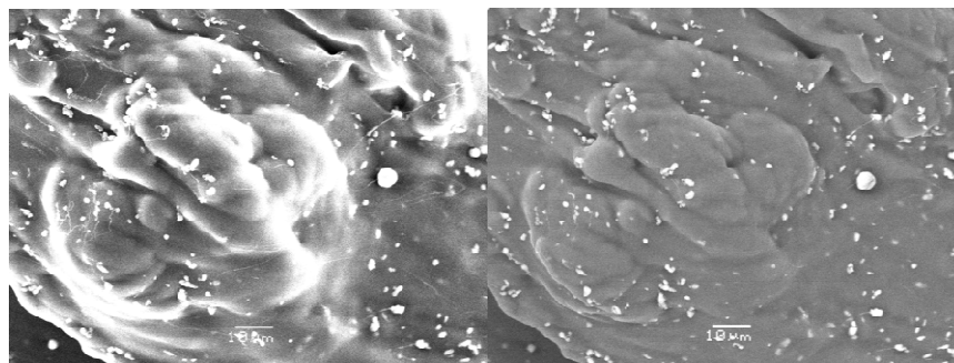
Fig. 11 Micrographs of a PS slab sheared with PTFE stub. Left, SEI; right, BEI.
