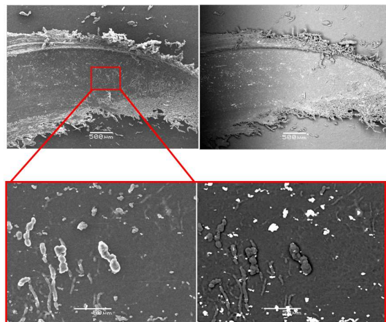
Fig. 5 SEI (left) and BEI (right) micrographs of an area of HDPE film sheared with a PTFE stub.
