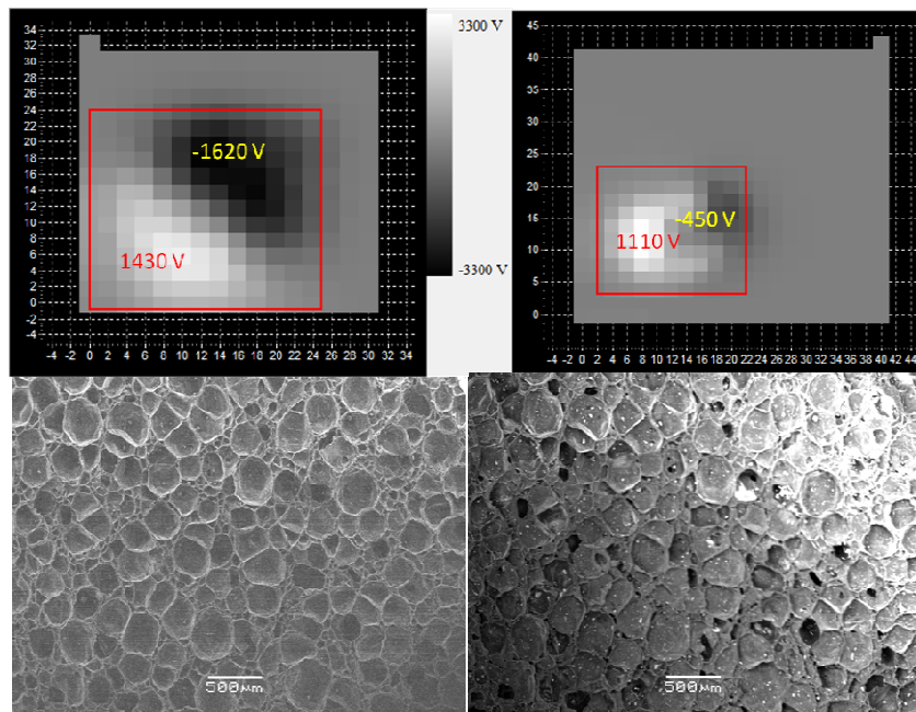
Fig. 2 (Top) Electrostatic potential maps of PTFE film (left) sheared with LDPE foam slabs (right). Average potential of positive and negative region of each material is printed in the respective area. (Bottom left) SEI micrograph of a negative area of sheared LDPE foam. (Bottom right) BEI micrograph of the same area.
