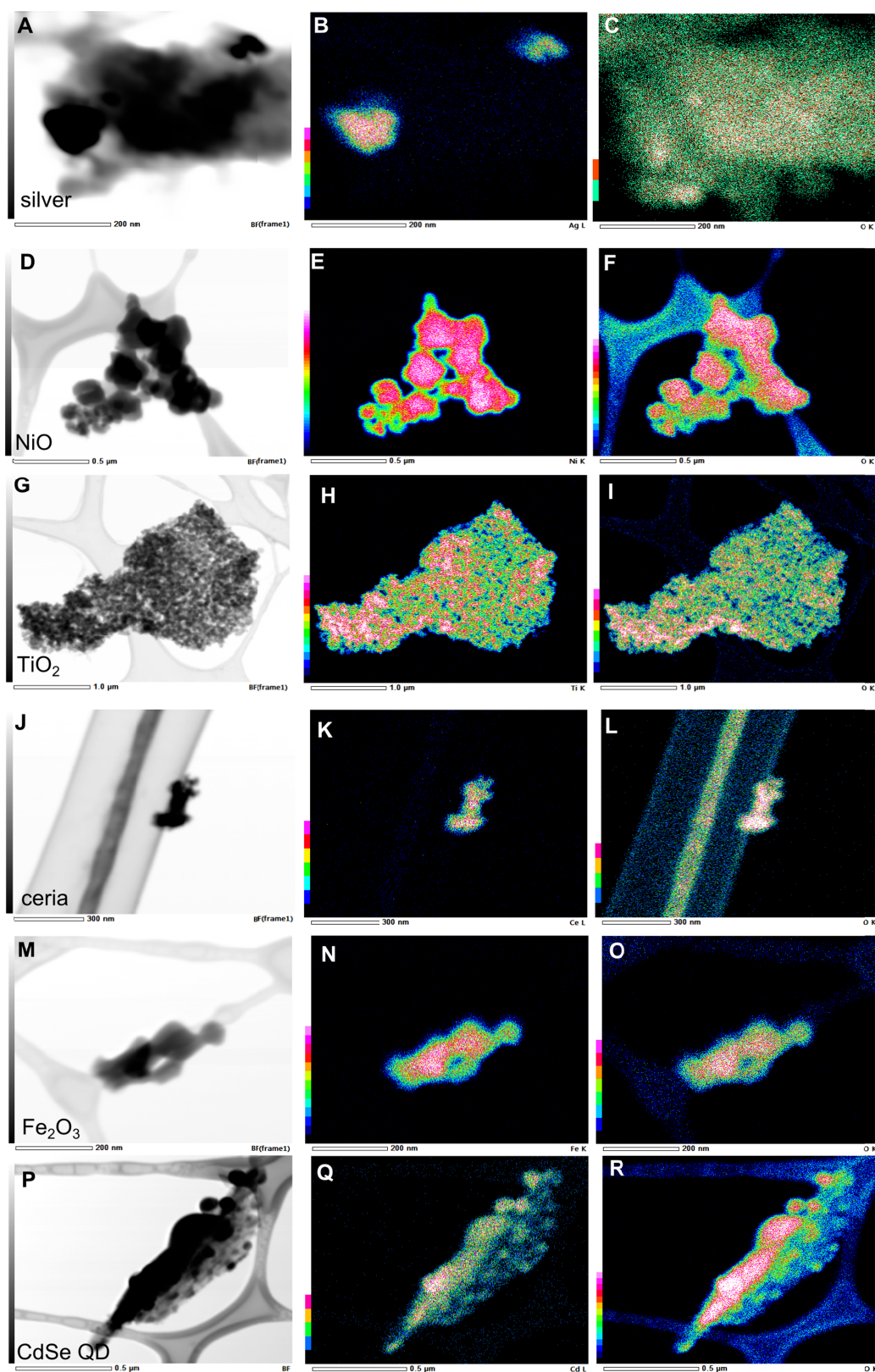
Fig. 5 Brightfield images of particles from waste containing (A) silver, (D) NiO, (G) TiO 2 , (J) ceria, (M) Fe 2 O 3 , and (P) CdSe QD. EDX maps of the metal of interest whose brightfield images are shown on the left that contains (B) silver, (E) NiO, (H) TiO 2 , (K) ceria, (N) Fe 2 O 3 , and (Q) CdSe QD nanomaterials. (C), (F), (I), (L), (O), and (R) are the oxygen signals suggesting the preservation or formation of the metal oxide system. Brighter colors indicate higher X-ray counts.
