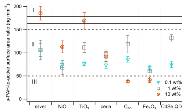
Fig. 3 Ratio of s -PAH to active surface area. Error bars are the propagated uncertainty (Equation 1, Supplementary Information). The solid black lines delineate the ratio of s -PAH to active surface area for the unspiked control waste. Data for 10 wt% CdSe QD are not available.
