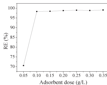
Fig. 10 Effect of CuZn-1 dose on the adsorption of MO, the initial MO concentration is 0.05\text{ g L}^{-1} .
