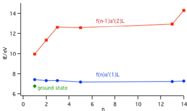
Figure 10. Plot of the IE to the lowest energy state of a configuration across the lanthanide series; red points are associated with an f^{n-1}a'^2L configuration and blue points with an f^n a'^1L configuration. The green point represents the ground state of CeCp_3^+
