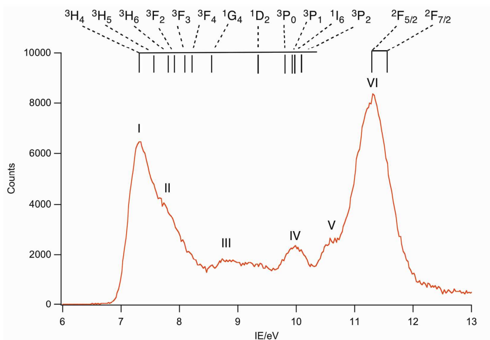
Figure 6. Difference of PE spectrum at 125 eV minus PE spectrum at 110 eV for PrCp 3 . The highest energy 4f band, VI, is assigned to the 2 F states.
