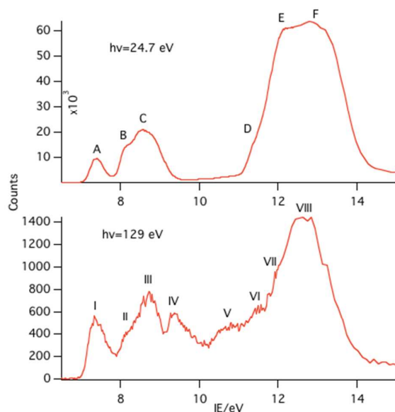
Figure 2. PE spectra of NdCp 3 with photon energies of 24.7 and 129 eV.
