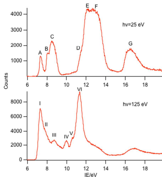
Figure 1. PE spectra of \text{PrCp}_3 with photon energies of 25 and 125 eV.
