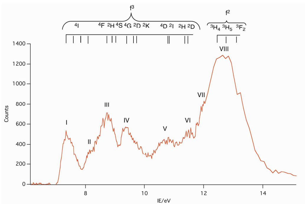
Figure 7. Difference of PE spectrum at 129 eV minus PE spectrum at 110 eV for NdCp 3 showing the energy range of identified 4f^3 spin-orbit states for \text{Nd}^{3+} and shows the likely energy range of 4f^2 states for \text{NdCp}_3^{3+} accessible by direct photoionization.
