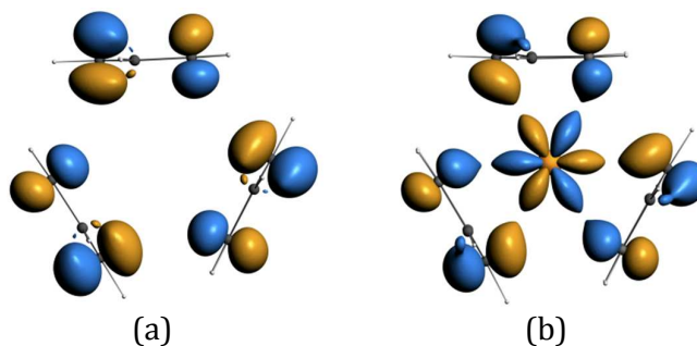
Figure 5. (a) the cp\pi a' symmetry adapted linear combination (b) possible overlap with \cos 3\phi component of the Ln 4f_{\pm 3} orbitals.. (These isosurfaces at value 4.8 were generated for CeCp_3^+ using the ADF program suite BP/TZP.) 19
