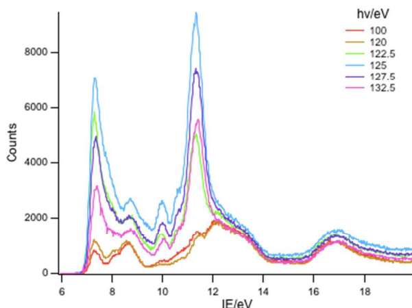
Figure 4. PE spectra of \text{PrCp}_3 with photon energies 100 – 132.5 eV.
