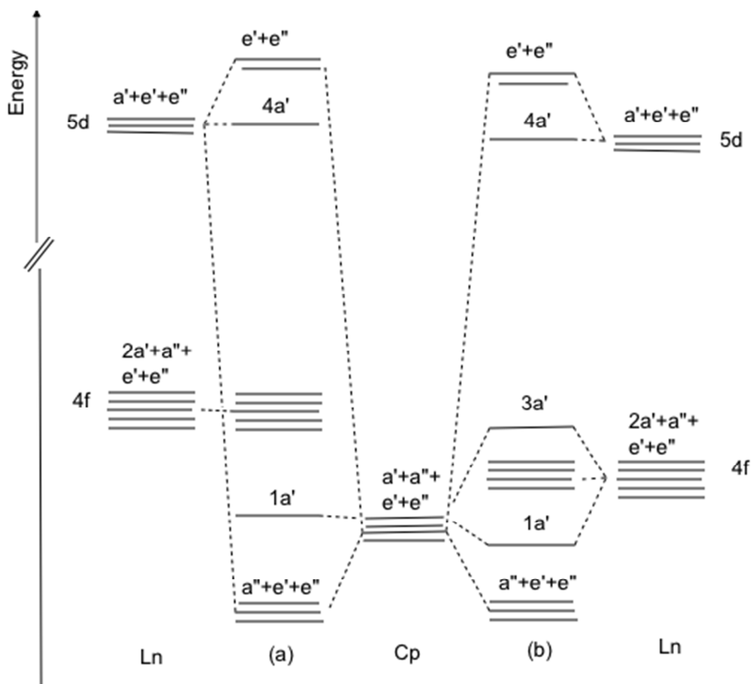
Figure 9. Orbital interaction diagram for \text{LnCp}_3 (a) 4f orbitals non-interacting (b) 4f orbitals close in energy to ring \pi a' orbital.
