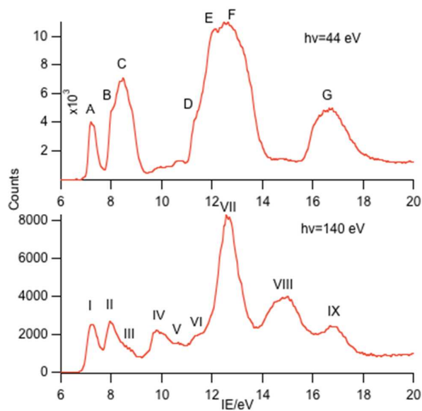
Figure 3. PE spectra of SmCp 3 with photon energies of 44 and 140 eV.
