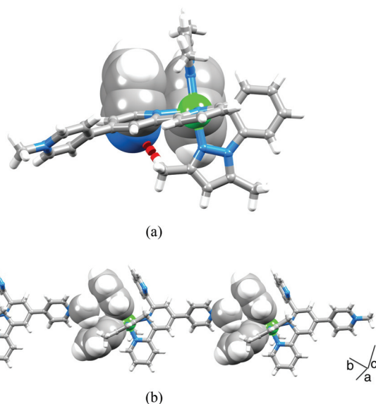
Fig. 6 (a) Structure of the [\text{Ir}(\text{dmppz})_2(\text{Mepytpy})]^{2+} cation showing face-to-face \pi -stacking and \text{CH}_{\text{Me}}\cdots\text{N} short contact (in red). (b) Cations assemble into chains through \pi\cdots\text{H}_{\text{Me}} contacts.
