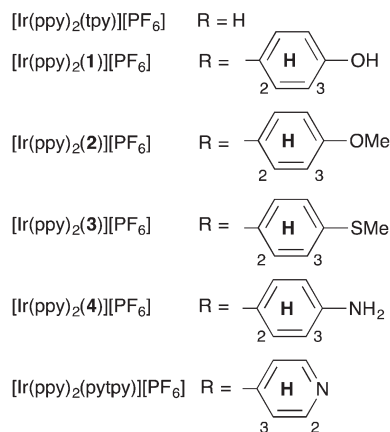
Scheme 2 Syntheses of [\text{Ir}(\text{ppy})_2(\text{N}^{\wedge}\text{N})][\text{PF}_6] complexes. Conditions: (i) N ^ N ligand, MeOH, microwave reactor 120 °C, time (see the Experimental section); (ii) \text{NH}_4\text{PF}_6 . Atom and ring labels used for NMR spectroscopic assignments are shown.
