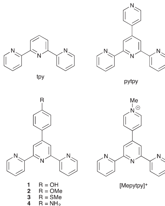
Scheme 1 Structures of the \text{N}^{\wedge}\text{N} ligands.
