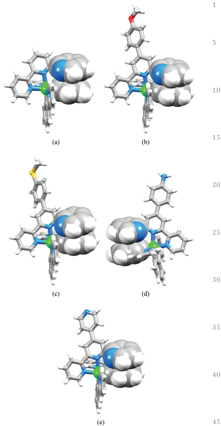
Fig. 3 Intra-cation \pi -interactions in (a) [\text{Ir}(\text{ppy})_2(\text{tpy})]^+ (one of two independent cations), (b) [\text{Ir}(\text{ppy})_2(2)]^+ (one of two independent cations), (c) [\text{Ir}(\text{ppy})_2(3)]^+ , (d) [\text{Ir}(\text{ppy})_2(4)]^+ and (e) [\text{Ir}(\text{ppy})_2(\text{pytpy})]^+ (one of two independent cations). Nitrogen atoms are shown in blue.
