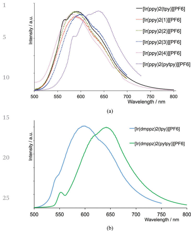
Fig. 8 Solution photoluminescence spectra of \text{CH}_2\text{Cl}_2 solutions of (a) [\text{Ir}(\text{ppy})_2(\text{N}^{\wedge}\text{N})]\text{PF}_6 and (b) [\text{Ir}(\text{dmppz})_2(\text{N}^{\wedge}\text{N})]\text{PF}_6 .
