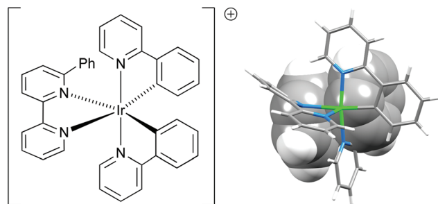
Fig. 1 Schematic representation of [\text{Ir}(\text{ppy})_2(6\text{-Phbpy})]^+ and structural figure showing the face-to-face stacking of the phenyl substitution and phenyl ring of one [\text{ppy}]^- ligand.
