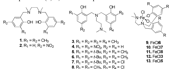
Chart 1. Ligands and complexes in this study.
