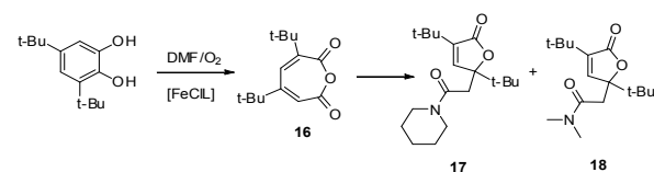
Scheme 2. Catechol oxidation products.
