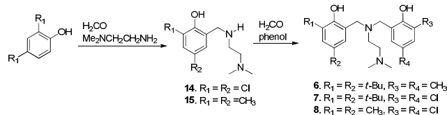
Scheme 1. Synthetic approach for ligands 6-8 .
