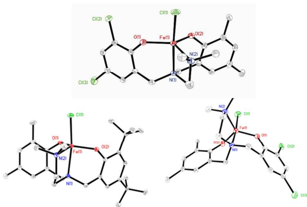
Figure 1. Thermal ellipsoid plots of the single crystal X-ray crystallographic structures of 9-11 . Ellipsoids are drawn at 50% and hydrogen atoms are omitted for clarity.
