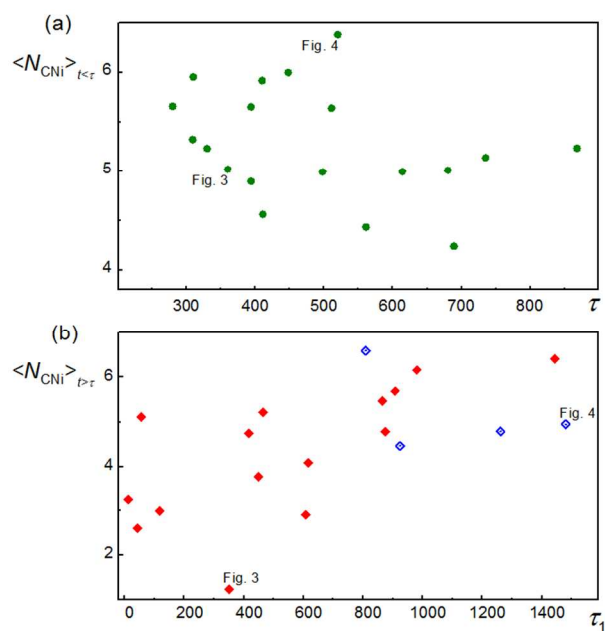
Fig. 5. (a) Calculated number \langle N_{CNI} \rangle_{t < \tau} of two-coordinated and one-coordinated carbon atoms bonded to the cluster averaged from the start of the simulations to the moment of graphene folding as a function of the graphene-heterofullerene transformation time \tau (in s) under electron irradiation in HRTEM. (b) Calculated number \langle N_{CNI} \rangle_{t > \tau} of two-coordinated and one-coordinated carbon atoms bonded to the cluster averaged from the moment of graphene folding to the moment of cluster desorption (filled symbols) or to the end of simulations (open symbols) as a function of the heterofullerene lifetime \tau_1 (in s) under electron irradiation in HRTEM. The data corresponding to evolution of structure presented in Figs. 3 and 4 are indicated.
