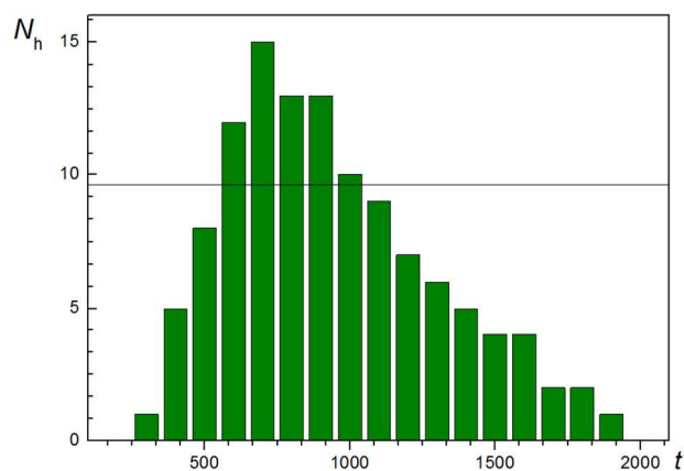
Fig. 6. Calculated number N_h of heterostructures in the transformation stage between the moments of graphene folding and cluster desorption for 19 simulation runs at different moments of time t (in s) under electron irradiation in HRTEM. The horizontal line corresponds to the 50% yield of heterostructures.
