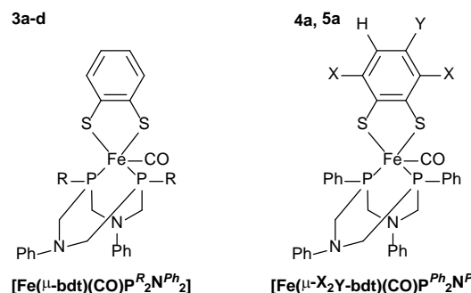
Figure 5. Overview of the mononuclear penta-coordinate Fe(II)-complexes, with its different substitutions at the bisphosphine ligand ( 3a R = Ph; 3b : R = benzyl; 3c : R = cyclo -hexyl; 3d : R = tert -Bu; left) and at the dithiolate bridge ( 4a : X = Cl, Y = H; 5a : X = H, Y = CH 3 ; right side).
