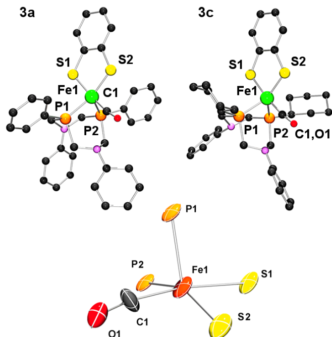
Figure 6. Molecular structures of 3a and 3c (top) and detailed view of the Fe(II) coordination mode of 3a (bottom). Note that compound 3c crystallizes with two independent complex molecules per unit cell and only one is depicted here. Thermal ellipsoids are drawn at 50% probability level. Hydrogen atoms and co-crystallized solvent molecules are omitted for clarity.
