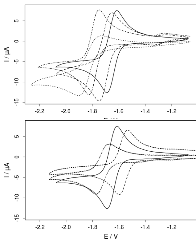
Figure 9. Top: Cyclic voltammograms of 3a (line), 3b (dashed), 3c (dotted) and 3d (dash-dotted). Bottom: CVs of 3a (line), 4a (dashed) and 5a (dotted) with a concentration of 1.0 M in acetonitrile. Conditions: scan rate of 100 \text{ mV s}^{-1} , 0.1 M (\text{Bu})_4\text{NPF}_6 as supporting electrolyte.
