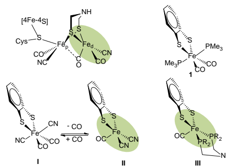
Figure 1 Schematic structure of the \text{H}_{\text{ox}} state of [FeFe] \text{H}_2\text{ase} active site highlighting free coordination site in the distal iron ( \text{Fe}_\text{d} ) (Top left). Hexacoordinate (I and \text{I}^{14} ) and penta-coordinate (II and III) mononuclear model complexes of \text{Fe}_\text{d} .
