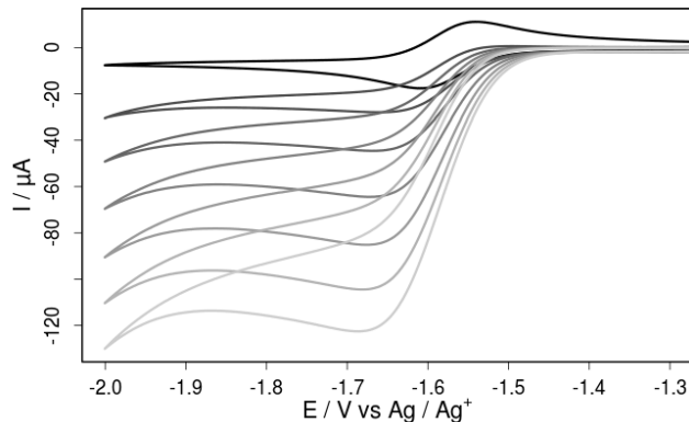
Figure 11. Cyclic voltammograms of 3a (1.0 mM) in acetonitrile solution in the absence (black) and presence (grey curves) of increasing AcOH concentrations (in steps of 50 eq from 0-300 eq). The increase in current in the presence of acid indicates that the proton reduction is catalyzed by the iron complex.
