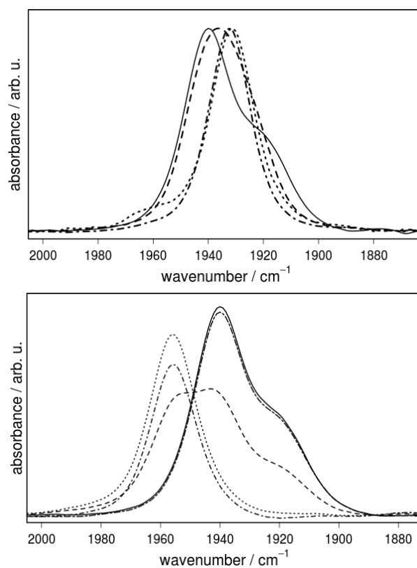
Figure 7. Top: normalized IR spectra of 3a (line), 3b (dashed), 3c (dotted) and 3d (dash-dotted) in acetonitrile in the region of the carbonyl stretching vibrations. Bottom: IR spectra of 3a in the absence of acid (line), with 1 eq. (dashed), 2 eq. (dotted), 5 eq. (dash-dotted) of triflic acid and deprotonated with 5 eq. triethylamine (dash long dotted). Acetonitrile at ambient temperatures.
