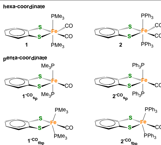
Figure 2. Conceivable coordination isomers that arise from the formal removal of one CO ligand from experimentally observed hexa-coordinate complexes 1 and 2 . sp = square pyramidal; tbp = trigonal bipyramidal
