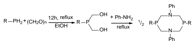
Scheme 2. Synthesis of cyclic bisphosphine ligands a-d ( P^R_2N^{Ph}_2 ) starting from primary phosphines and aniline: a : R = Ph (phenyl), b : R = Bn (benzyl), c : R = Cyc ( cyclo -hexyl) and d : R = t Bu ( tert -butyl)
