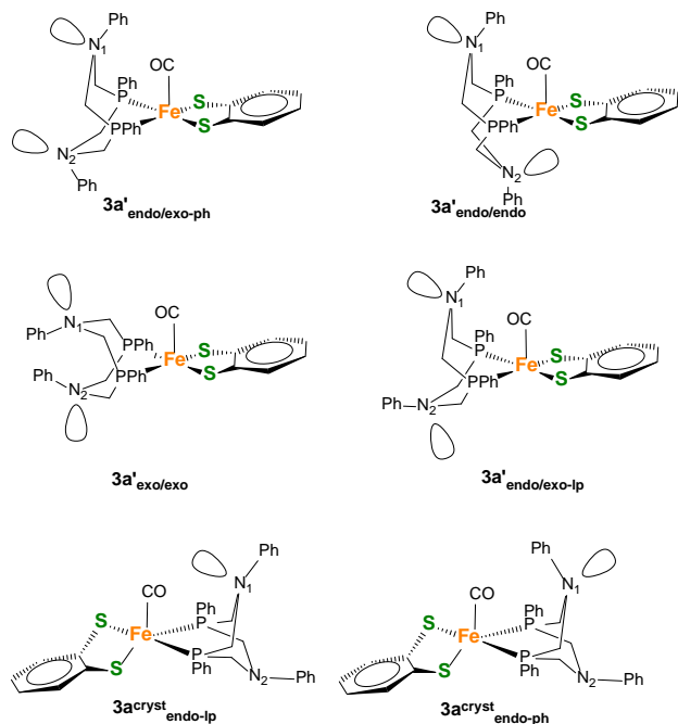
Figure 8. Potential coordination isomers 3a' and 3a^{\text{cryst}} with different endo/exo conformations of the 6-membered FePCNCP heterocycles as well as different orientations of the N-Ph substituent.
