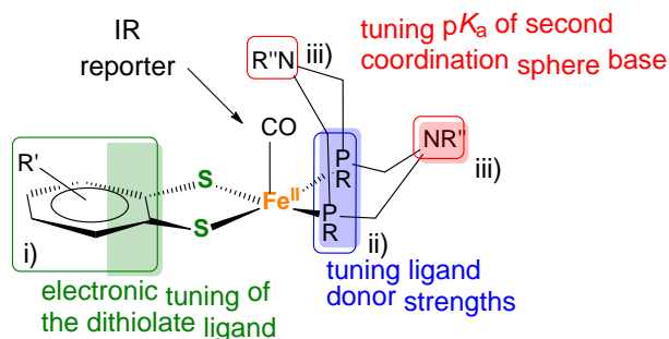
Figure 3. Modular design of mononuclear pentacoordinate iron complexes containing a \text{P}^{\text{R}}_2\text{N}^{\text{R}'_2} ligand and its three different possible sites i)-iii) of independent modifications.
