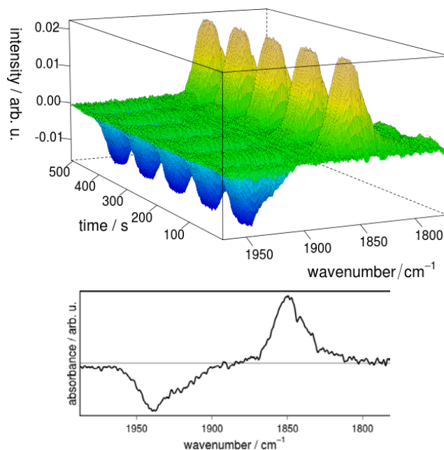
Figure 10. Fully reversible reduction-oxidation cycles of complex 3a in acetonitrile solution, monitored by FTIR spectro-electrochemistry. Time-dependent FTIR spectra of 3a red induced by reduction of 3a at -1.8 V and reoxidation at -1.4 V vs. \text{Ag}/\text{Ag}^+ , respectively, measured against the IR spectrum of 3a as background. The reduction-oxidation cycles (first five of 20 cycles à 100 seconds are shown) were performed without any loss or decomposition of compound.
