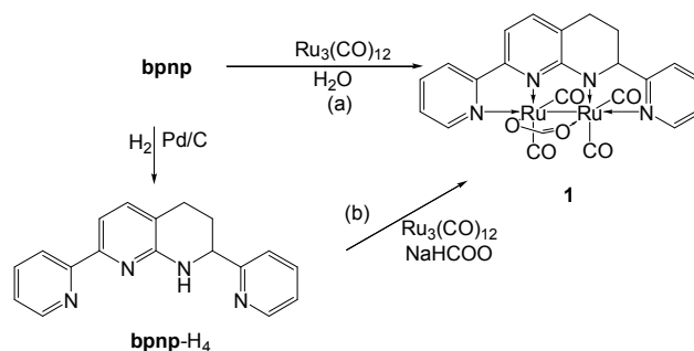
Scheme 1 Formation of diruthenium complex 1 .
