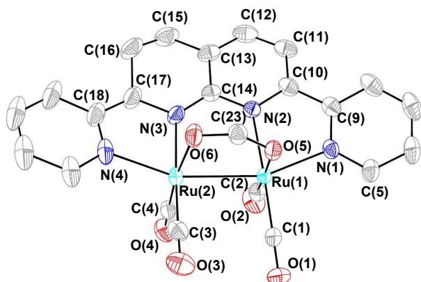
Fig. 1 ORTEP plot of 1 at the 30% probability level. Label of some aromatic carbons are omitted for clarity.
