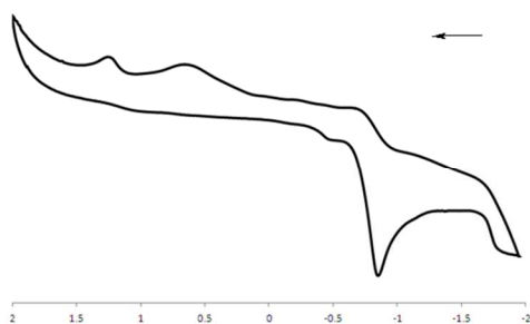
Fig. 2 Cyclic voltammogram for 1 with 0.1 M [Bu 4 N][PF 6 ] as the supporting electrolyte at a scanning rate of 100 mV/s.
