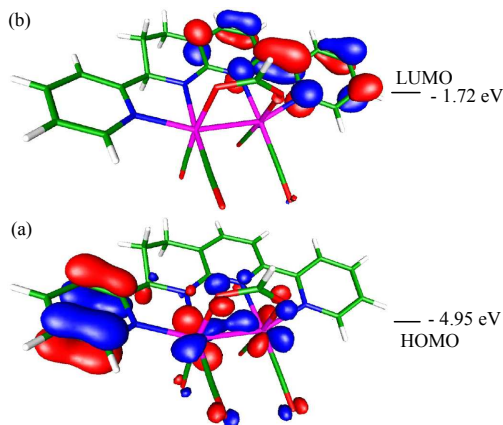
Fig. 3 HOMO (a) and LUMO (b) calculated for complex 1 .
