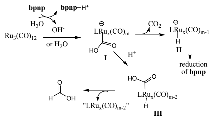
Scheme 2 Pathway for the formation of metal-hydride and the formate ligand
