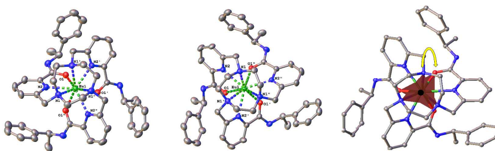
Figure 1 Views of the structures of the tripositively charged cations of S - \Delta -( \lambda\lambda\lambda )-[EuL 1 ] ( left ) and R - \Delta -( \delta\delta\delta )-[EuL 1 ] ( right ) (120 K), showing the twist angle (23.7°) associated with trigonal prismatic distortion, compared to 19.5° for [Eu.L 3 ] and 22.3° for [Eu.L 4 ]. CCDC 965909-911
