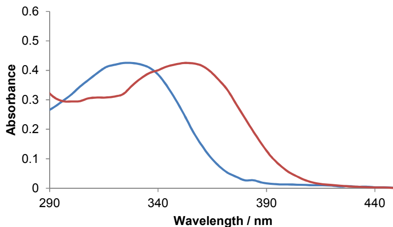
Figure 5 UV-absorption spectra of S\text{-[EuL}^{2c}\text{]Cl}_3 in i\text{PrOH:H}_2\text{O} (80:20 v/v) at an apparent pH of 10.3 (blue) and pH 4.4 (red).
