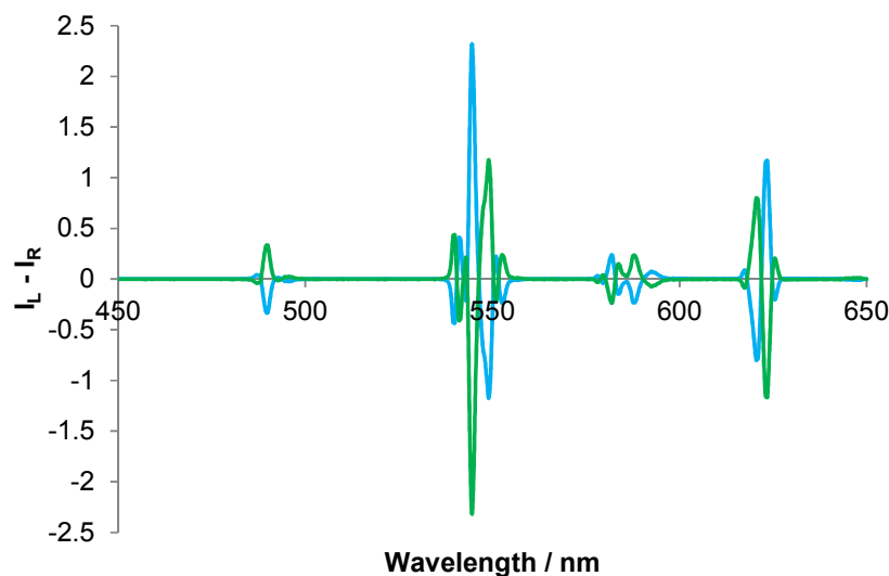
Figure 6 Circularly polarized luminescence emission spectra for S\text{-}\Delta (green) and R\text{-}\Lambda (blue) [\text{Tb.L}^1] ( \lambda_{\text{exc}} 280 nm; \text{H}_2\text{O} , pH 6.5, 295K; \Delta -complex: g_{\text{em}}(539) +0.11 ; g_{\text{em}}(623) -0.35 ).
