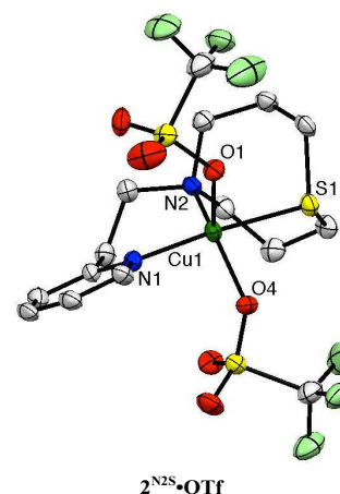
Fig. 4 ORTEP drawings of \mathbf{2}^{\text{N2S}}\cdot\text{OTf} showing 50 % probability thermal ellipsoids. Hydrogen atoms are omitted for clarity. \text{Cu}(1)-\text{S}(1) , 2.2860(15) Å; \text{Cu}(1)-\text{O}(1) , 2.247(4) Å; \text{Cu}(1)-\text{O}(4) , 2.118(4) Å; \text{Cu}(1)-\text{N}(1) , 2.006(5) Å; \text{Cu}(1)-\text{N}(2) , 2.040(6) Å; \text{S}(1)-\text{Cu}(1)-\text{O}(1) , 84.84(11)°; \text{S}(1)-\text{Cu}(1)-\text{O}(4) , 84.78(12)°; \text{S}(1)-\text{Cu}(1)-\text{N}(1) , 171.15(16)°; \text{S}(1)-\text{Cu}(1)-\text{N}(2) , 90.42(14)°; \text{O}(1)-\text{Cu}(1)-\text{O}(4) , 95.93(15)°; \text{O}(1)-\text{Cu}(1)-\text{N}(1) , 92.12(16)°; \text{O}(1)-\text{Cu}(1)-\text{N}(2) , 109.86(17)°; \text{O}(4)-\text{Cu}(1)-\text{N}(1) , 87.27(18)°; \text{O}(4)-\text{Cu}(1)-\text{N}(2) , 153.25(16)°; \text{N}(1)-\text{Cu}(1)-\text{N}(2) , 98.4(2)°.
