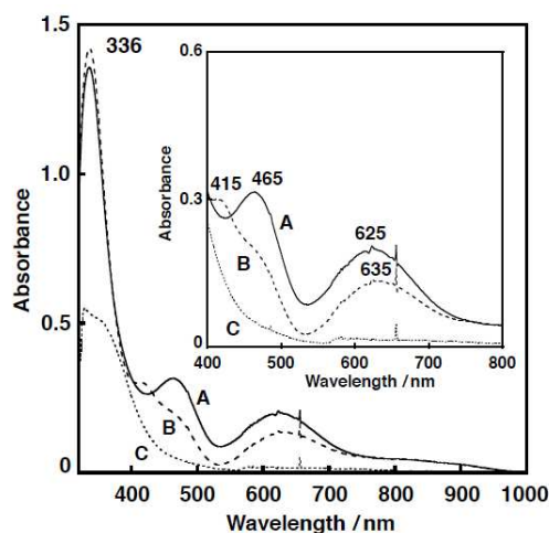
Fig. 7 The UV-vis spectra of Intermediate A (solid line; 1000 s after the reaction of 1^{N2S} (0.5 mM) with an equimolar amount of CmOOH in acetone at -85^{\circ}\text{C} ), B (dashed line; 1h after the reaction), and C (dotted line; after warming up to 30^{\circ}\text{C} ). Inset: Expanded spectra at 400–800 nm region.
