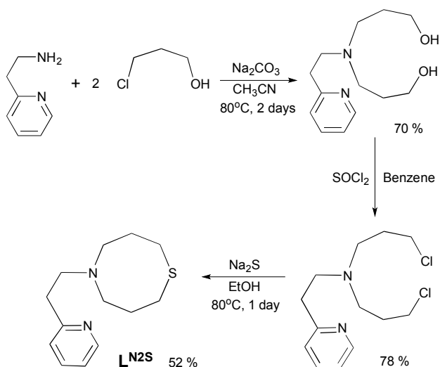
Scheme 1 Ligand synthesis.
