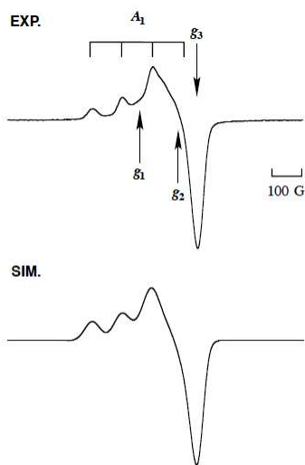
Fig. 6 The EPR spectrum (EXP, top) of 2^{N2S}\cdot OTf (0.5 mM) in acetone at -196^\circ C , and its computer simulation spectrum (SIM, bottom) with the parameters of g_1 = 2.275 , g_2 = 2.100 , g_3 = 2.015 , A_1 = 150 G, A_2 = 59 G, and A_3 = 16 G.
