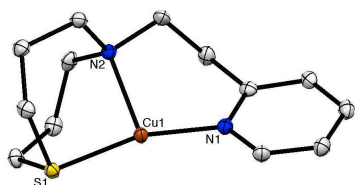
Fig. 2 ORTEP drawing of \mathbf{1}^{\text{N2S}} showing 50 % probability thermal ellipsoids. Counter anion ( \text{PF}_6^- ) and hydrogen atoms are omitted for clarity. \text{Cu}(1)-\text{S}(1) , 2.2028(4) Å; \text{Cu}(1)-\text{N}(1) , 1.9295(13) Å; \text{Cu}(1)-\text{N}(2) , 2.1662(13) Å; \text{S}(1)-\text{Cu}(1)-\text{N}(1) , 163.02(4)°; \text{S}(1)-\text{Cu}(1)-\text{N}(2) , 94.37(4)°; \text{N}(1)-\text{Cu}(1)-\text{N}(2) , 102.60(6)°.
