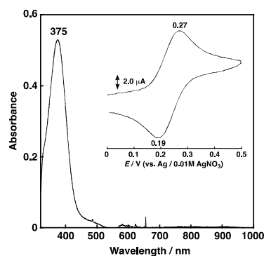
Fig. 3 UV-vis spectrum of \mathbf{1}^{\text{N2S}} (0.5 mM) in acetone at 25°C. Inset: Cyclic voltammogram of \mathbf{1}^{\text{N2S}} (1.0 mM) in acetone containing 0.1 M TBAPF 6 ; working electrode GC, counter electrode Pt, reference electrode Ag/0.01 M AgNO 3 , scan rate 50 mV/s.
