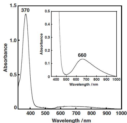
Fig. 5 The UV-vis spectrum of 2^{N2S}\cdot OTf (0.25 mM) in acetone, at -85^\circ C . \lambda_{max} = 370 nm ( \epsilon = 5520 M^{-1} cm^{-1} ). Inset: An expanded UV-vis spectrum of 2^{N2S}\cdot OTf (0.60 mM). \lambda_{max} = 660 nm ( \epsilon = 222 M^{-1} cm^{-1} ).
