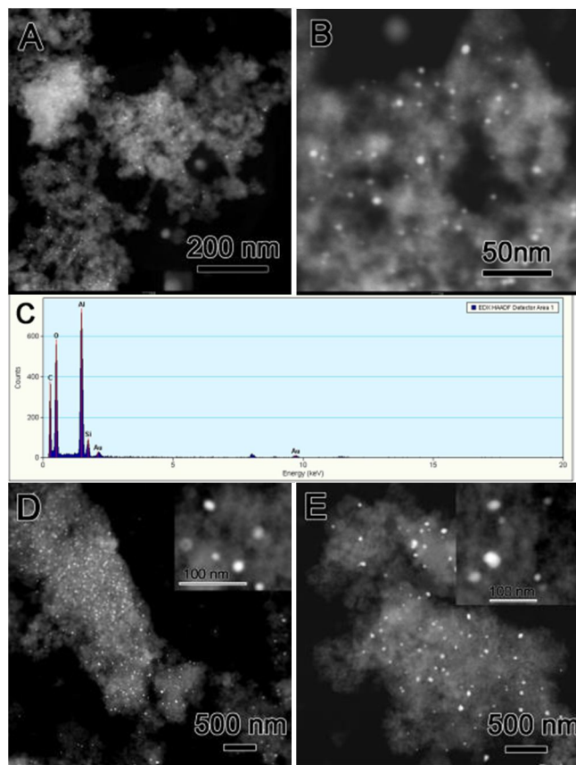
Figure 3. HAADF-STEM images of Au/SiO 2 @Al 2 O 3 catalyst (A, B) and the EDX analysis at the selected area (C); HAADF-STEM images of Au/SiO 2 @Al 2 O 3 catalyst calcined at 650 °C (D) and 750 °C (E).
