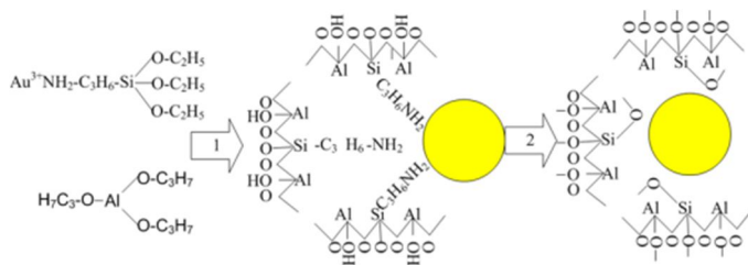
Figure 1 The schematic illustration of the simultaneous synthesis process of \text{Au}/\text{SiO}_2@\text{Al}_2\text{O}_3 . The arrow marked as ‘1’ signifies the reduction of gold and hydrolysis and condensation of aluminum alkoxide and APTES; the arrow marked as ‘2’ signifies the 5 hour calcination process at 500\text{ }^\circ\text{C} .
