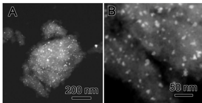
Figure 4. HAADF-STEM images of Au/Al 2 O 3 .
