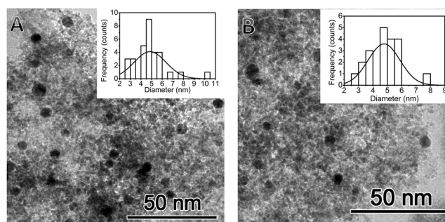
Figure 6. Bright-field TEM images of Au/SiO 2 @Al 2 O 3 catalyst before (A) and after (B) reaction at 120 °C.
