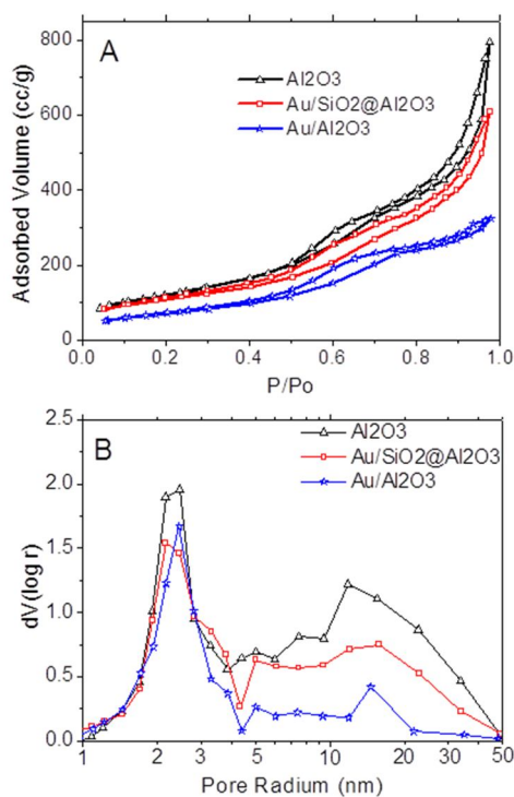
Figure 2. Nitrogen adsorption/desorption isotherms at -196\text{ }^\circ\text{C} (A) and BJH pore-size distribution (B) of \text{Au}/\text{SiO}_2@\text{Al}_2\text{O}_3 , \text{Au}/\text{Al}_2\text{O}_3 and \text{Al}_2\text{O}_3 aerogel.
