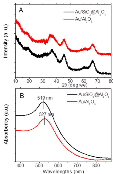
Figure 5. XRD spectra (A) and diffuse-reflectance UV-vis spectra (B) of Au/SiO 2 @Al 2 O 3 and Au/Al 2 O 3 catalysts.
