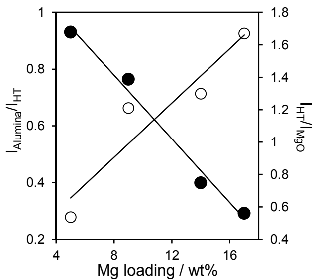
Fig. 6 Evolution of Mg-HT/ \text{Al}_2\text{O}_3 surface species as a function of bulk Mg loading
