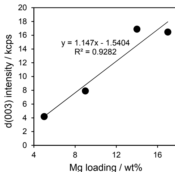
Fig. 2 Intensity of d(003) reflection of Mg-Al hydrotalcite phase as a function of bulk Mg loading
