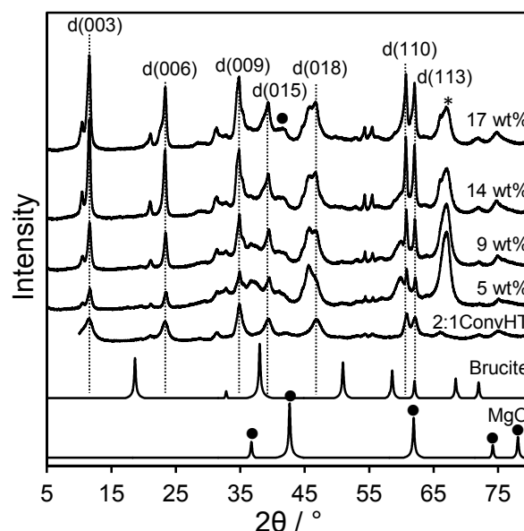
Fig. 1 XRD patterns for Mg-HT/ \text{Al}_2\text{O}_3 series as a function of bulk Mg loading alongside 2:1 ConvHT reference (* indicates parent \text{Al}_2\text{O}_3 and ● MgO)
