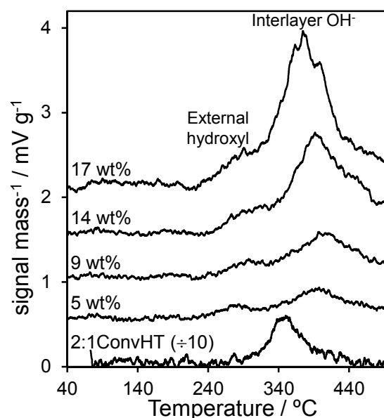
Fig. 4 CO 2 TPD profiles for Mg-HT/Al 2 O 3 series and convHT reference as a function of bulk Mg loading
