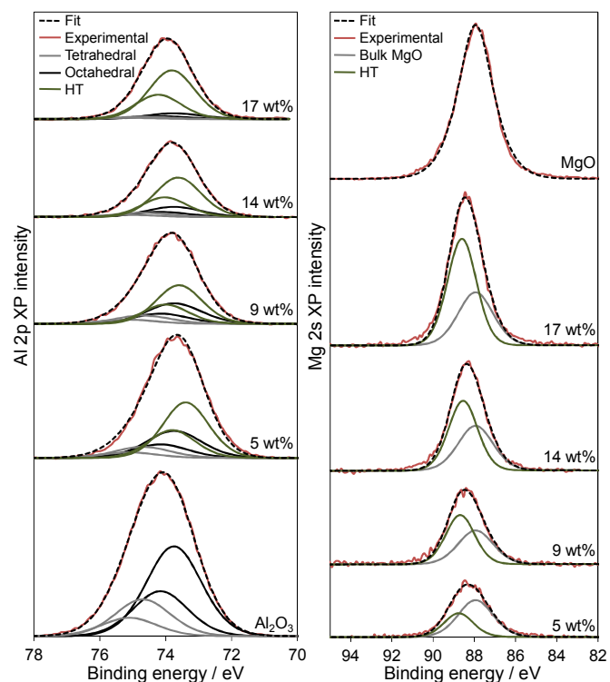
Fig. 5 (a) Al 2p and (b) Mg 2s XP spectra of Mg-HT/ \text{Al}_2\text{O}_3 series as a function of bulk Mg loading and pure \text{Al}_2\text{O}_3 and MgO references
