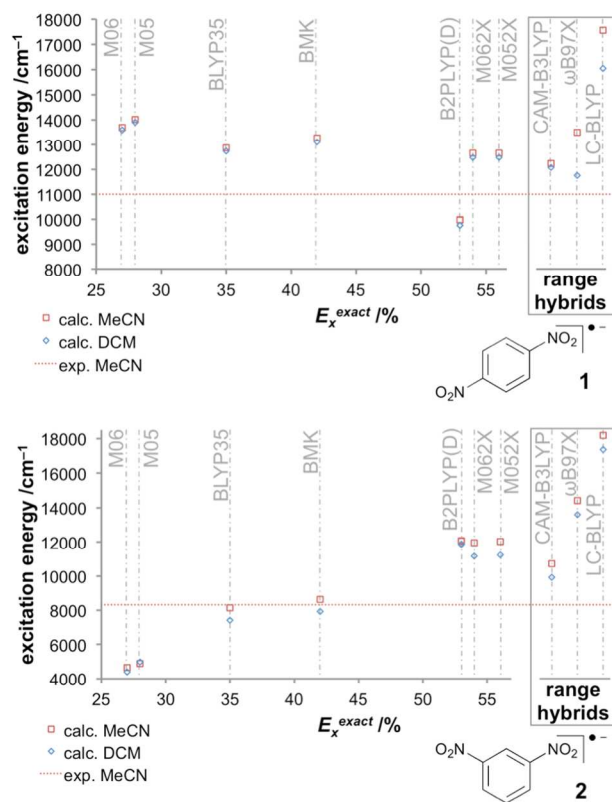
Figure 3. Computed excitation energies with different functionals for the class III system 1 (top) and for the class II system 2 (bottom) in two solvents (C-PCM) compared to experimental values in MeCN (11000 cm -1 for 1 and 8320 cm -1 for 2 ). 151 Reprinted with permission from M. Renz, M. Kess, M. Diedenhofen, A. Klamt and M. Kaupp, J. Chem. Theory Comput. , 2012, 8 , 4189. Copyright 2012 American Chemical Society.
