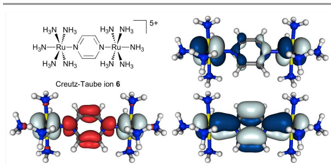
Figure 5. Isosurface plots of spin density (bottom left, \pm 0.002 a.u.) and \beta -SOMO (top right)/ \beta -HOMO (bottom right) ( \pm 0.03 a.u.) of the Creutz-Taube ion, 6 , calculated at the BLYP35/def2-SVP/COSMO(MeCN) level. 219 Adapted with permission from M. Parthey, J. B. G. Gluyas, M. A. Fox, P. J. Low and M. Kaupp, Chem. Eur. J. , accepted. Copyright © 2014 WILEY-VCH Verlag GmbH & Co. KGaA, Weinheim.
