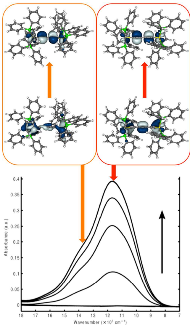
Figure 8. Isosurface plots ( \pm 0.03 a.u.) of the orbitals involved in the NIR transitions of 8 calculated at the BLYP35/(def2-)SVP/COSMO(CH 2 Cl 2 ) level and experimental spectrum collected during spectroelectrochemical oxidation in CH 2 Cl 2 / 0.1 M NBu 4 PF 6 . 158 The excitation around 14000 cm -1 only gains intensity for rotameric forms, which exhibit approximately orthogonal disposition of the Cp rings around the Ru 4 Ru axis. Adapted with permission from M. Parthey, J. B. G. Gluyas, P. A. Schauer, D. S. Yufit, J. A. K. Howard, M. Kaupp and P. J. Low, Chem. Eur. J. , 2013, 19 , 9780. Copyright © 2013 WILEY-VCH Verlag GmbH & Co. KGaA, Weinheim.
