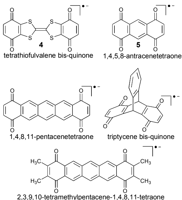
Figure 4. Some diquinone radical anions investigated.
