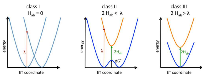
Figure 1. Potential curves for the three primary Robin-Day classes: Class I (left), class II (middle) and class III (right).
