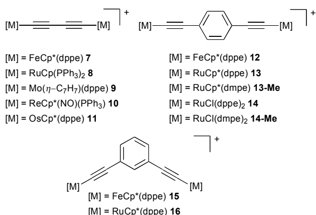
Figure 6. Diynediyl-bridged complexes 7-11 , diethynylphenyl-bridged complexes 12-16 , and the truncated models 13-Me and 14-Me , which were used to computationally investigate the influence of different conformers on the UV-vis-NIR and IR spectra of 13 and 14 .
