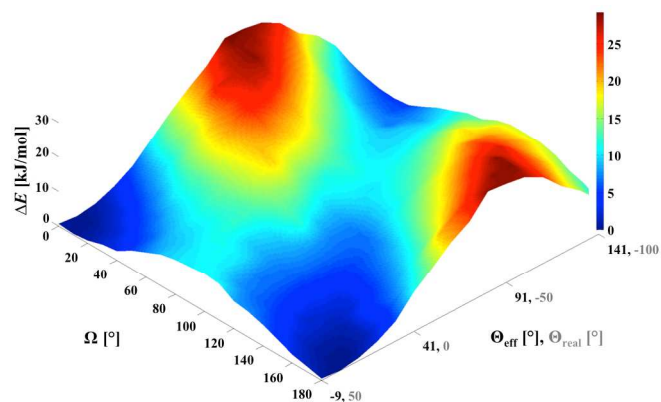
Figure 91. Computed potential energy surface of truncated 13-Me (BLYP35/COSMO(CH 2 Cl 2 ) level). 219 \Omega represents the dihedral angle for the redox centres and \Theta_{\text{eff}} for the bridge rotation. Adapted with permission from M. Parthey, J. B. G. Gluyas, M. A. Fox, P. J. Low and M. Kaupp, Chem. Eur. J. , accepted. Copyright © 2014 WILEY-VCH Verlag GmbH & Co. KGaA, Weinheim.
