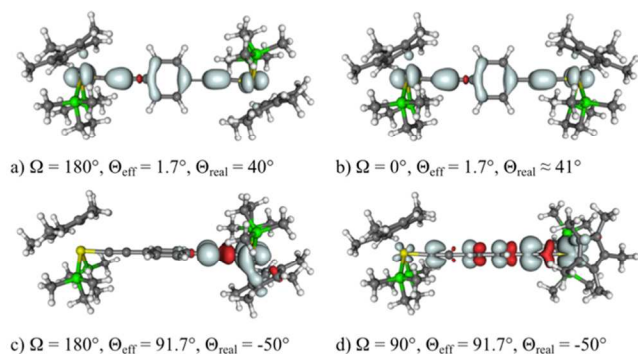
Figure 10. Spin density isosurface plots ( \pm 0.002 a.u.) of truncated 13-Me for different points on the potential energy surface (BLYP35/COSMO( \text{CH}_2\text{Cl}_2 ) level; cf. Figure 9 for the potential energy surface). 219 Adapted with permission from M. Parthey, J. B. G. Gluyas, M. A. Fox, P. J. Low and M. Kaupp, Chem. Eur. J. , accepted. Copyright © 2014 WILEY-VCH Verlag GmbH & Co. KGaA, Weinheim.
