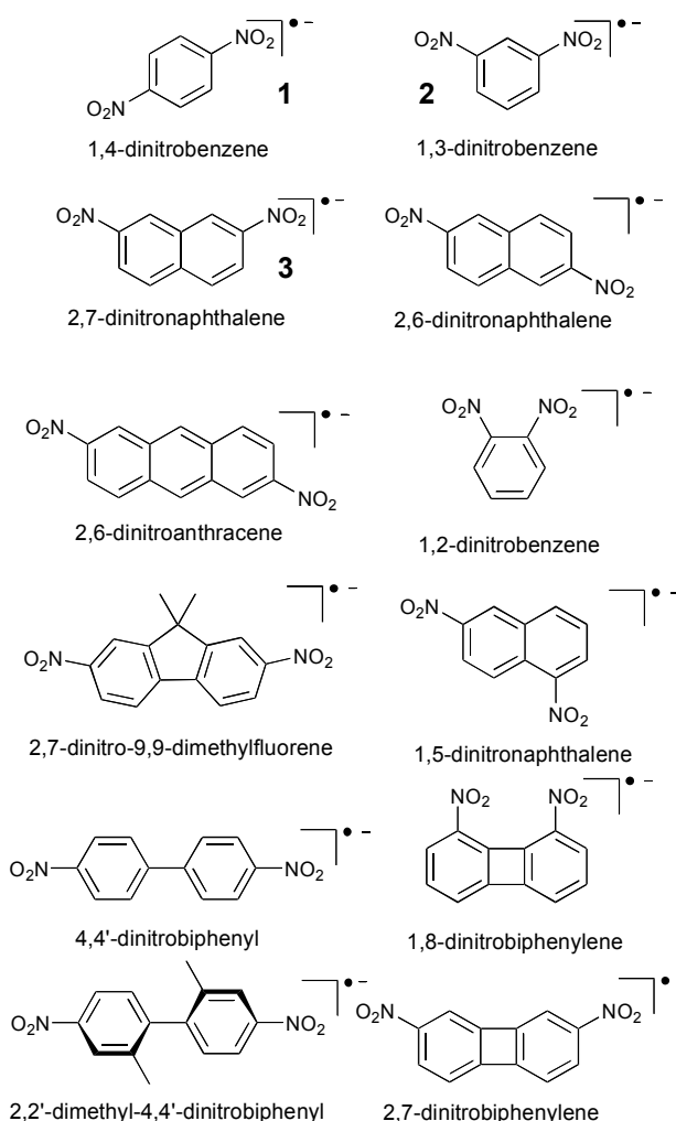
Figure 2. Dinitro radical anions investigated in refs. 3, 151.
