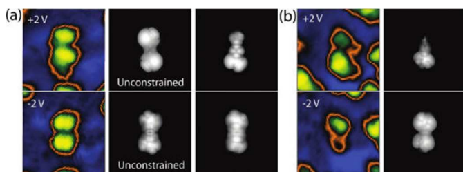
Figure 7. Comparison of simulated and experimental STM images under opposite biases for 12 (a, left) and 15 (b, right). CDFT (B3LYP) was employed to obtain charge localisation. 100 Reprinted with permission from R. C. Quardokus, Y. Lu, N. A. Wasio, C. S. Lent, F. Justaud, C. Lapinte and S. A. Kandel, J. Am. Chem. Soc. , 2012, 134 , 1710. Copyright 2012 American Chemical Society.
