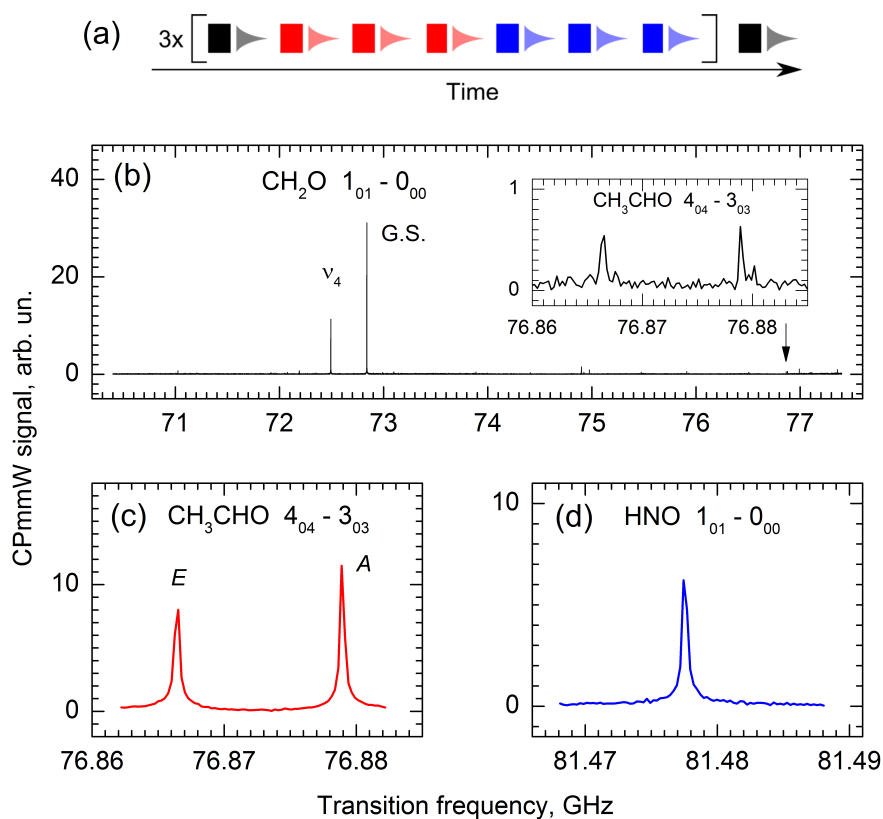
Figure 3. CPmmW spectroscopy of \text{CH}_3\text{CHO} , \text{H}_2\text{CO} , and \text{HNO} products of \text{CH}_3\text{CH}_3\text{ONO} pyrolysis using the multi-chirp approach. (a) Example of a multi-chirp sequence. In this sequence, a broadband 7 GHz chirp covering 70.4–77.4 GHz (black) is used in combination with 20 MHz chirps centered on relevant known transitions for \text{CH}_3\text{CHO} [60, 61] (red) and \text{HNO} [61, 62] (blue) to study pyrolysis of ethyl nitrite. (b-d) Spectra obtained from use of the chirp sequence in (a). Rotational J_{KaKc} assignments of the transitions are provided. (b) The broadband chirp, covering 70.4–77.4 GHz, provides an overview of the possible products and contains transitions of formaldehyde in the vibrational ground state (G.S.) and in the \nu_4 excited state. The insert magnifies the spectral region that contains two acetaldehyde transitions. (c) The narrowband chirp covering the 76.862–76.882 GHz region with the two acetaldehyde transitions that belong to the E and A symmetry ground states of the internal rotor excitation [60, 61]. (d) The narrowband chirp covering the 81.468 – 81.488 GHz region with the \text{HNO} transition [61, 62].
