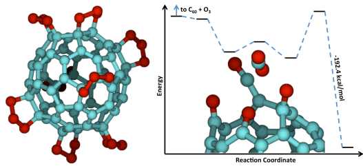
Reaction of ozone with C 60 leads to an opening of the fullerene cage
