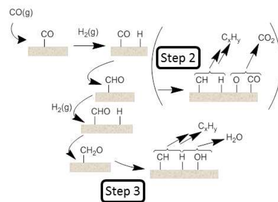
Figure 3. Reaction schemes for (1) carbide and (2) indirect mechanisms, via direct CO dissociation to form surface carbon (Step 1), or hydrogenation followed by subsequent dissociation (Step 2 or 3), respectively. Note: Schemes show only initial steps in the mechanism, the subsequent surface polymerisation to form C x H y species has been condensed for clarity. Also note the fate of oxygen as CO 2 or H 2 O has been given as argued by reference 31 based on the dominance of CO ads over H ads on the catalyst surface and the independence of CO 2 production from H 2 partial pressure.
