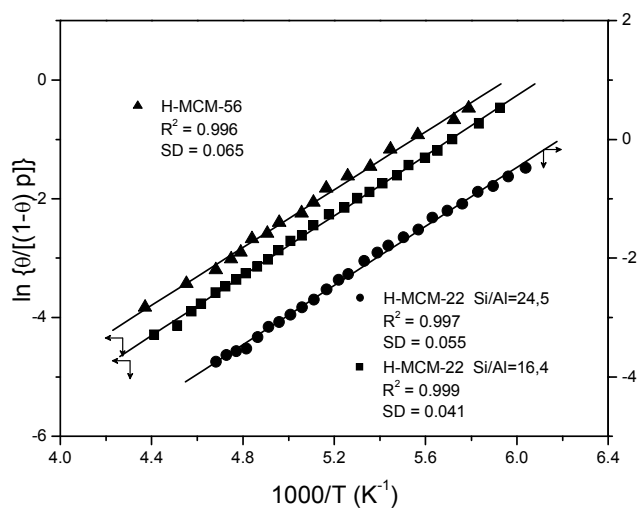
Figure 5. Plot of the left-hand side of eqn (5) against the reciprocal of the temperature for CO adsorbed on H-MCM-22 (Si:Al = 24.5:1 and 16.4:1) and H-MCM-56; data obtained from the O–H stretching bands. R, linear regression coefficient; SD, standard deviation.
