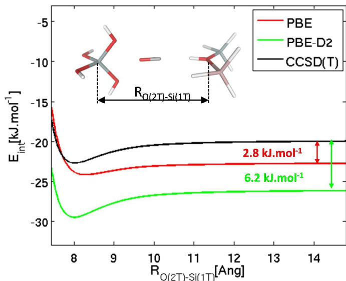
Figure 2. Interaction energy of CO with the Brønsted-acid site (represented by the 2T cluster model) and the model of zeolite framework (represented by 1T cluster model) calculated at CCSD(T), PBE, PBE-D2 levels, as a function of R_{O(2T)-Si(1T)} distance. Framework Si, Al, O, and H atom depicted in grey, pink, red, and white colours, respectively, CO atoms depicted in red and grey (O and C atom, respectively).
