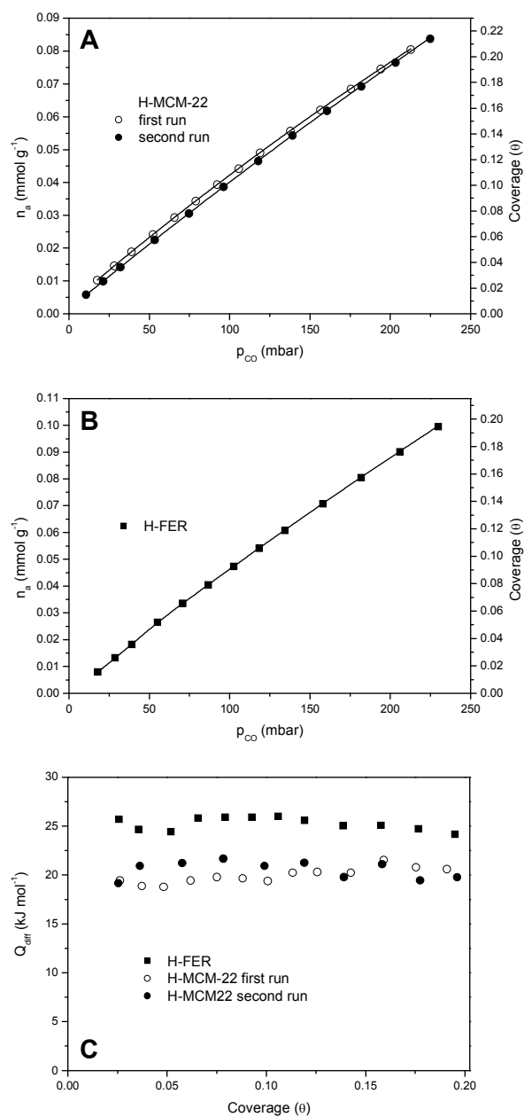
Figure 7. (A) Adsorption isotherm of CO on H-MCM-22 (Si:Al = 24.5:1) at 303 K; (B) adsorption isotherm of CO on H-FER zeolite (Si:Al = 27.5:1) at 303 K; (C) adsorption heat of CO on H-FER (squares) and H-MCM-22 (circles) measured by calorimetry at 303 K, as a function of coverage.
