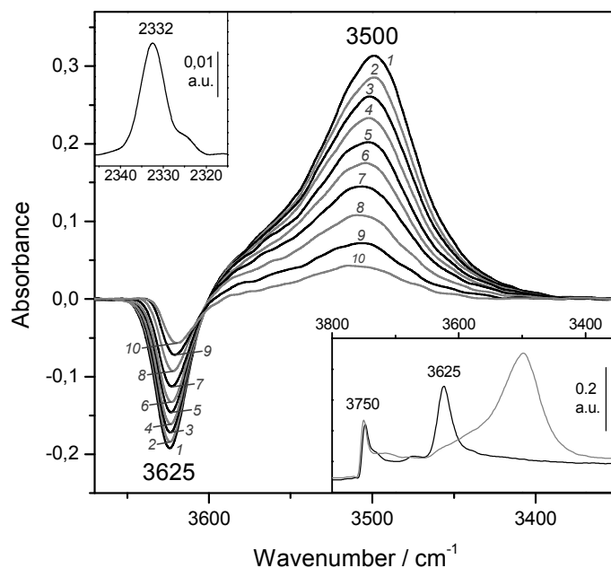
Figure 10. Representative variable-temperature IR spectra (O–H stretching region) of N 2 adsorbed on H-MCM-22 (Si:Al = 16.4:1). The spectra are shown in the difference mode (zeolite blank subtracted). Temperature (in K) and equilibrium pressure (mbar, in brackets) as follows: 1, 117 (4.43); 2, 125 (5.48); 3, 131 (6.27); 4, 137 (6.98); 5, 143 (7.68); 6, 149 (8.22); 7, 155 (8.73); 8, 163 (9.27); 9, 171 (9.70); 10, 179 (10.03). Bottom inset shows the blank zeolite spectrum (black) and the effect of dosing with CO at 77 K (grey). Top inset shows the N–N stretching region of spectrum 1.
