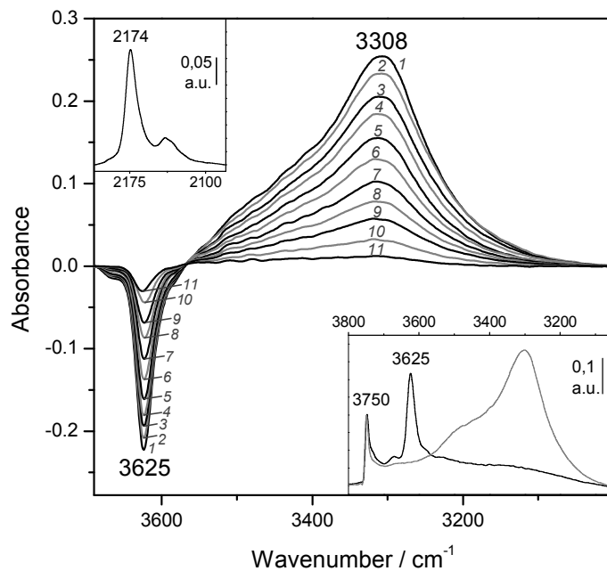
Figure 8. Representative variable-temperature IR spectra (O-H stretching region) of CO adsorbed on H-MCM-22 (Si:Al = 16.4:1). The spectra are shown in the difference mode (zeolite blank subtracted). Temperature (in K) and equilibrium pressure (mbar, in brackets) as follows: 1, 165 (15.13); 2, 171 (15.72); 3, 177 (16.13); 4, 181 (16.41); 5, 187 (16.78); 6, 193 (17.13); 7, 200 (17.47); 8, 206 (17.74); 9, 212 (18.01); 10, 222 (18.35); 11, 235 (18.69). Bottom inset shows the blank zeolite spectrum (black) and the effect of dosing with CO at 77 K (grey). Top inset shows the C-O stretching region of spectrum 1.
