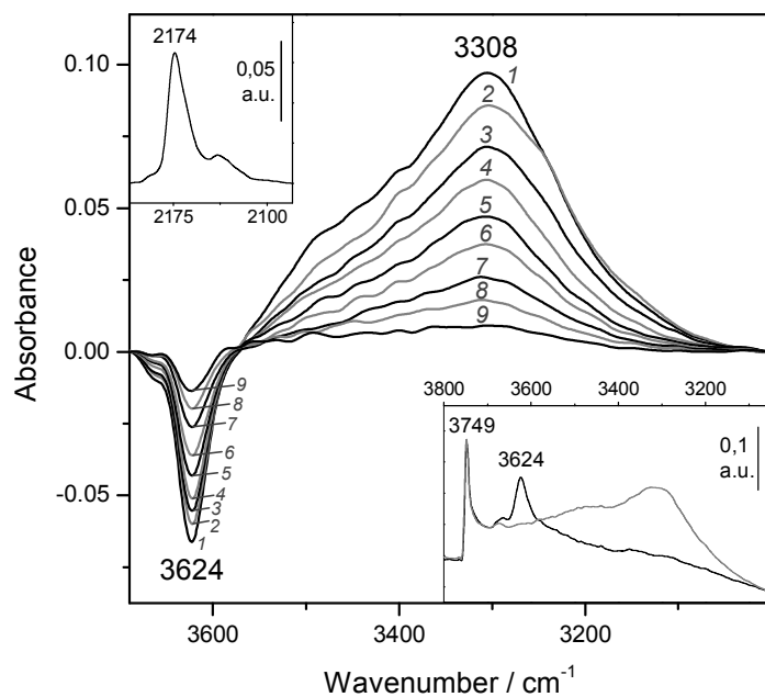
Figure 9. Representative variable-temperature IR spectra (O–H stretching region) of CO adsorbed on H-MCM-56. The spectra are shown in the difference mode (zeolite blank subtracted). Temperature (in K) and equilibrium pressure (mbar, in brackets) as follows: 1, 165 (10.33); 2, 175 (10.81); 3, 180 (11.01); 4, 184 (11.15); 5, 190 (11.37); 6, 196 (11.54); 7, 204 (11.74); 8, 211 (11.89); 9, 220 (12.07). Bottom inset shows the blank zeolite spectrum (black) and the effect of dosing with CO at 77 K (grey). Top inset shows the C–O stretching region of spectrum 1.
