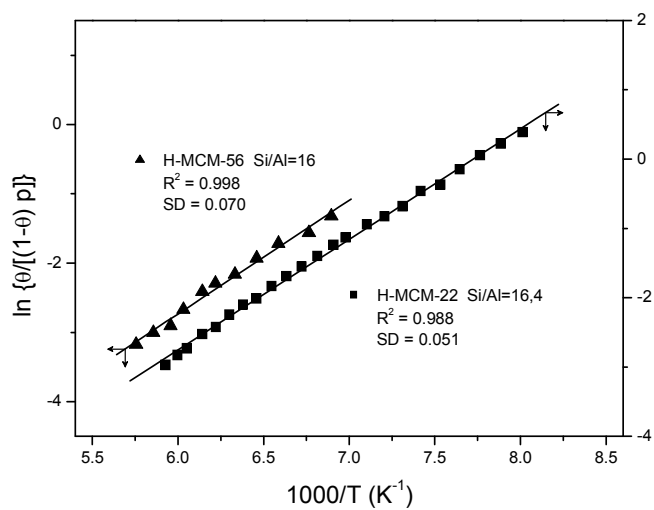
Figure 11. Plot of the left-hand side of eqn (5) against the reciprocal of the temperature for \text{N}_2 adsorbed on H-MCM-22 (Si:Al = 16.4:1) and H-MCM-56; data obtained from the corresponding O–H stretching bands. R, linear regression coefficient; SD, standard deviation.
