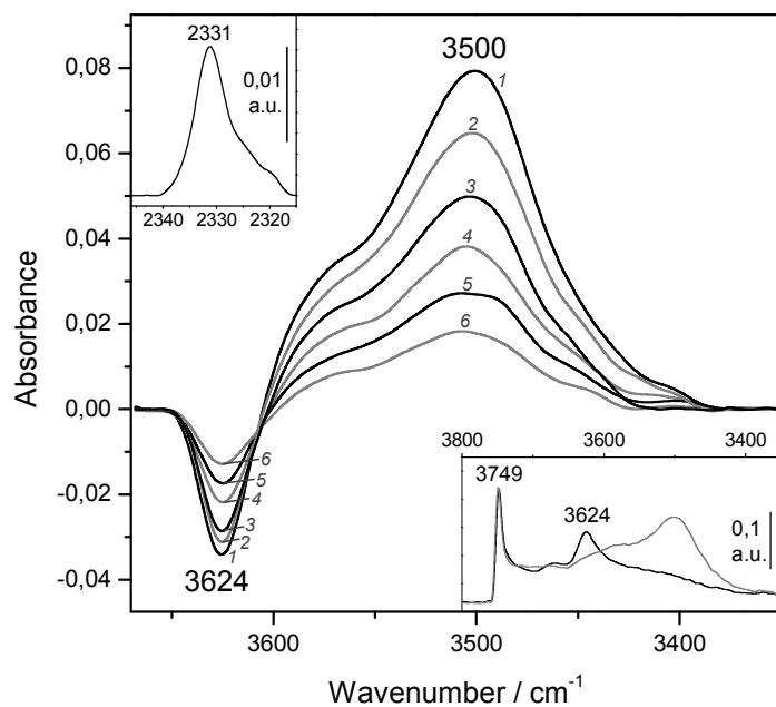
Figure 12. Representative variable-temperature IR spectra (O–H stretching region) of N 2 adsorbed on H-MCM-56. The spectra are shown in the difference mode (zeolite blank subtracted). From 1 to 6, temperature goes from 145 to 174 K; and equilibrium pressure from 9.55 to 10.95 mbar. Bottom inset shows the blank zeolite spectrum (black) and the effect of dosing with CO at 77 K (grey). Top inset shows the N–N stretching region of spectrum 1.
