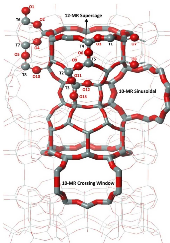
Figure 1. Structure of the MCM-22 framework and numbering scheme of the eight non-equivalent T sites and thirteen non-equivalent framework oxygen atoms. Framework T sites and framework oxygen atoms are depicted in grey and red, respectively.
