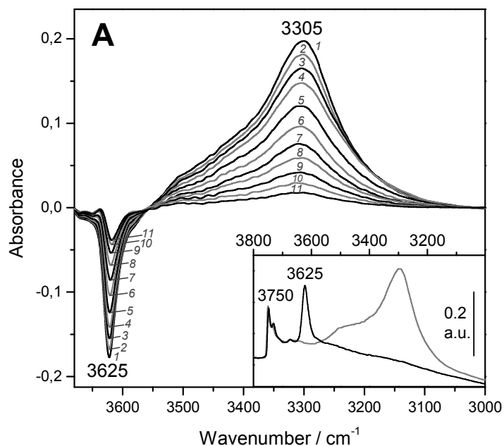
Figure 4A. Representative variable-temperature IR spectra (O-H stretching region) of CO adsorbed on H-MCM-22 (Si:Al = 24.5:1). The spectra are shown in the difference mode (zeolite blank subtracted). Temperature (in K) and equilibrium pressure (mbar, in brackets) as follows: 1, 154 (6.52); 2, 160 (6.99); 3, 166 (7.37); 4, 172 (7.72); 5, 178 (8.01); 6, 184 (8.29); 7, 190 (8.55); 8, 196 (8.75); 9, 202 (8.93); 10, 208 (9.11); 11, 214 (9.24). Inset shows the blank zeolite spectrum (black) and the effect of dosing with CO at 77 K (grey).
