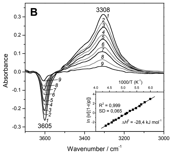
Figure 4B. Representative variable-temperature IR spectra (O–H stretching region) of CO adsorbed on H-FER (Si:Al = 27.5:1). The spectra are shown in the difference mode (zeolite blank subtracted). From 1 to 9, temperature goes from 167 to 224 K; and equilibrium pressure from 0.57 to 1.75 mbar. Inset shows the corresponding van't Hoff plot (Ref. 52).
