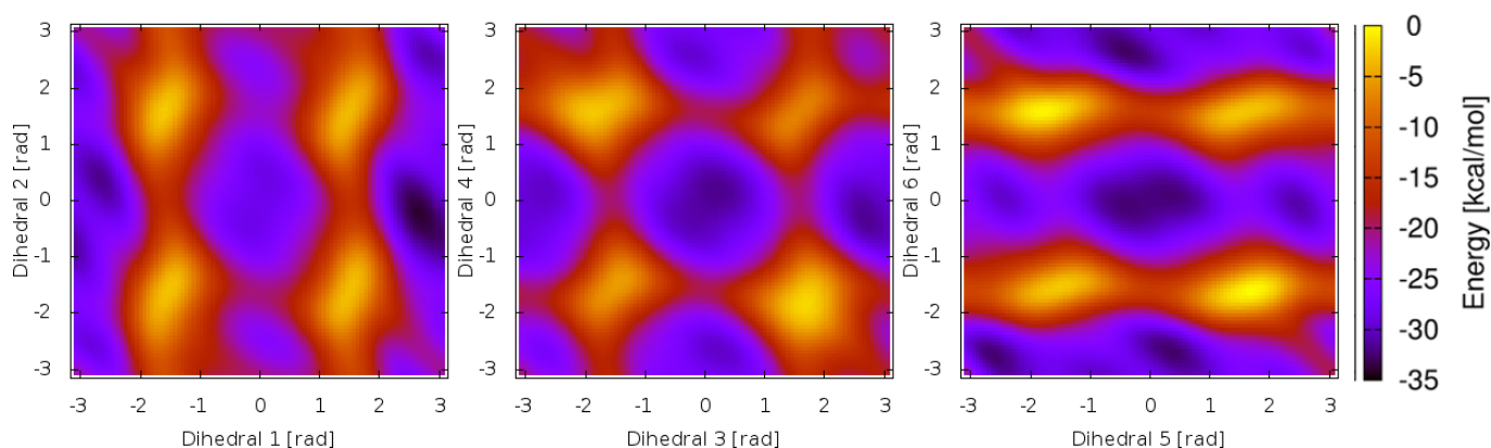
Fig. 2 Energy surface for the three dihedral pairs (1,2) to (5,6) connecting the pyrrol rings A to D. Twofold degenerate minima are visible for planar conformations, while the overall depth of the minima and height of the energy barriers varies to a great extent.
