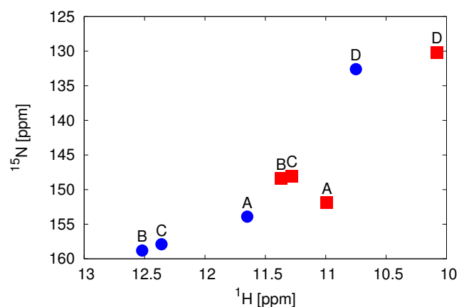
Fig. 5 Experimental 2D ^1\text{H} and ^{15}\text{N} NMR spectra different solvents: HMPT 22 (blue dots) and methanol 57 (red squares) of the amine groups of rings A to D
