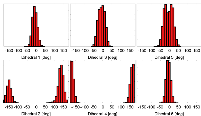
Fig. 3 Dihedral angle distributions during a molecular dynamics simulation. All dihedral angles remain stable on the simulation time of 75 ps. The different bond characteristics are clearly visible.
