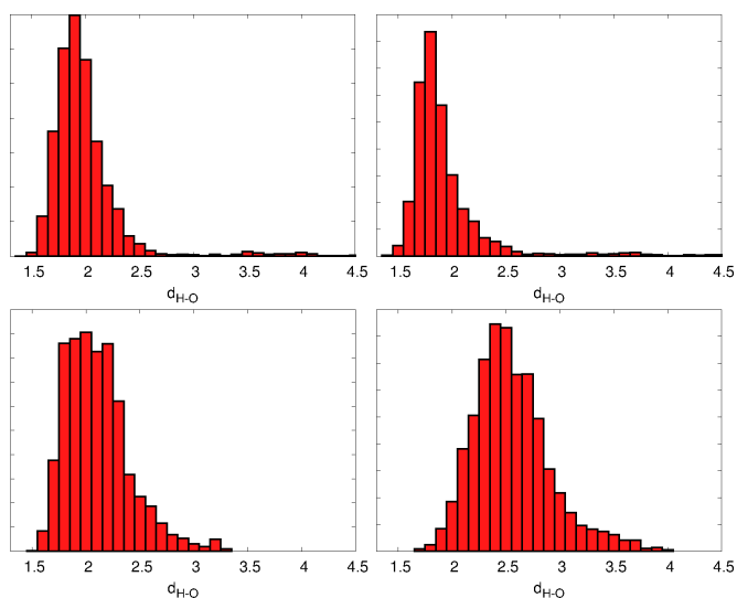
Fig. 4 Distribution of the four possible hydrogen bonds between the NH groups and the carboxylic groups lone oxygens, taken from a 10 ps BLYP-D trajectory of the ZEZsss conformation. Top left: ring A, right: ring B, bottom left: ring C, right: ring D
