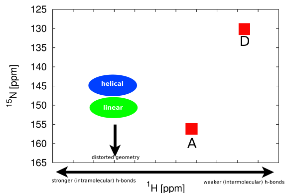
Fig. 6 Overview of the different influences on the ^1\text{H} and ^{15}\text{N} chemical shifts of PCB. A conformational change in the central dihedral pair of ring B and C causes a change in the positions of the signals of ring B and C as indicated by the green and blue areas. The remaining signals A and D remain stable. Changes in hydrogen bonding strength mainly causes the hydrogen chemical shifts to change.
