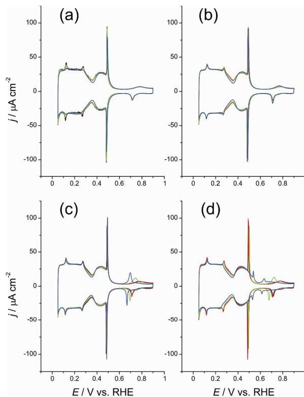
Figure 2. Cyclic Voltammograms, at 50 mV s -1 , of Pt(111) in 0.1 M H 2 SO 4 + x M MClO 4 . M = Li + (a), Na + (b), K + (c) and Cs + (d). x = 10 -4 (black), 10 -3 (red), 10 -2 (green) and 5 × 10 -2 (blue).
