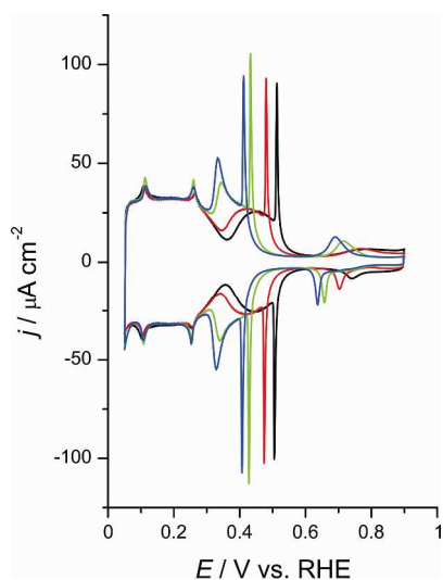
Figure 1. Cyclic Voltammograms, at 50 mV s -1 , of Pt(111) in 0.05 (black), 0.1 (red), 0.5 (green), and 1 M (blue) H 2 SO 4 .
