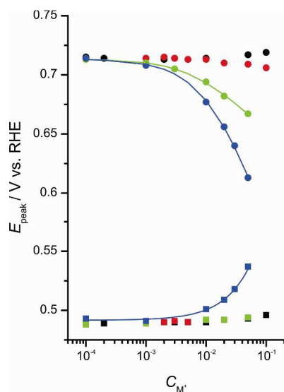
Figure 3. Semilogarithmic plots of the dependence of the spike potential in the positive sweep (squares), and of the hump potential in the negative sweep (circles) in the CV at 50 mV s -1 of Pt(111) in 0.1 M H 2 SO 4 on the concentration of alkali-metal cations (black: Li + ; red: Na + ; green: K + ; blue: Cs + ). The lines are fits of the experimental data to Equations (7) and (8), respectively.
